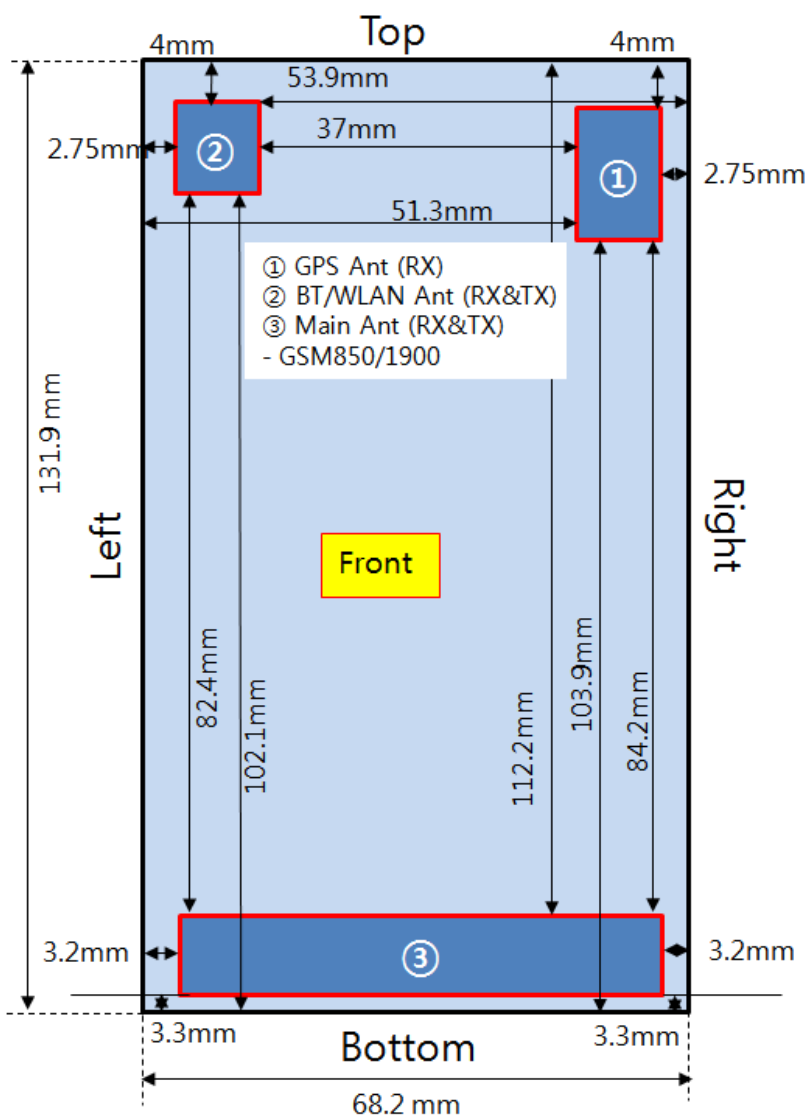
Figure 12.1 Identification of Sides for SAR Testing (Front Side View)
