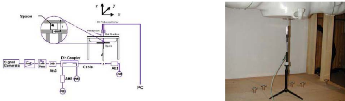
Figure 9.1 Dipole Validation Test Setup
