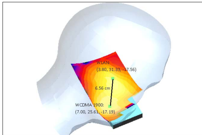
Figure 16-3 WCDMA 1900 and WLAN in Left Touch
