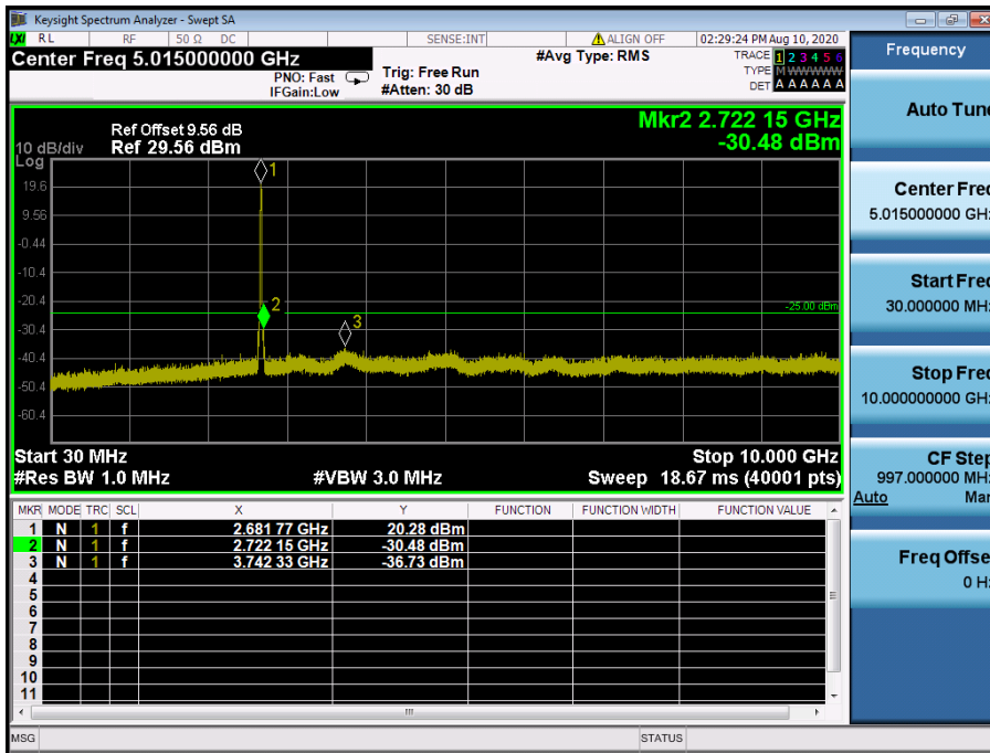
LTE Band 41 / 15 MHz / QPSK - RB Size/Offset (75/0) – High Channel
