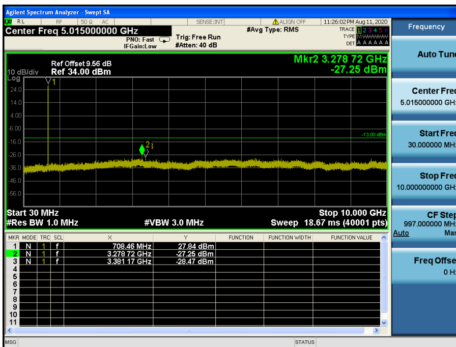
LTE Band 12 / 5 MHz / 64QAM - RB Size/Offset (12/13) – Mid Channel
