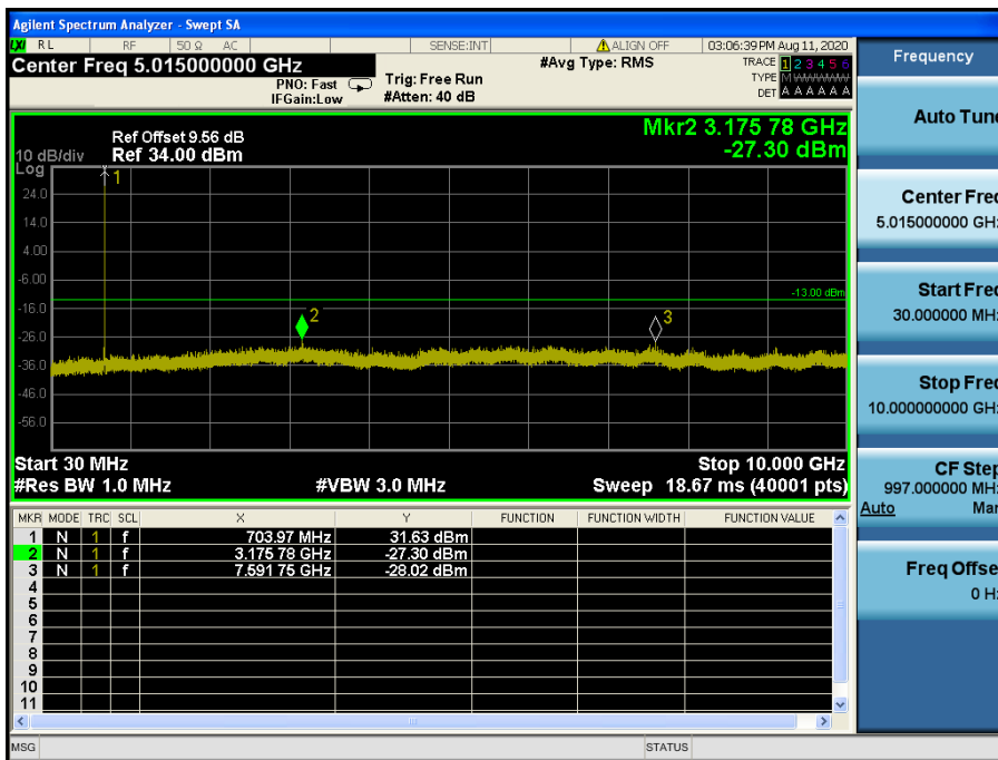
LTE Band 12 / 5 MHz / QPSK - RB Size/Offset (1/24) – Low Channel
