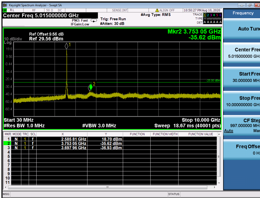
LTE Band 41 / 20 MHz / 64QAM - RB Size/Offset (100/0) – Mid Channel
