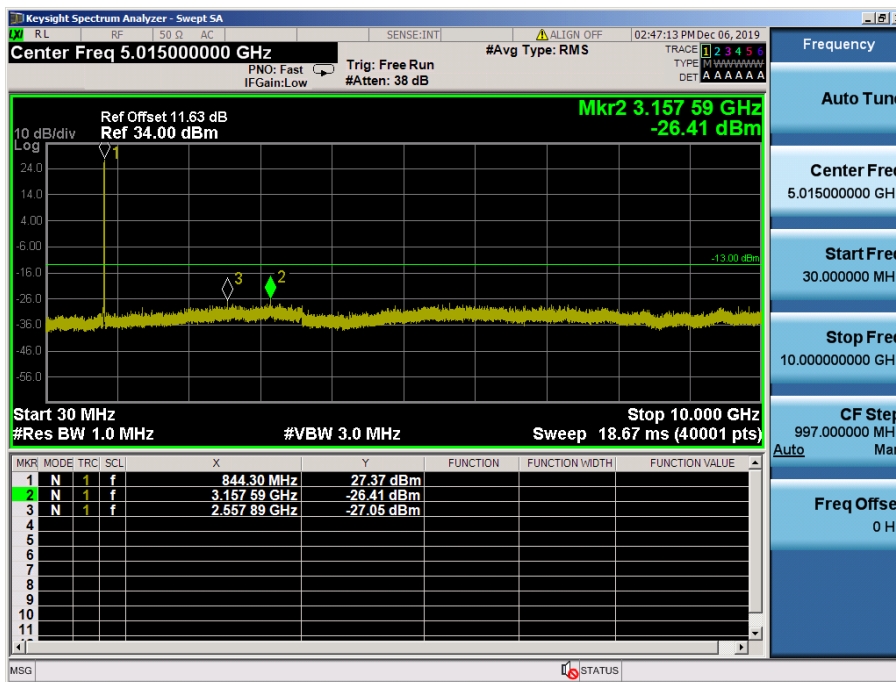
LTE Band 5 / 10MHz / 16QAM - RB Size/Offset (25/12) – High Channel
