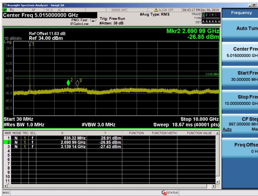
LTE Band 5 / 5MHz / 64QAM - RB Size/Offset (12/0) – Mid Channel
