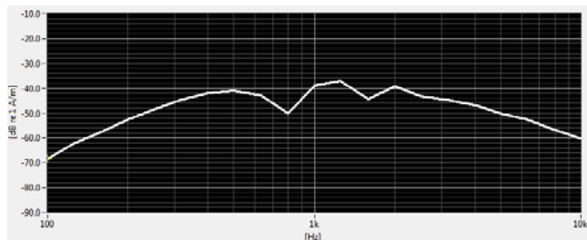
Figure 6-2 Worst-case ABM2 Plot for WD
