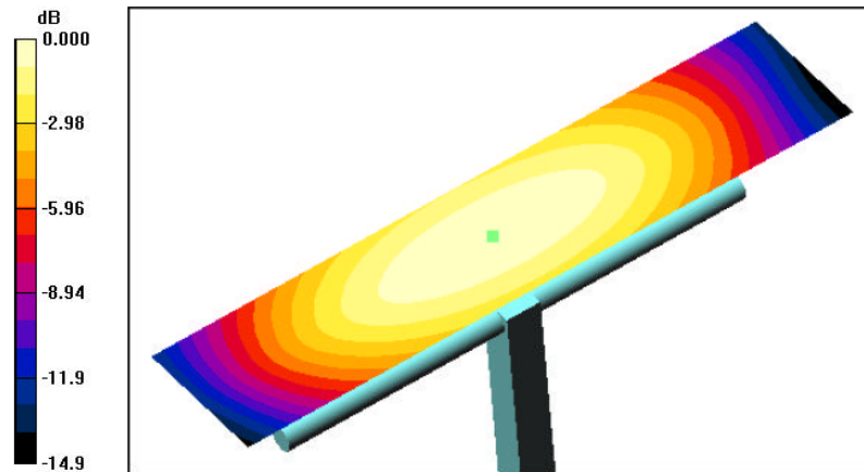
0 dB = 0.449A/m
