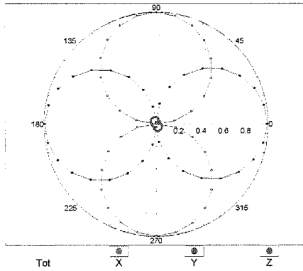
f=600 MHz,TEM,0°
