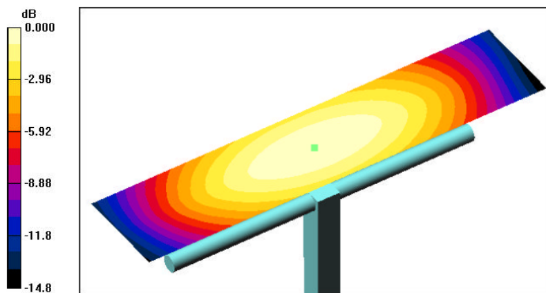
0 dB = 0.507 A/m
