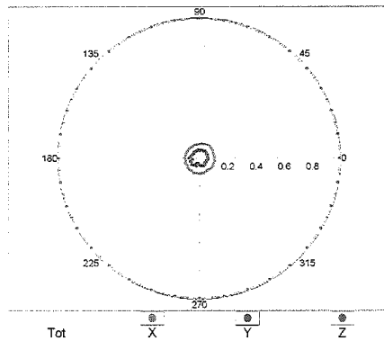
f=600 MHz,TEM,90°
