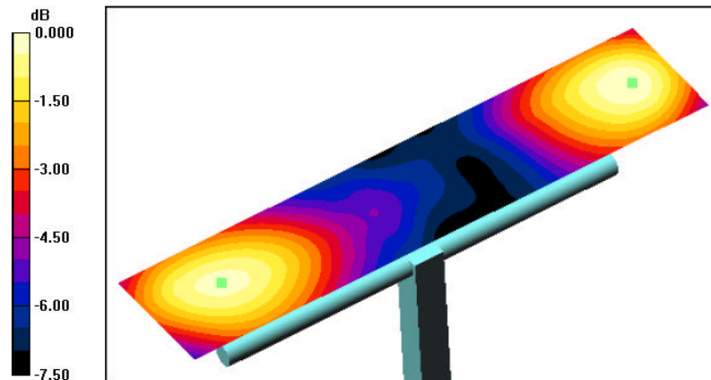
0 dB = 142.2V/m
