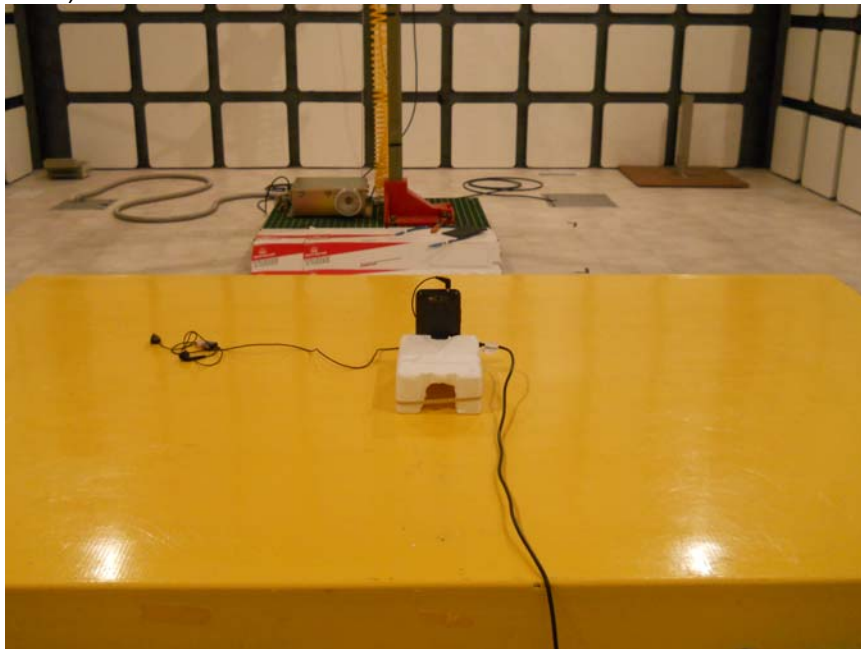
Y-AXIS with Ear Phone & AC Adapter_BACK PHOTO (worst-case)
