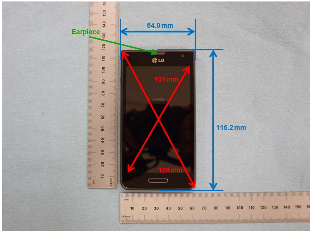
Overall Dimensions
