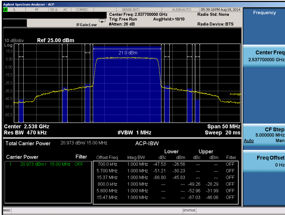
Plot 6-99. Mid ACP Plot (Band 7 – 15.0MHz QPSK – RB Size 75)
