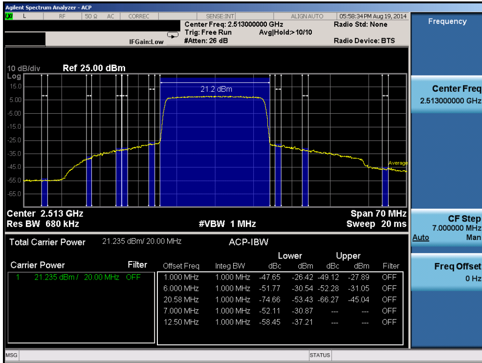
Plot 6-101. Lower ACP Plot (Band 7 – 20.0MHz QPSK – RB Size 100)
