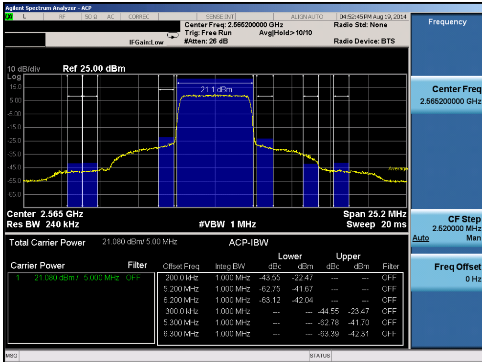
Plot 6-94. Upper ACP Plot (Band 7 – 5.0MHz QPSK – RB Size 25)
