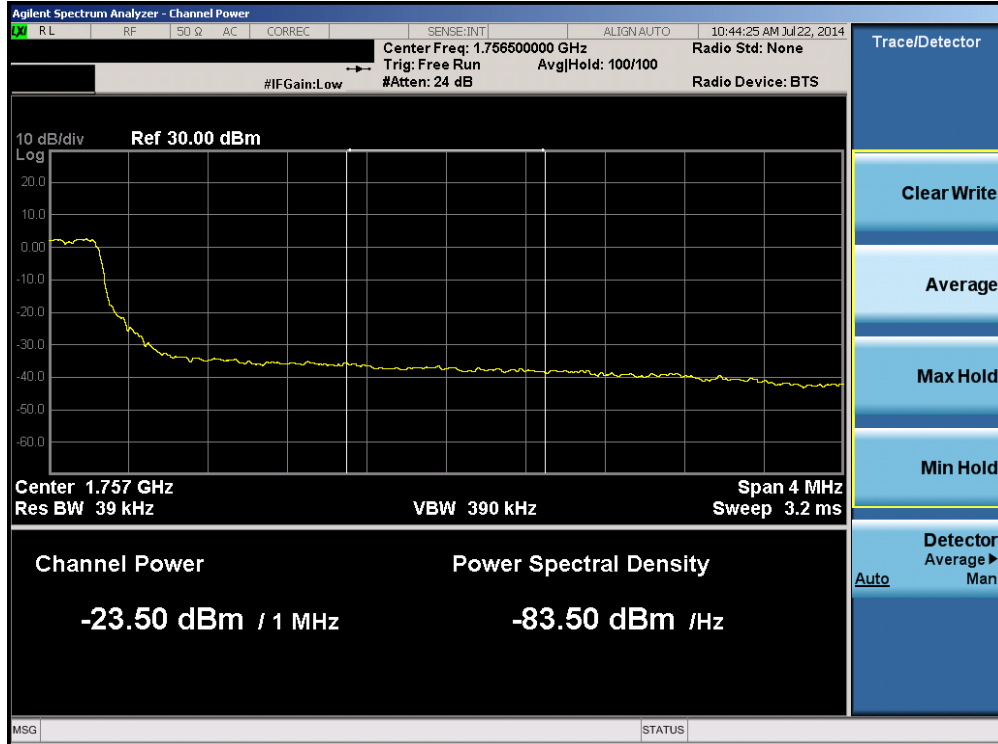
Plot 6-63. Upper Extended Band Edge Plot (Band 4 – 5.0MHz QPSK – RB Size 25)
