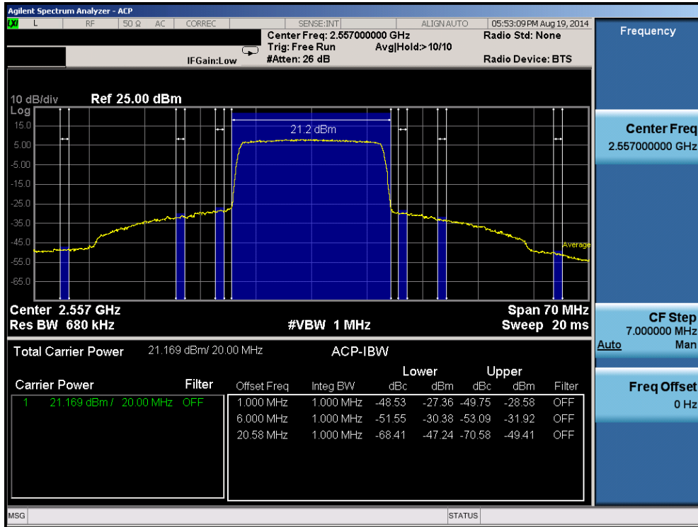
Plot 6-103. Upper ACP Plot (Band 7 – 20.0MHz QPSK – RB Size 100)
