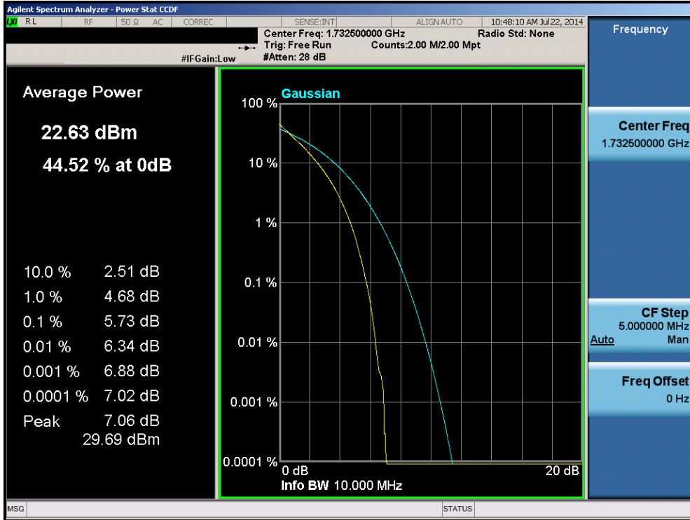
Plot 6-122. PAR Plot (Band 4 – 10.0MHz – QPSK – RB Size 50)
