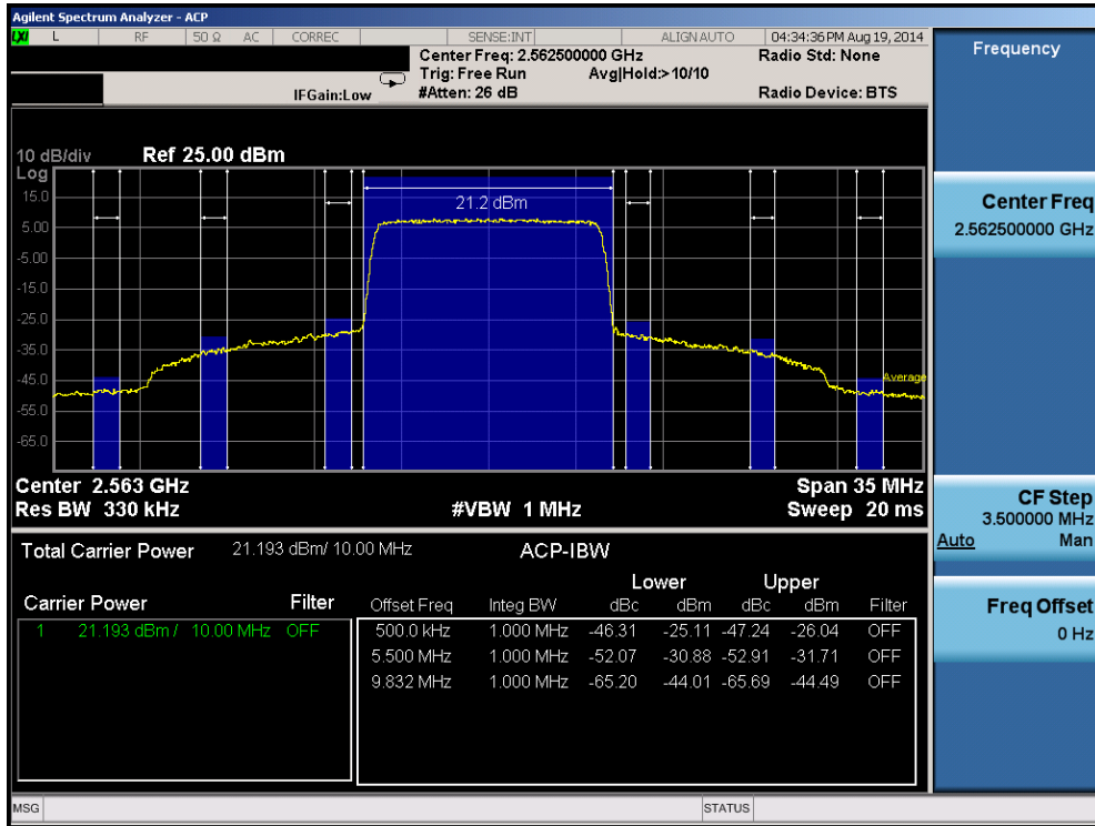
Plot 6-97. Upper ACP Plot (Band 7 – 10.0MHz QPSK – RB Size 50)
