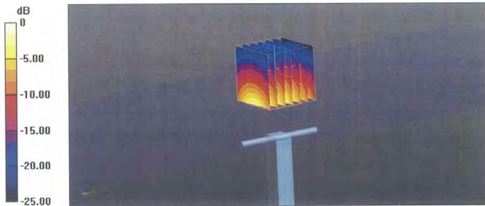
0 dB = 25.3 W/kg = 14.03 dBW/kg
