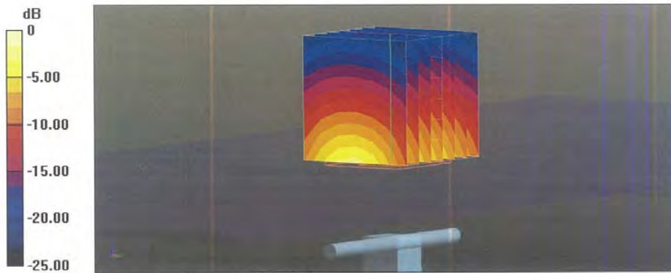
0 dB = 20.7 W/kg = 13.16 dBW/kg
