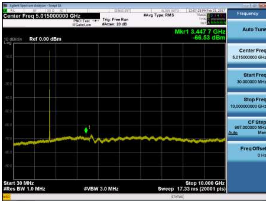
BAND 4. Conducted Spurious Plot_1 (20175ch_20MHz_QPSK_RB 1_0)
