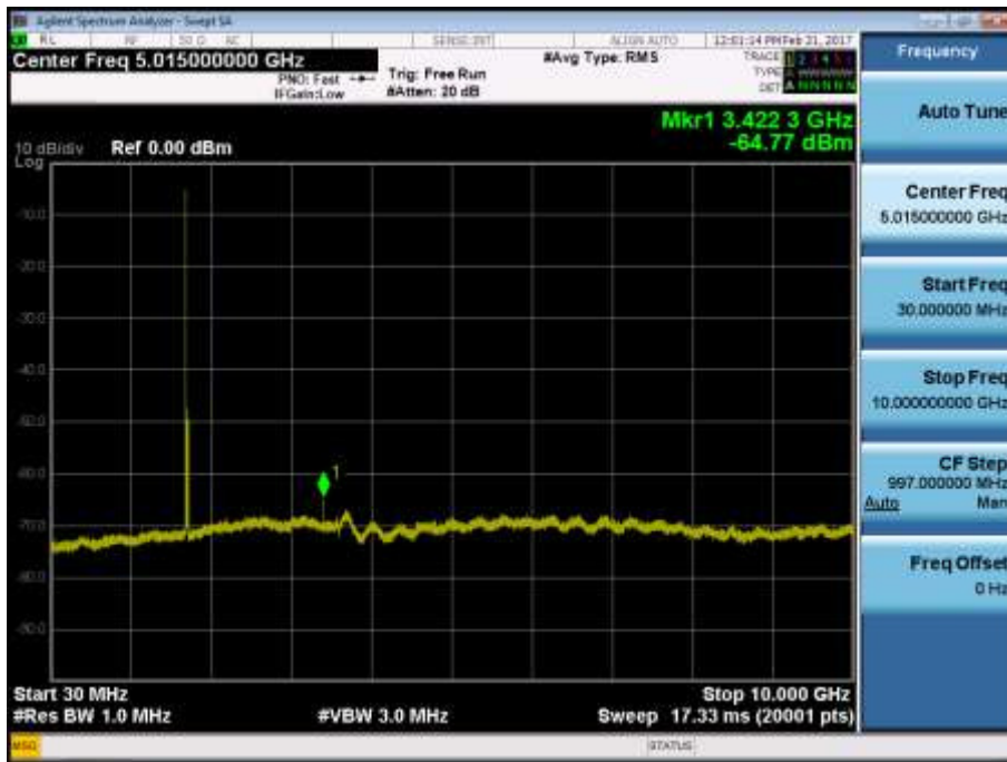
BAND 4. Conducted Spurious Plot_1 (20025ch_15MHz_QPSK_RB 1_0)
