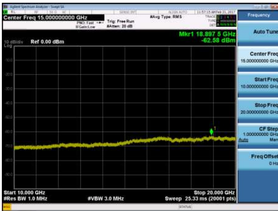
BAND 4. Conducted Spurious Plot_2 (20000ch_10MHz_QPSK_RB 1_0)
