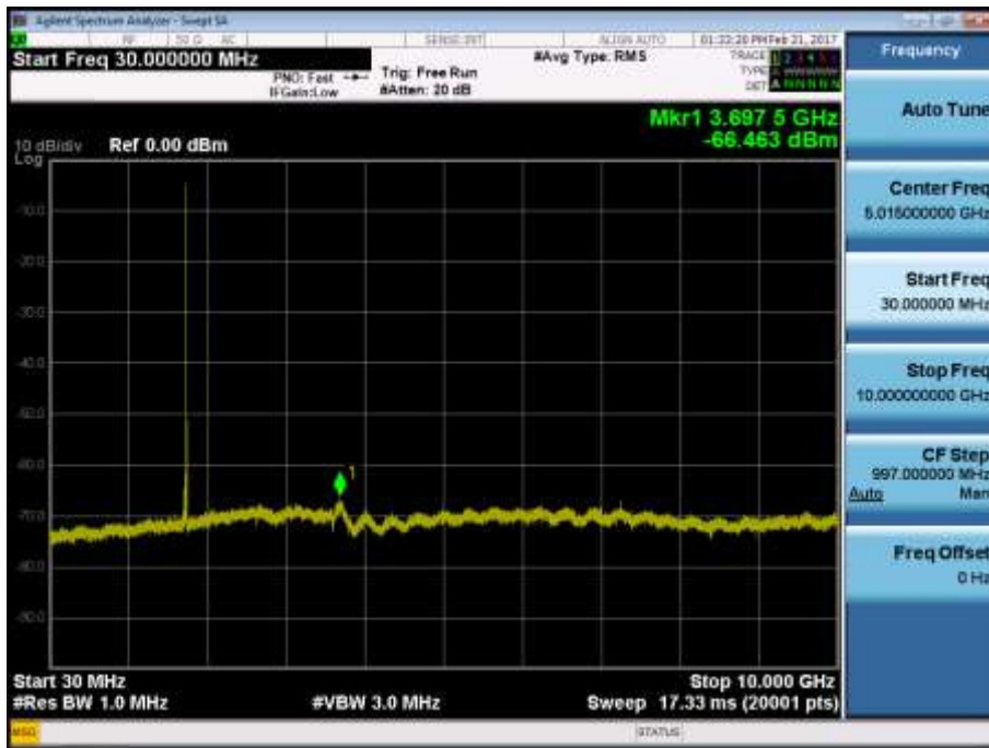
BAND 4. Conducted Spurious Plot_1 (20325ch_15MHz_QPSK_RB 1_0)
