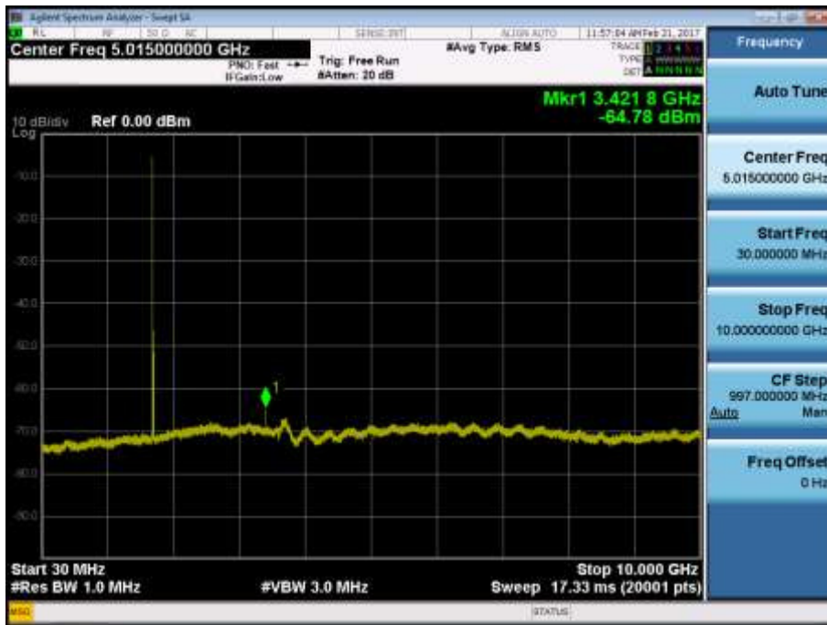
BAND 4. Conducted Spurious Plot_1 (20000ch_10MHz_QPSK_RB 1_0)
