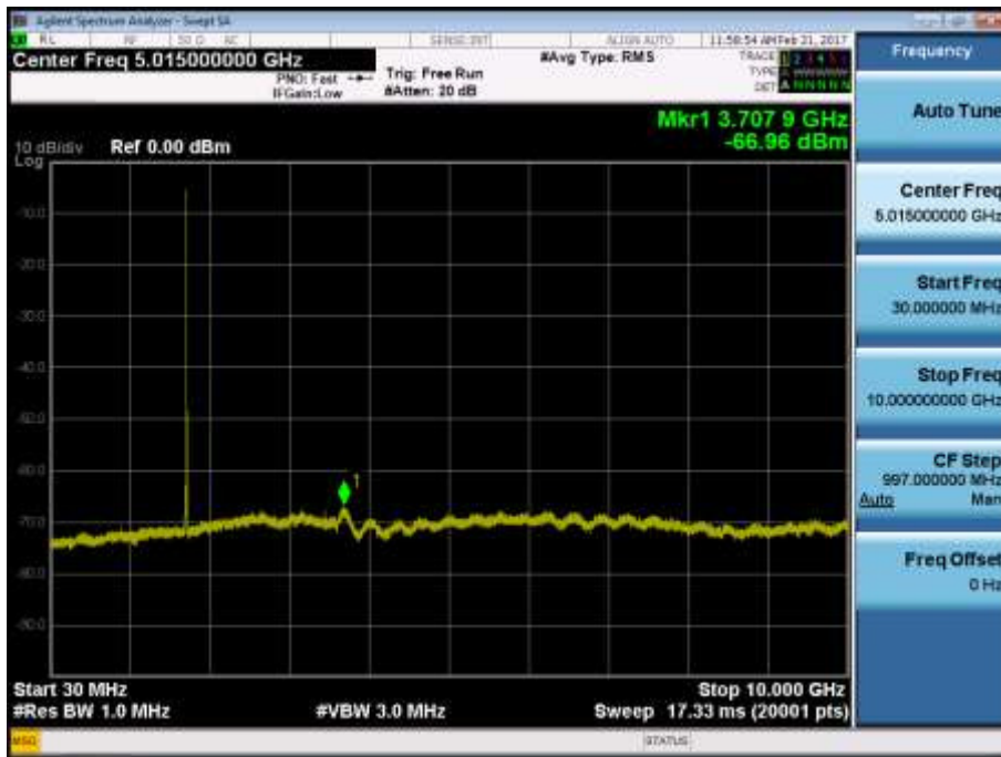
BAND 4. Conducted Spurious Plot_1 (20175ch_10MHz_QPSK_RB 1_0)
