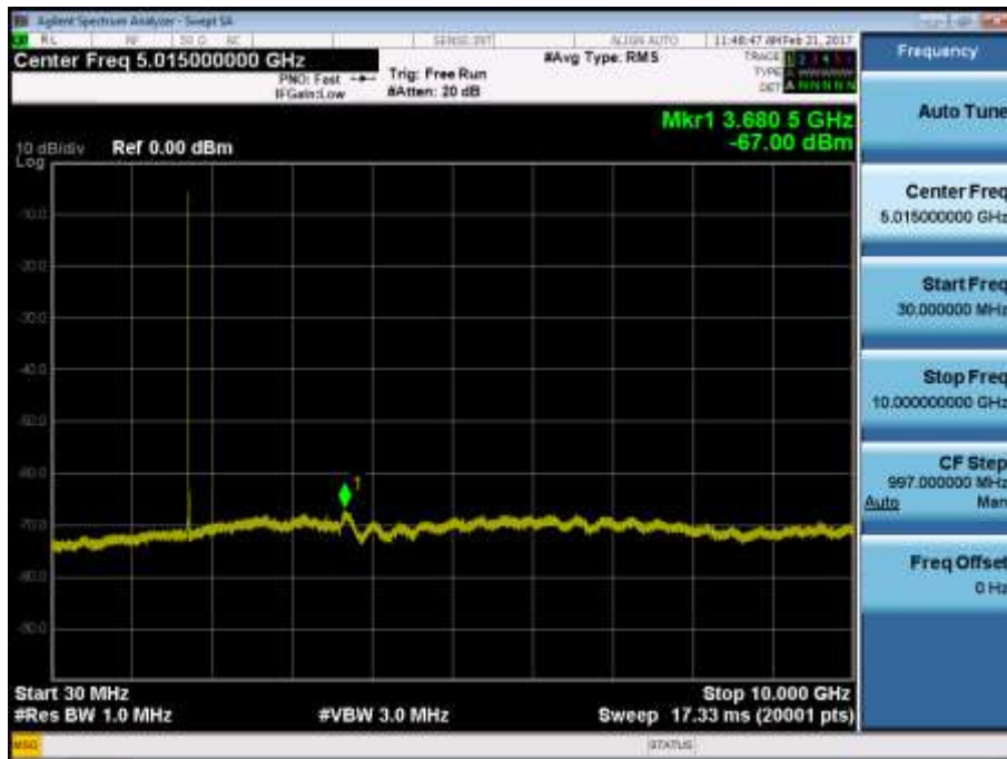
BAND 4. Conducted Spurious Plot_1 (20175ch_3MHz_QPSK_RB 1_0)
