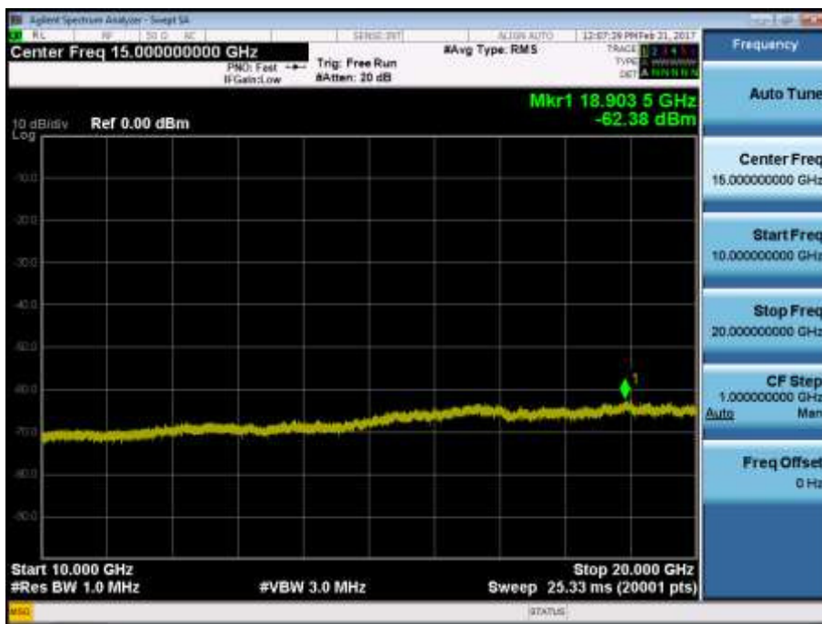
BAND 4. Conducted Spurious Plot_2 (20175ch_20MHz_QPSK_RB 1_0)
