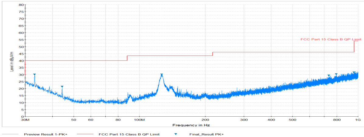
Plot 7-44. Radiated Spurious Plot below 1GHz (Pol. V)
