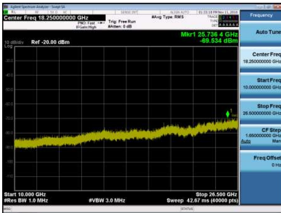
BAND7. Conducted Spurious Plot 2 (20MHz Ch.21100 QPSK RB 1, Offset 0)
