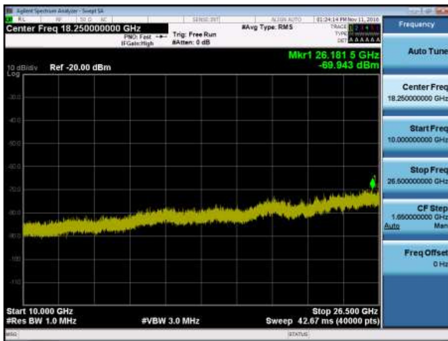
BAND7. Conducted Spurious Plot 2 (10MHz Ch.20800 QPSK RB 1, Offset 0)
