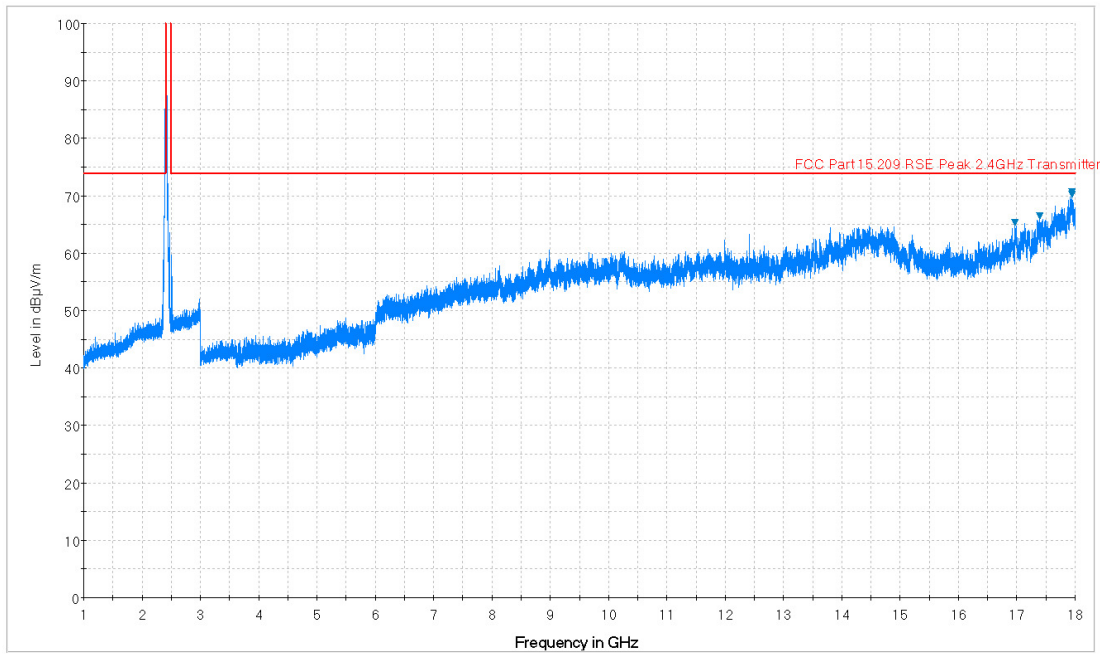
Plot 7-37. Radiated Spurious Plot above 1GHz (802.11b – Ch. 1, Ant. Pol. H)
