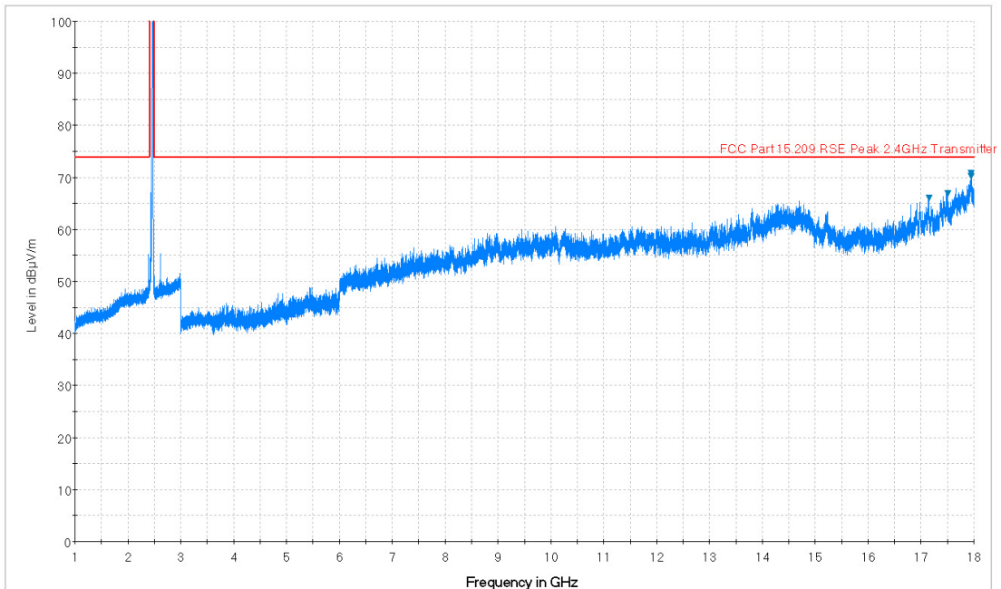
Plot 7-42. Radiated Spurious Plot above 1GHz (802.11b – Ch. 11, Ant. Pol. V)
