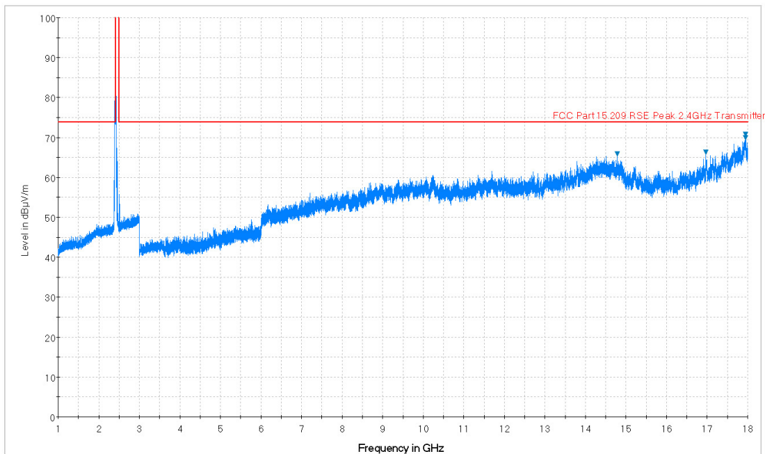
Plot 7-38. Radiated Spurious Plot above 1GHz (802.11b – Ch. 1, Ant. Pol. V)
