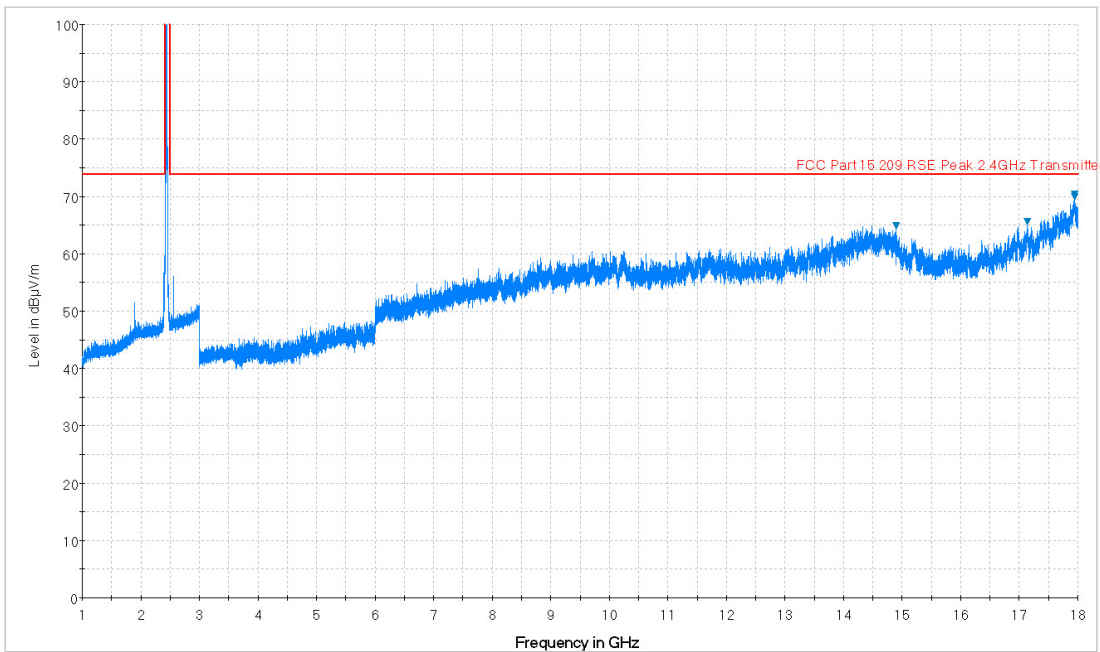
Plot 7-40. Radiated Spurious Plot above 1GHz (802.11b – Ch. 6, Ant. Pol. V)
