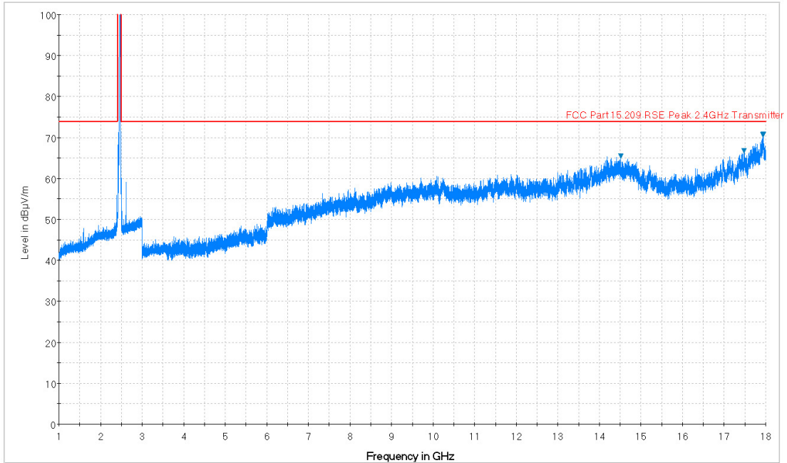
Plot 7-41. Radiated Spurious Plot above 1GHz (802.11b – Ch. 11, Ant. Pol. H)
