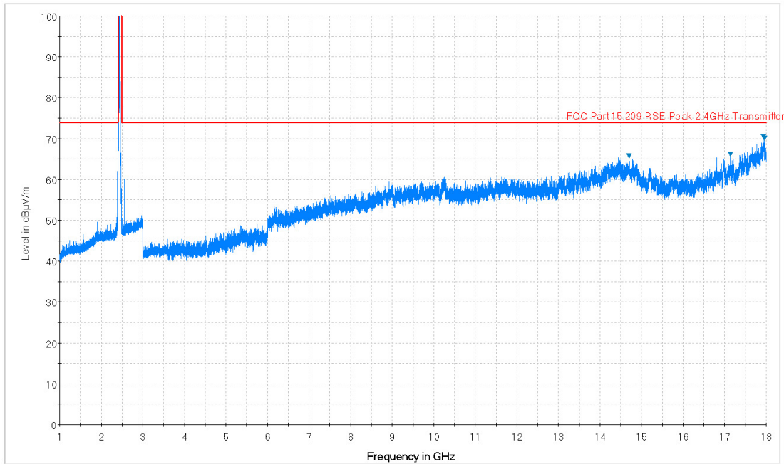
Plot 7-39. Radiated Spurious Plot above 1GHz (802.11b – Ch. 6, Ant. Pol. H)
