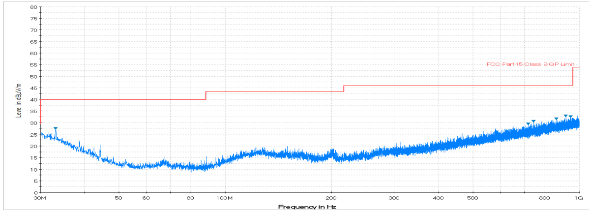
Plot 7-37. Radiated Spurious Plot below 1GHz (Pol. H)
