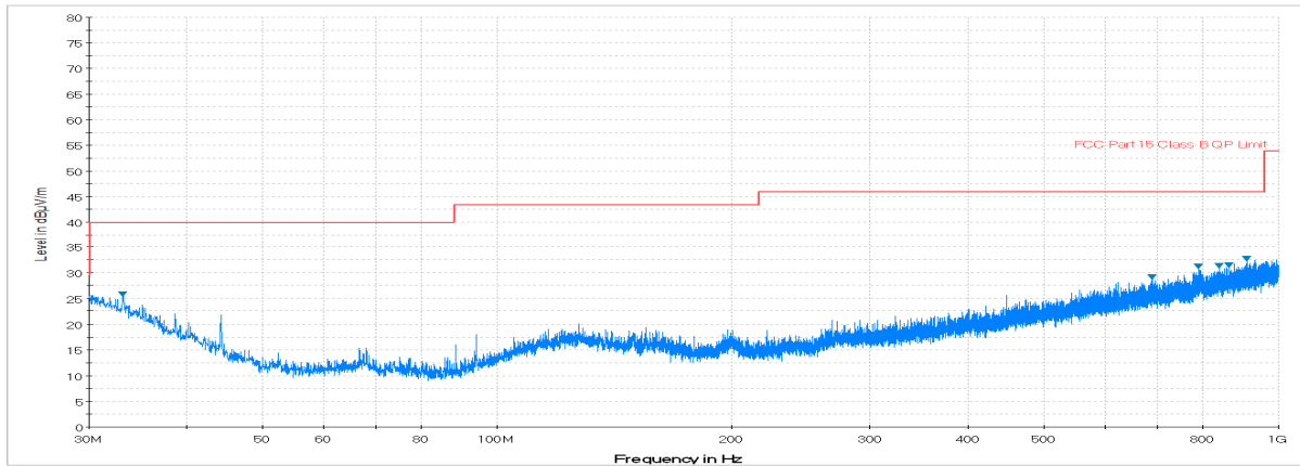
Plot 7-38. Radiated Spurious Plot below 1GHz (Pol. V)
