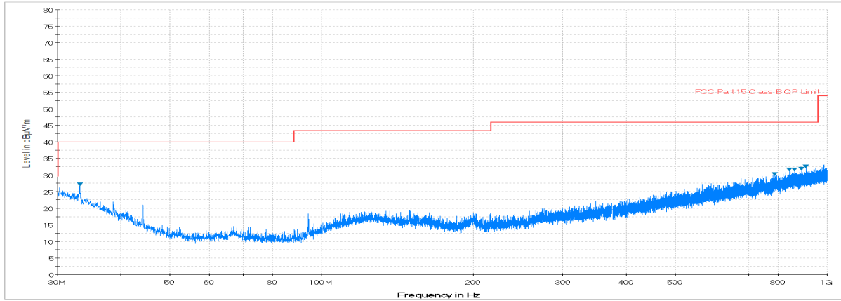
Plot 7-35. Radiated Spurious Plot below 1GHz (Pol. H)
