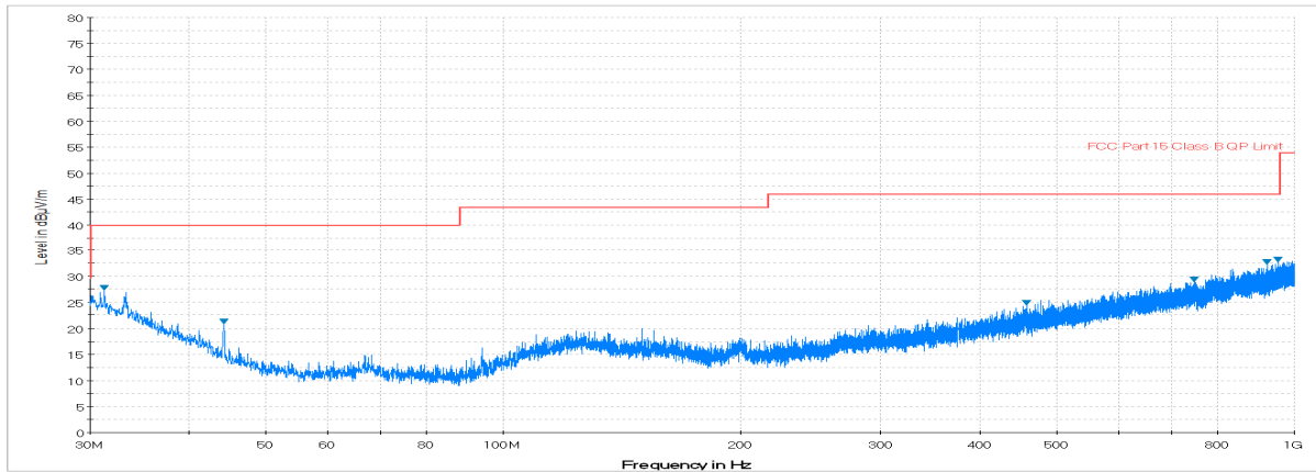
Plot 7-36. Radiated Spurious Plot below 1GHz (Pol. V)
