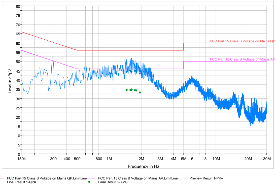
Plot 6-110. Line Conducted Plot with 802.11a UNII Band 4 (N)
