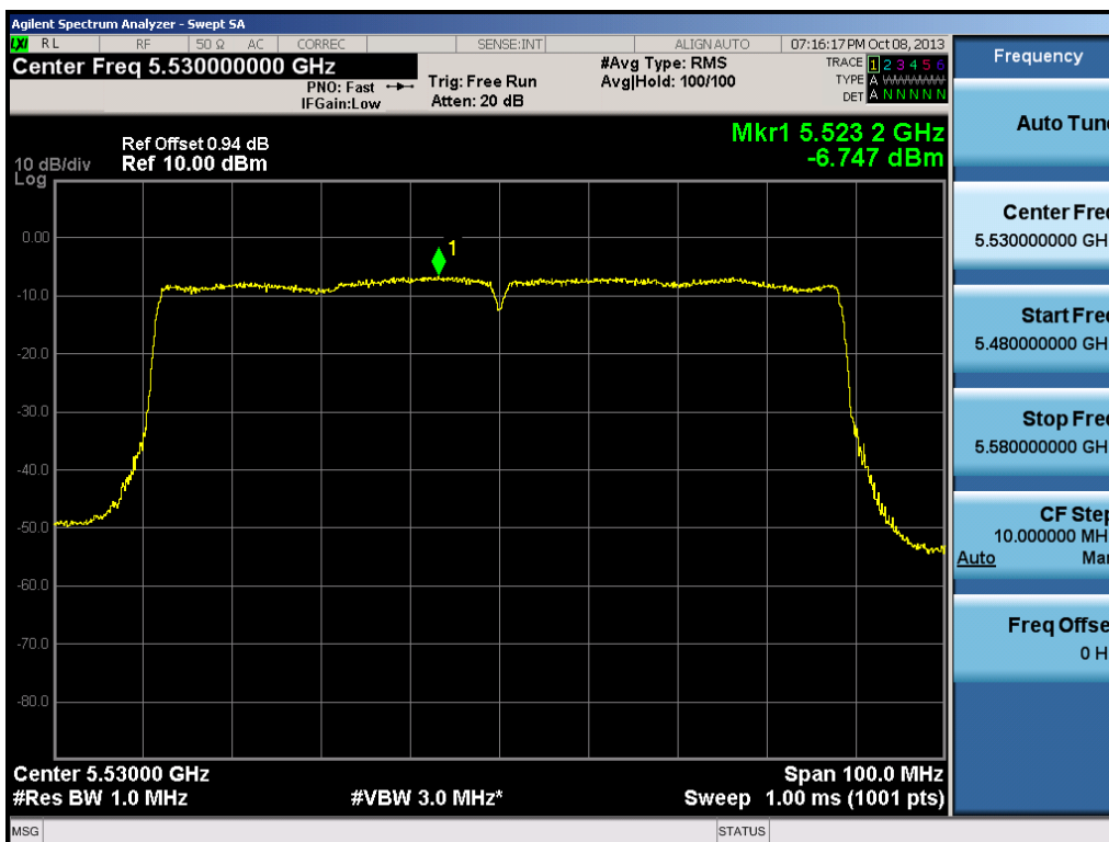
Plot 6-68. Peak Power Spectral Density Plot (80MHz BW 802.11ac (UNII Band 3) – Ch. 106)
