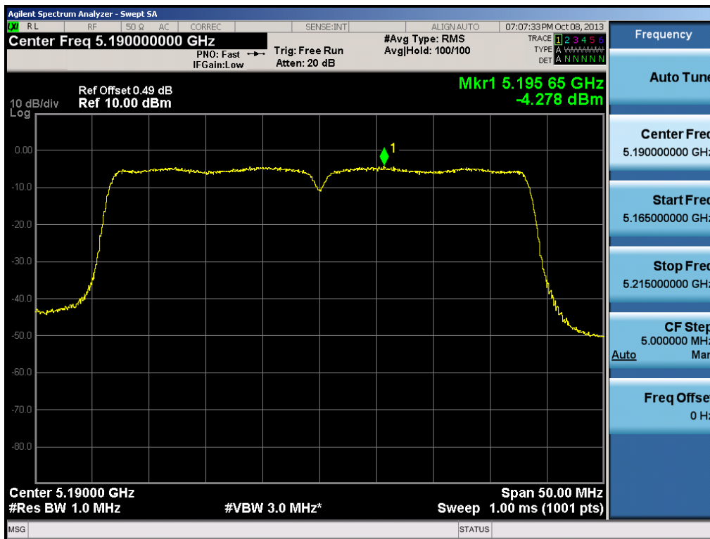
Plot 6-47. Peak Power Spectral Density Plot (40MHz BW 802.11n (UNII Band 1) – Ch. 38)
