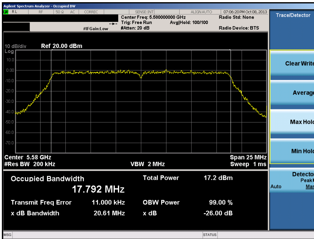
Plot 6-23. 26dB Bandwidth Plot (20MHz BW 802.11n (UNII Band 3) – Ch. 116)
