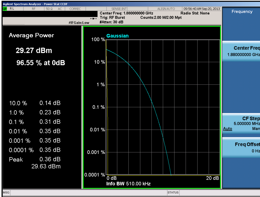
Plot 6-64. Peak-Average Ratio Plot (PCS GSM Mode – Ch. 661)
