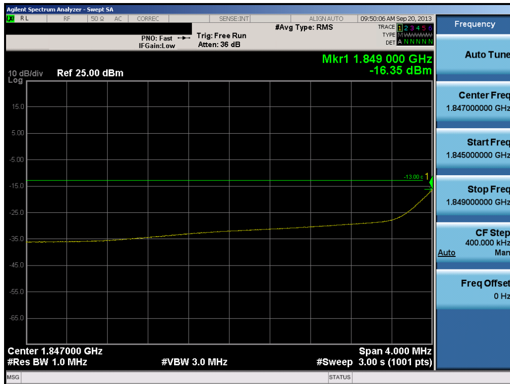
Plot 6-61. 4MHz Span Plot (PCS WCDMA Mode – Ch. 9262)
