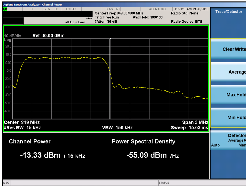
Plot 6-53. Band Edge Plot (Cellular CDMA Mode – Ch. 777)
