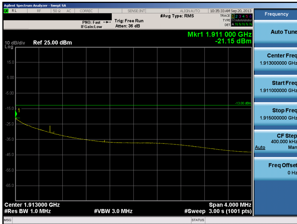
Plot 6-57. 4MHz Span Plot (PCS CDMA Mode – Ch. 1175)
