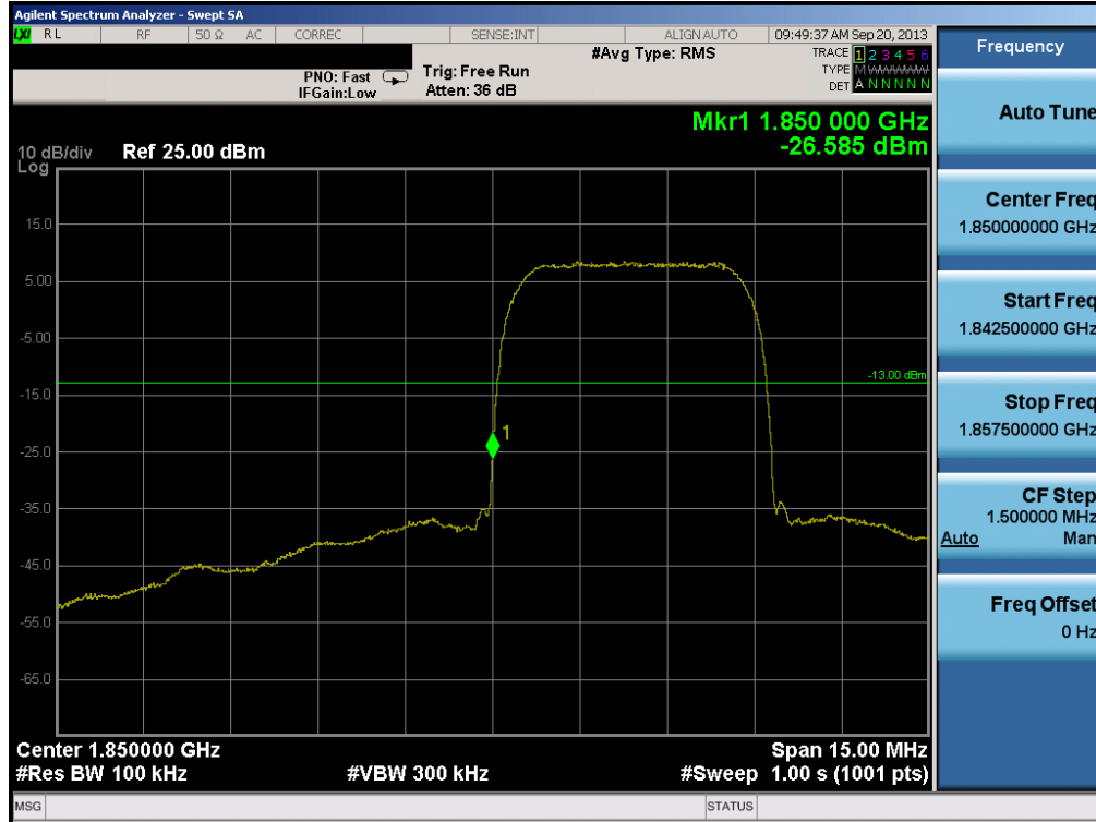
Plot 6-60. Band Edge Plot (PCS WCDMA Mode – Ch. 9262)
