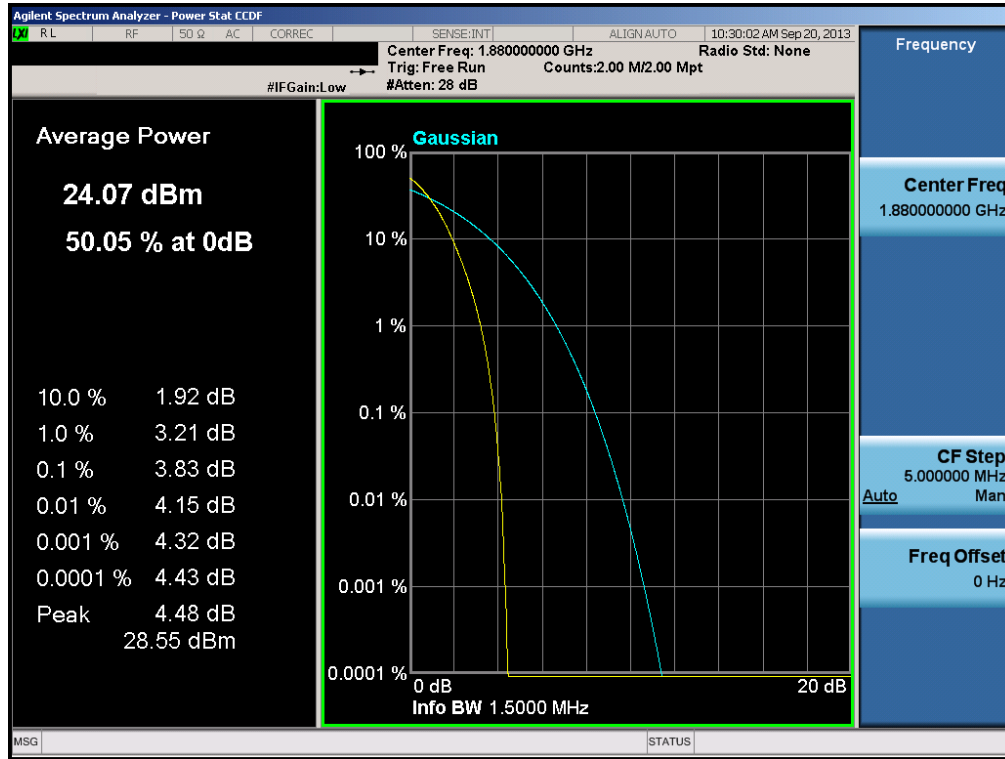
Plot 6-66. Peak-Average Ratio Plot (PCS CDMA Mode – Ch. 600)
