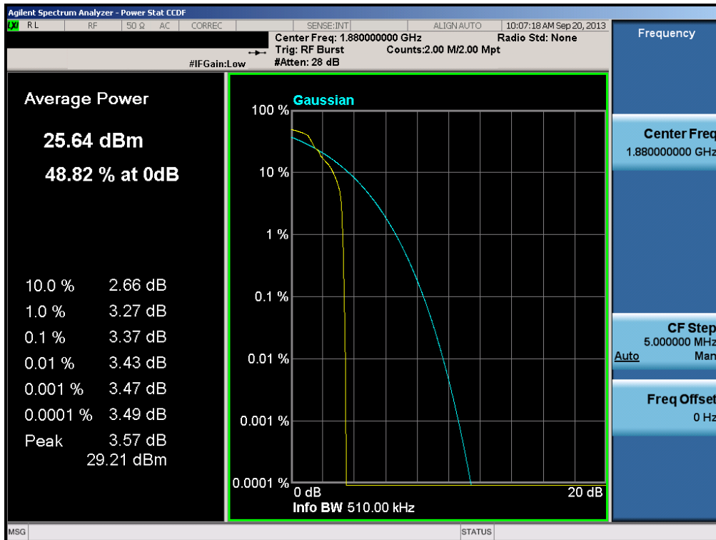
Plot 6-65. Peak-Average Ratio Plot (EDGE1900 Mode – Ch. 661)
