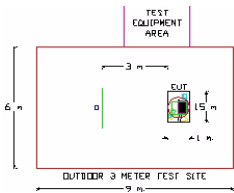
Figure 3-2. Dimensions of Outdoor Test Site
