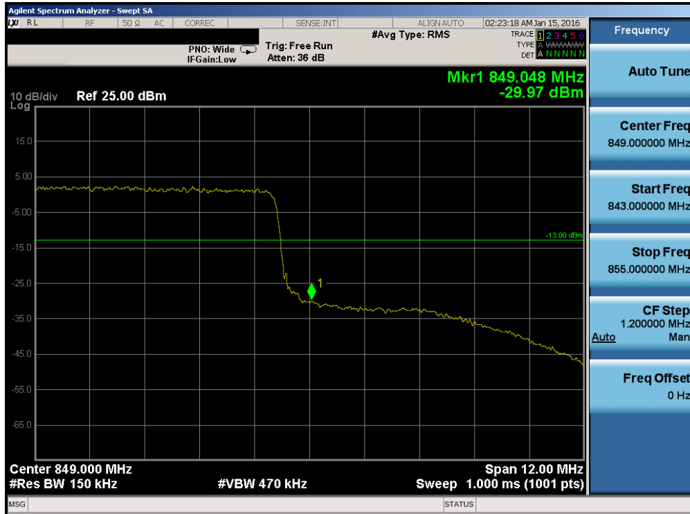
Plot 7-125. Upper Band Edge Plot (Band 26 – 15.0MHz QPSK – RB Size 75)
