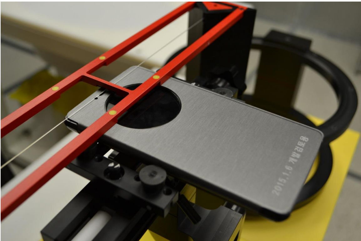
Front View of the DUT with Smart Cover
