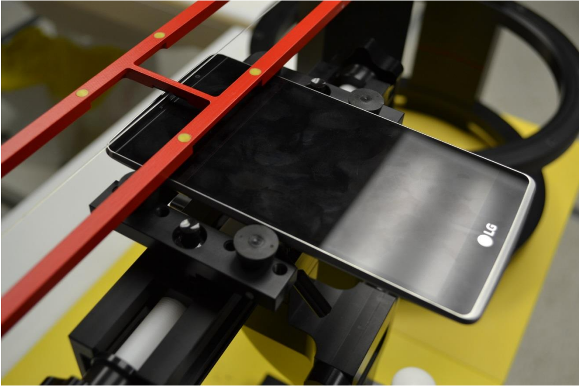
Front View of the DUT without Stylus
