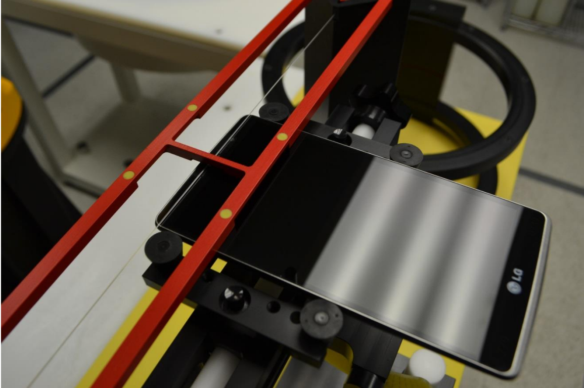
Setup Photo without Smart Cover
