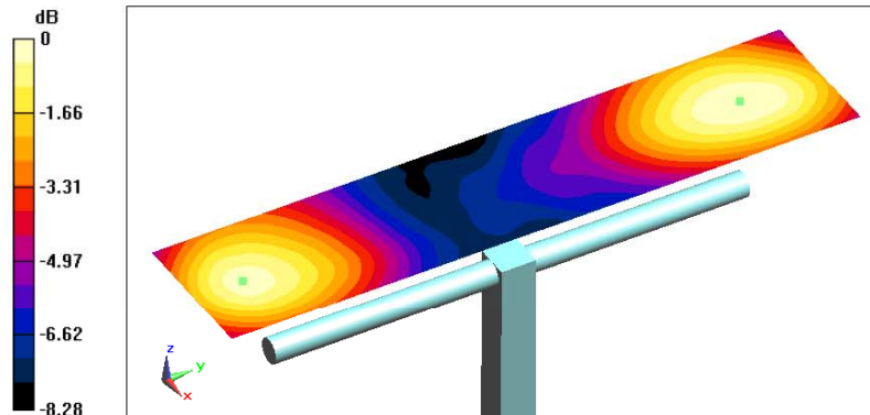
0 dB = 144.9V/m
