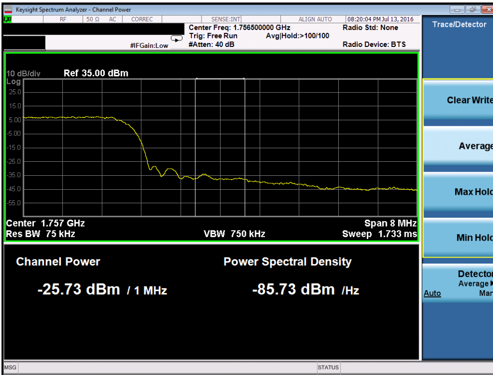
Plot 7-92. Band Edge Plot (AWS WCDMA Mode – Ch. 1513)
