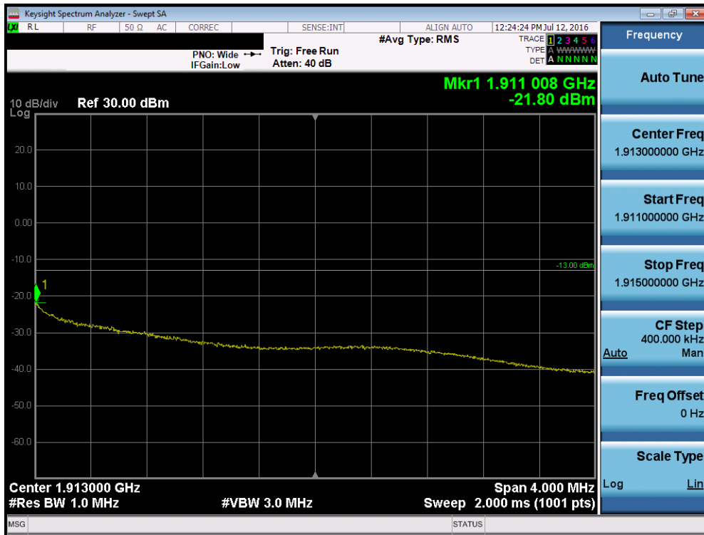
Plot 7-86. 4MHz Span Plot (PCS CDMA Mode – Ch. 1175)
