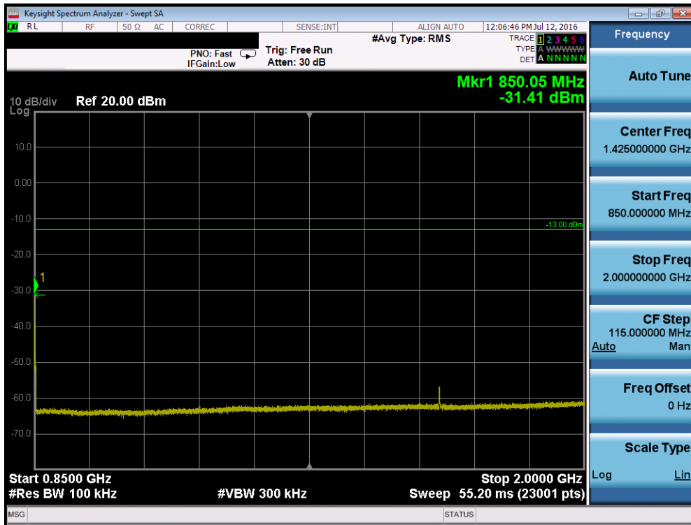
Plot 7-35. Conducted Spurious Plot (Cellular CDMA Mode – Ch. 777)
