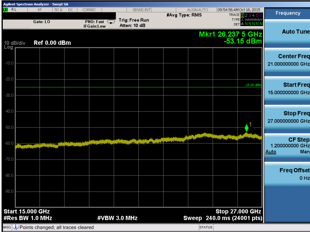
Plot 7-63. Conducted Spurious Plot (Band 41 – 10.0MHz QPSK – RB Size 1, RB Offset 0 – Mid Channel)
