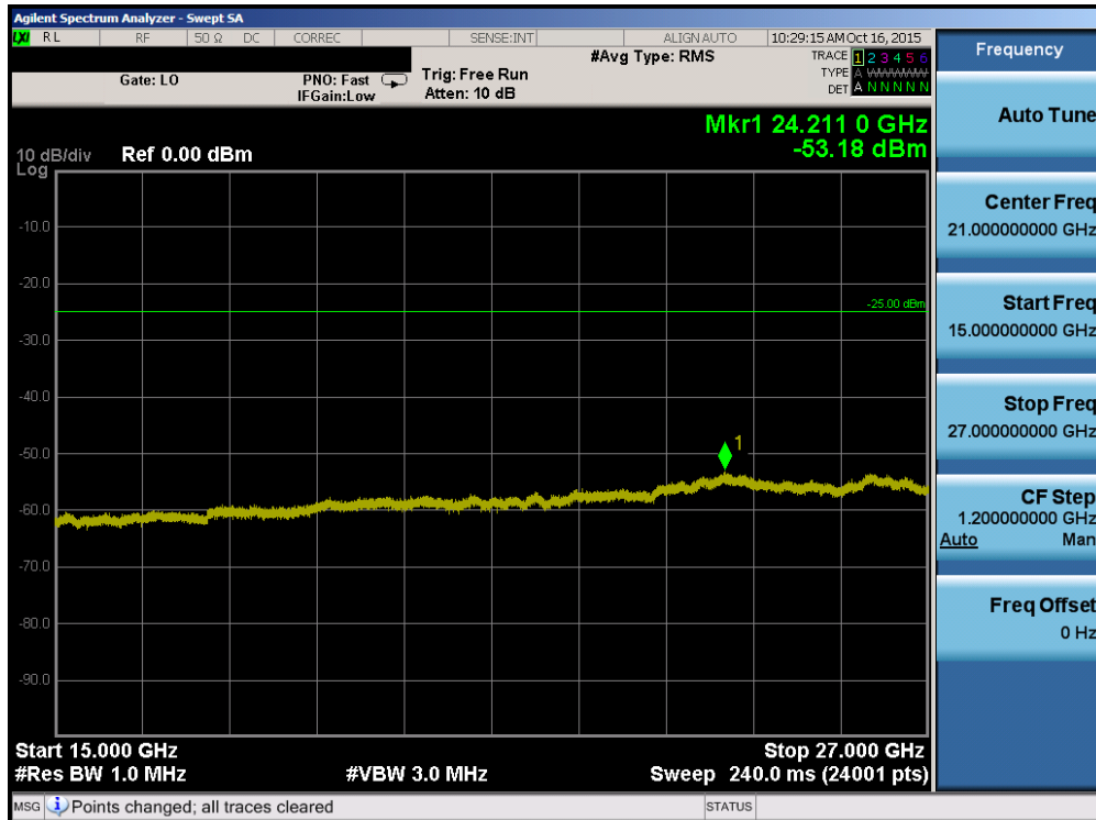
Plot 7-78. Conducted Spurious Plot (Band 41 – 20.0MHz QPSK – RB Size 1, RB Offset 0 – Low Channel)
