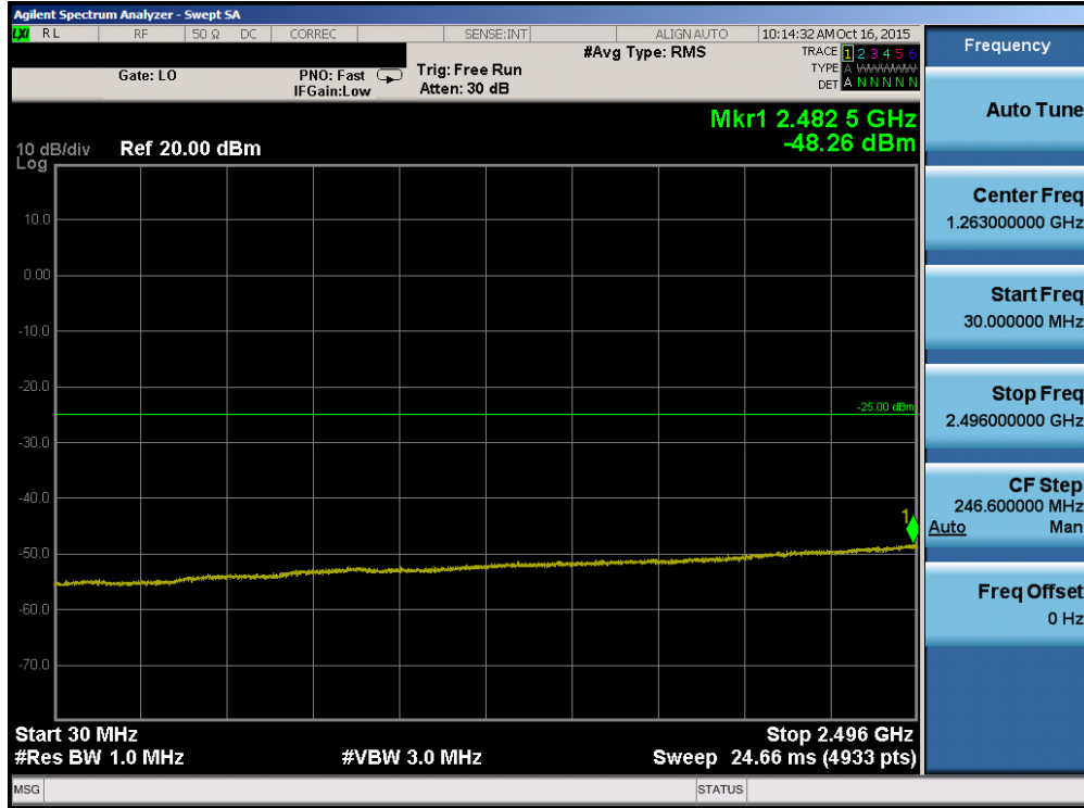
Plot 7-73. Conducted Spurious Plot (Band 41 – 15.0MHz QPSK – RB Size 1, RB Offset 0 – High Channel)
