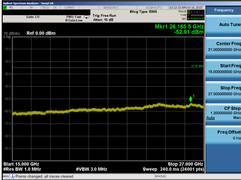
Plot 7-69. Conducted Spurious Plot (Band 41 – 15.0MHz QPSK – RB Size 1, RB Offset 0 – Low Channel)
