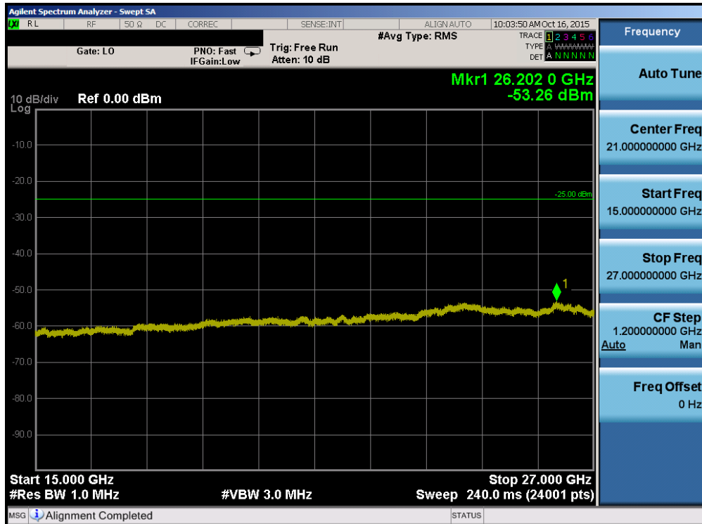
Plot 7-66. Conducted Spurious Plot (Band 41 – 10.0MHz QPSK – RB Size 1, RB Offset 0 – High Channel)
