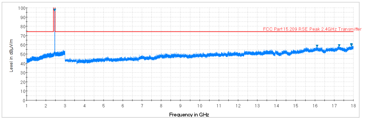
Plot 7-37. Radiated Spurious Plot above 1GHz (802.11b – Ch. 11, Ant. Pol. H)
