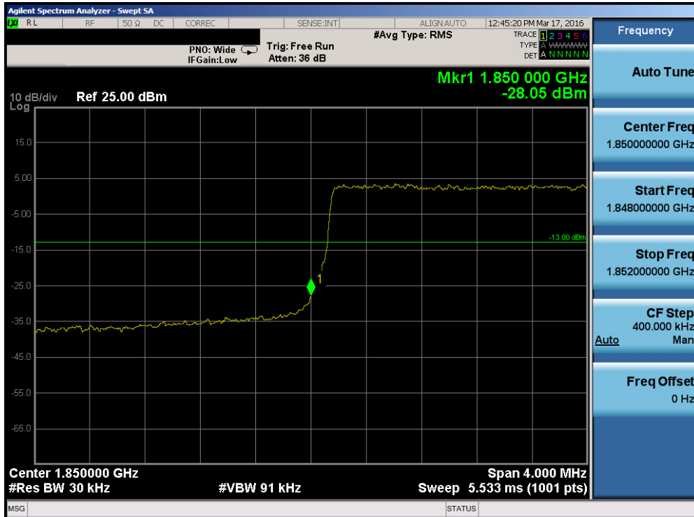
Plot 7-154. Lower Band Edge Plot (Band 25 – 3.0MHz QPSK – RB Size 15)
