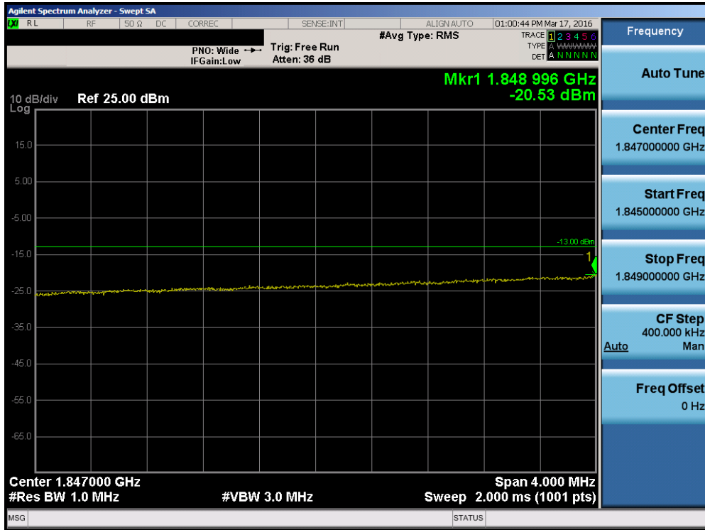
Plot 7-163. Lower Extended Band Edge Plot (Band 25 – 10.0MHz QPSK – RB Size 50)
