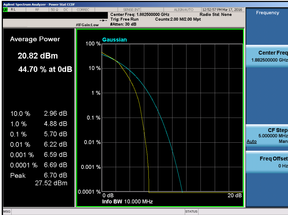
Plot 7-189. PAR Plot (Band 25 – 10.0MHz 16-QAM – RB Size 50)
