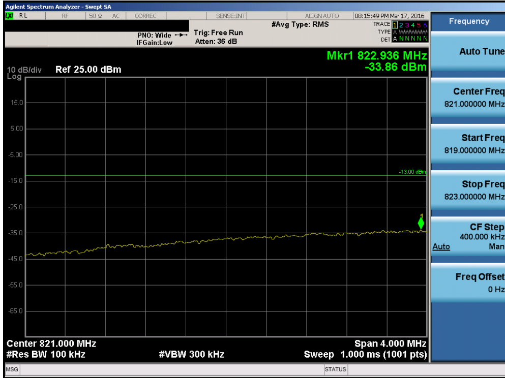
Plot 7-119. Lower Extended Band Edge Plot (Band 26 – 5.0MHz QPSK – RB Size 25)
