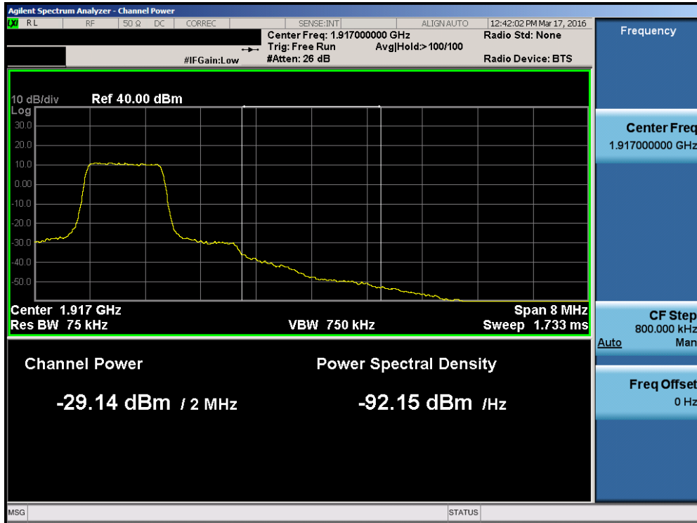
Plot 7-153. Upper Extended Band Edge Plot (Band 25 – 1.4MHz QPSK – RB Size 6)
