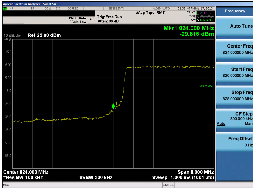
Plot 7-122. Lower Band Edge Plot (Band 26 – 10.0MHz QPSK – RB Size 50)
