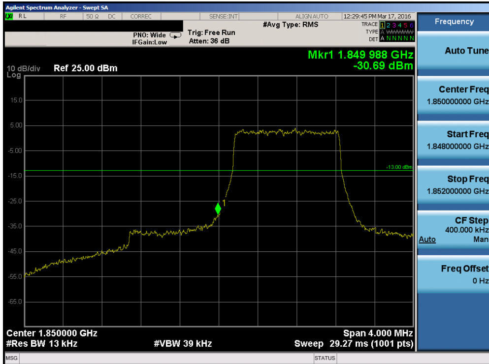
Plot 7-150. Lower Band Edge Plot (Band 25 – 1.4MHz QPSK – RB Size 6)
