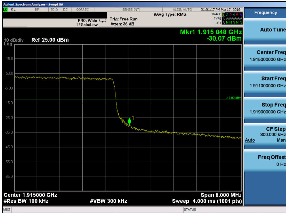
Plot 7-164. Upper Band Edge Plot (Band 25 – 10.0MHz QPSK – RB Size 50)
