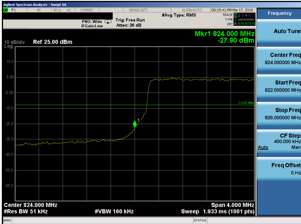
Plot 7-118. Lower Band Edge Plot (Band 26 – 5.0MHz QPSK – RB Size 25)
