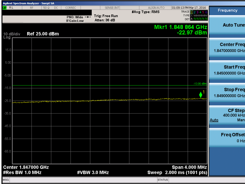
Plot 7-167. Lower Extended Band Edge Plot (Band 25 – 15.0MHz QPSK – RB Size 75)
