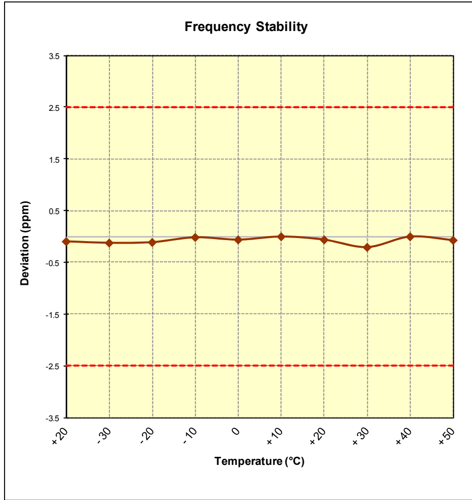
Figure 7-9. Frequency Stability Graph (Band 26)
