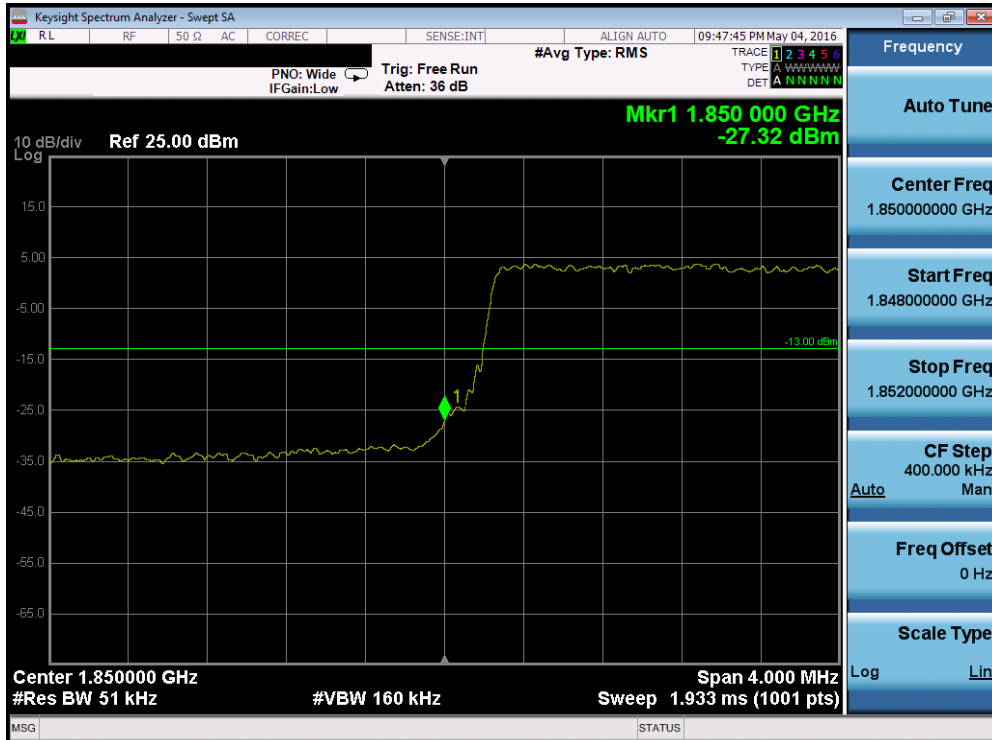
Plot 7-158. Lower Band Edge Plot (Band 25 – 5.0MHz QPSK – RB Size 25)
