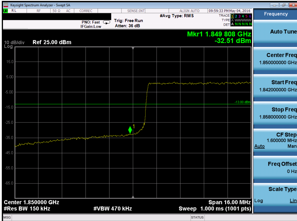
Plot 7-170. Lower Band Edge Plot (Band 25 – 20.0MHz QPSK – RB Size 100)
