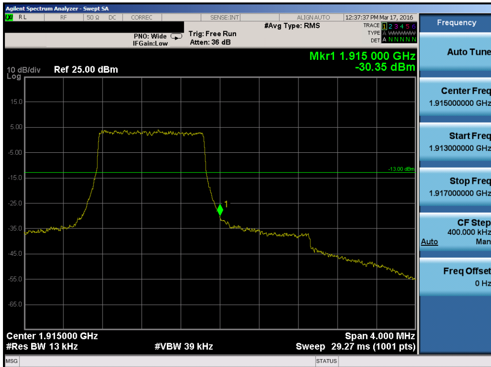
Plot 7-152. Upper Band Edge Plot (Band 25 – 1.4MHz QPSK – RB Size 6)
