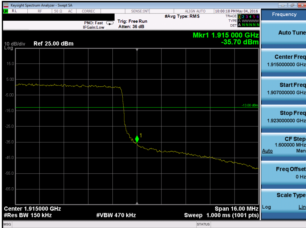
Plot 7-172. Upper Band Edge Plot (Band 25 – 20.0MHz QPSK – RB Size 100)
