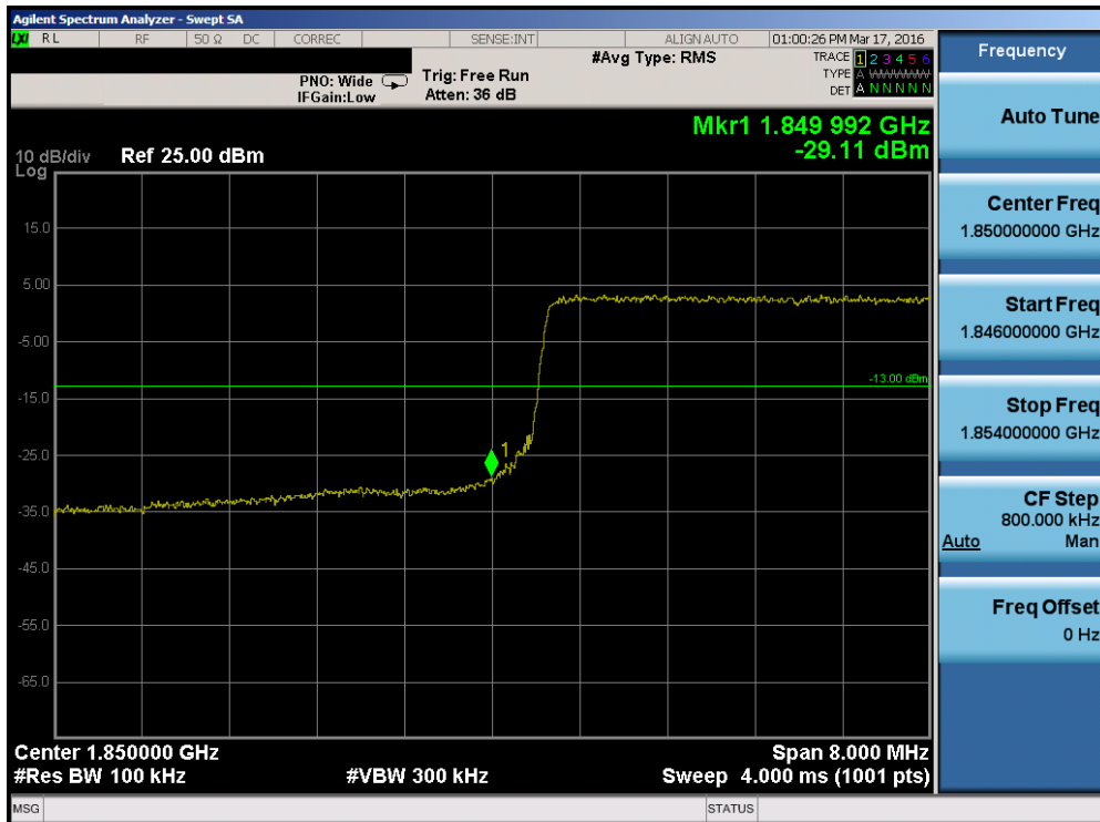
Plot 7-162. Lower Band Edge Plot (Band 25 – 10.0MHz QPSK – RB Size 50)
