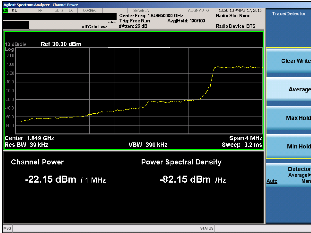
Plot 7-151. Lower Extended Band Edge Plot (Band 25 – 1.4MHz QPSK – RB Size 6)
