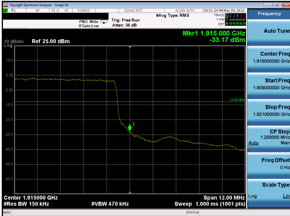
Plot 7-168. Upper Band Edge Plot (Band 25 – 15.0MHz QPSK – RB Size 75)
