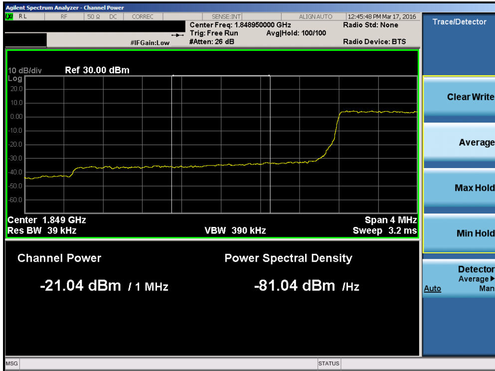
Plot 7-155. Lower Extended Band Edge Plot (Band 25 – 3.0MHz QPSK – RB Size 15)
