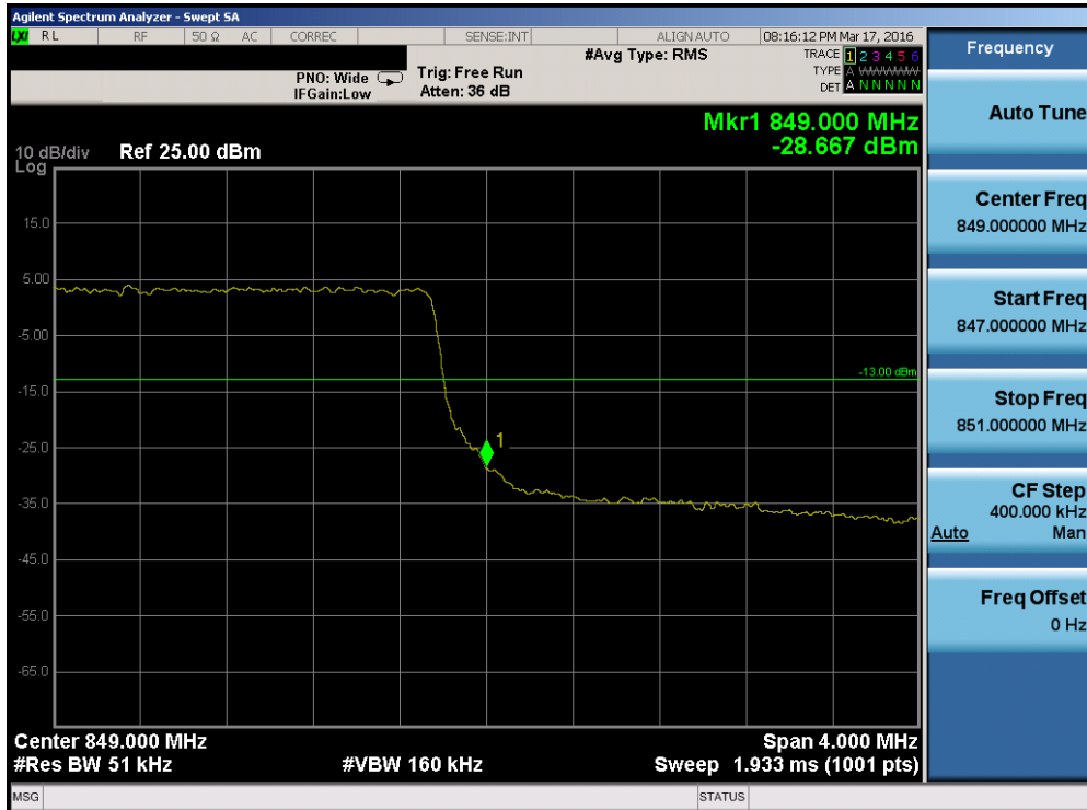
Plot 7-120. Upper Band Edge Plot (Band 26 – 5.0MHz QPSK – RB Size 25)
