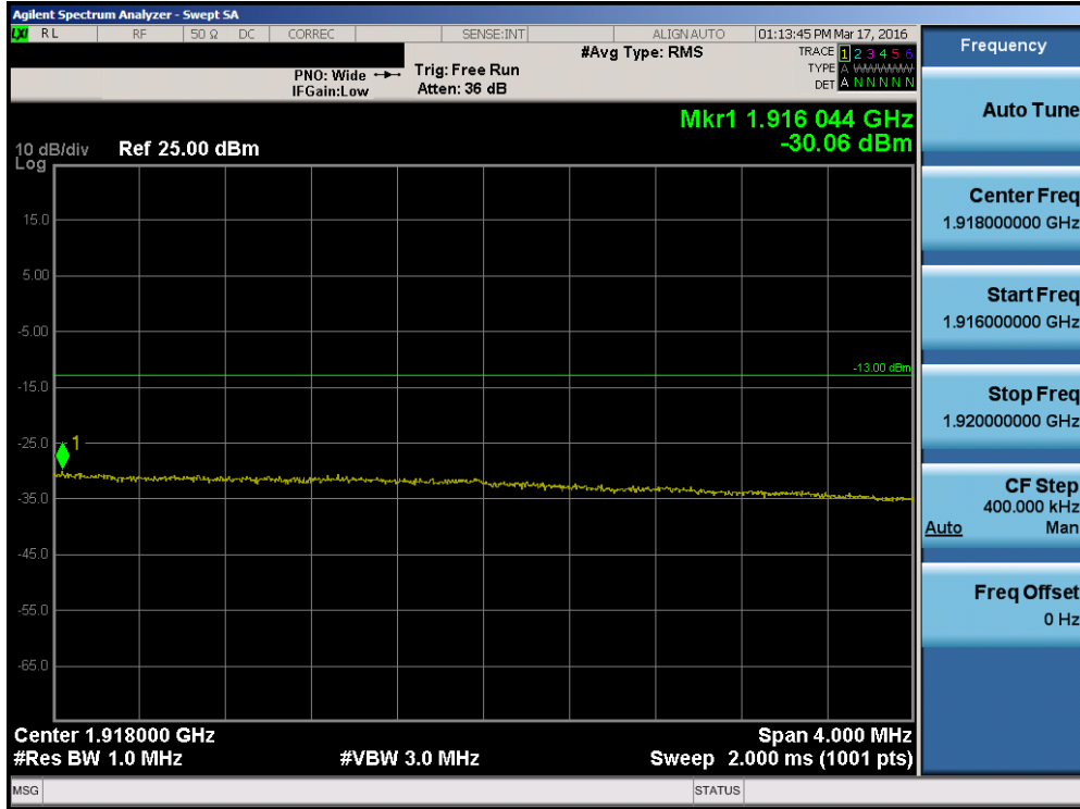
Plot 7-173. Upper Extended Band Edge Plot (Band 25 – 20.0MHz QPSK – RB Size 100)
