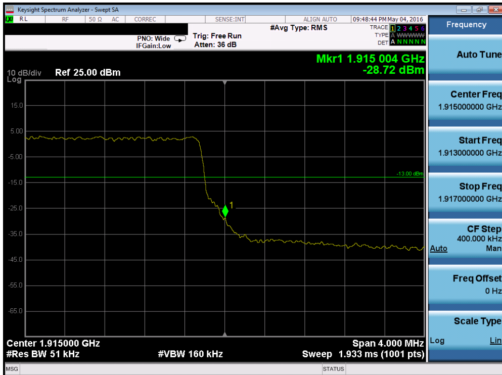
Plot 7-160. Upper Band Edge Plot (Band 25 – 5.0MHz QPSK – RB Size 25)
