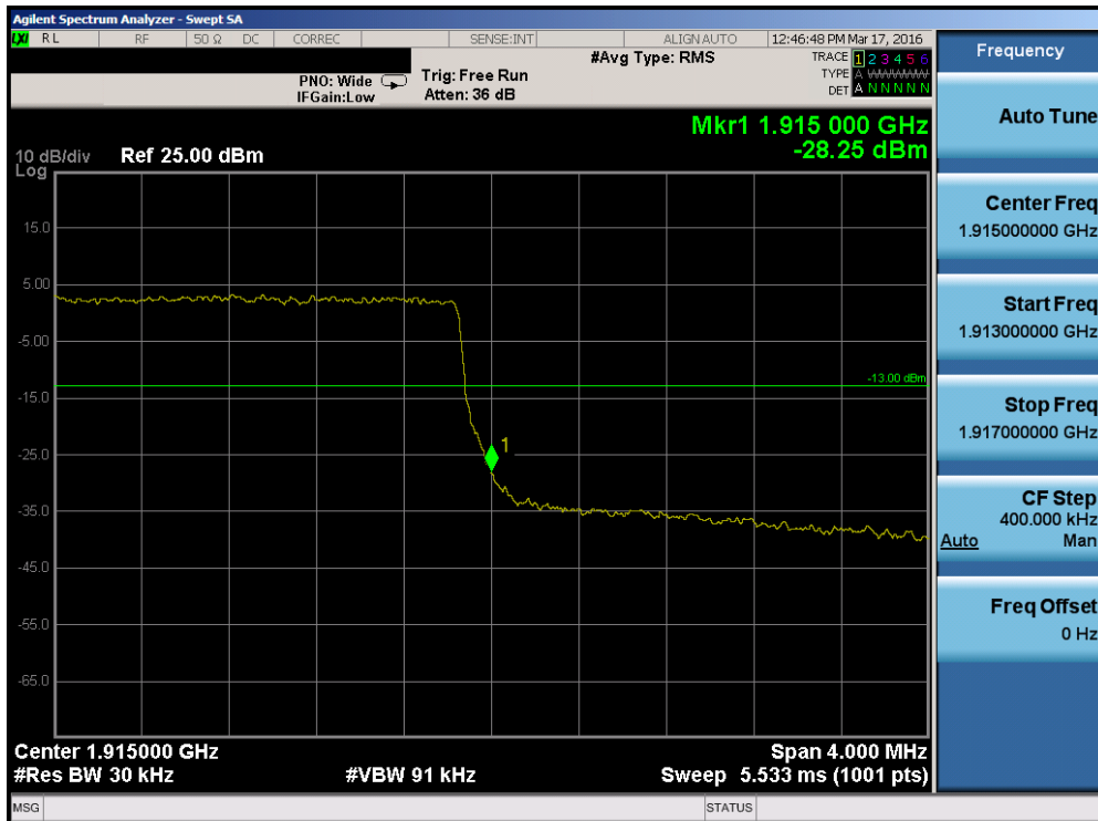
Plot 7-156. Upper Band Edge Plot (Band 25 – 3.0MHz QPSK – RB Size 15)
