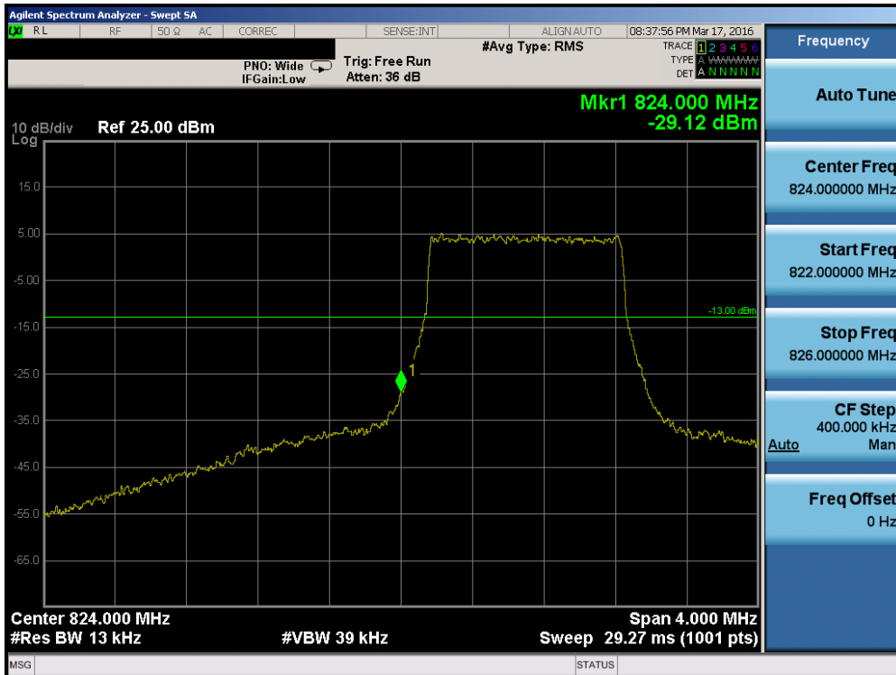
Plot 7-110. Lower Band Edge Plot (Band 26 – 1.4MHz QPSK – RB Size 6)
