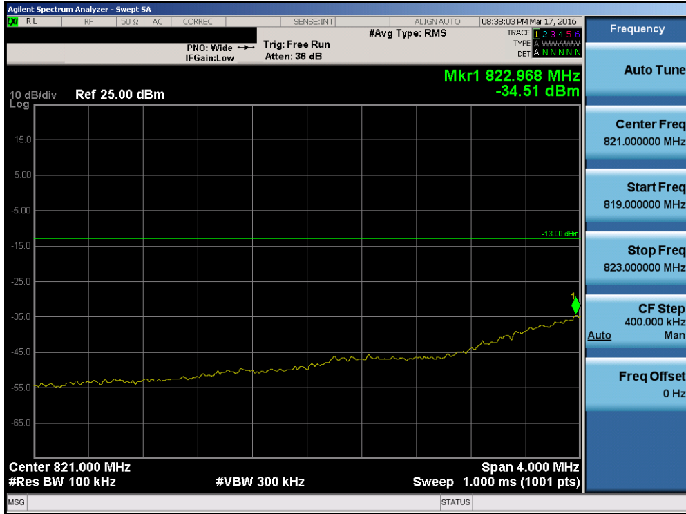
Plot 7-111. Lower Extended Band Edge Plot (Band 26 – 1.4MHz QPSK – RB Size 6)
