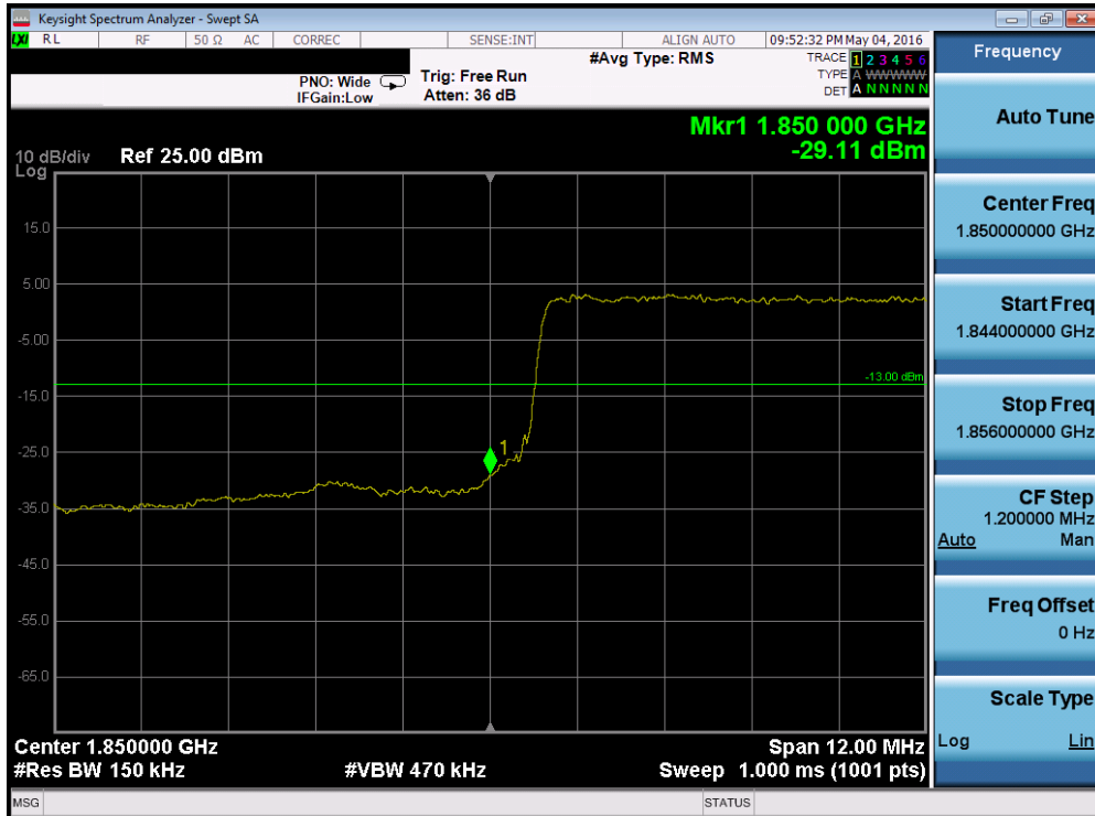
Plot 7-166. Lower Band Edge Plot (Band 25 – 15.0MHz QPSK – RB Size 75)
