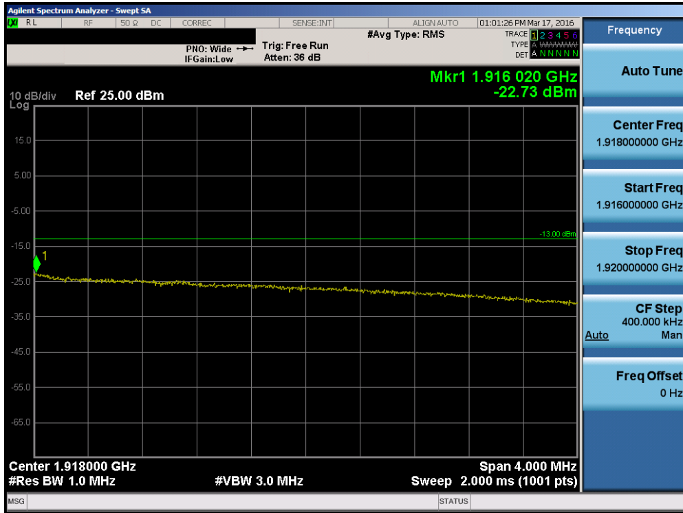
Plot 7-165. Upper Extended Band Edge Plot (Band 25 – 10.0MHz QPSK – RB Size 50)
