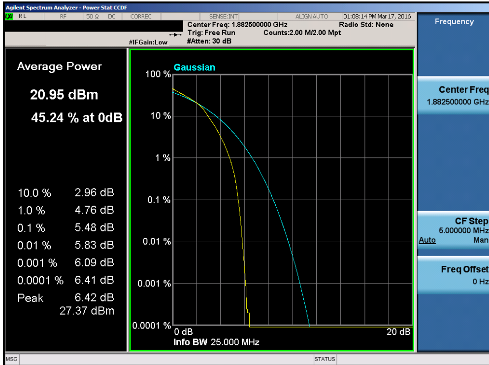
Plot 7-191. PAR Plot (Band 25 – 15.0MHz 16-QAM – RB Size 75)
