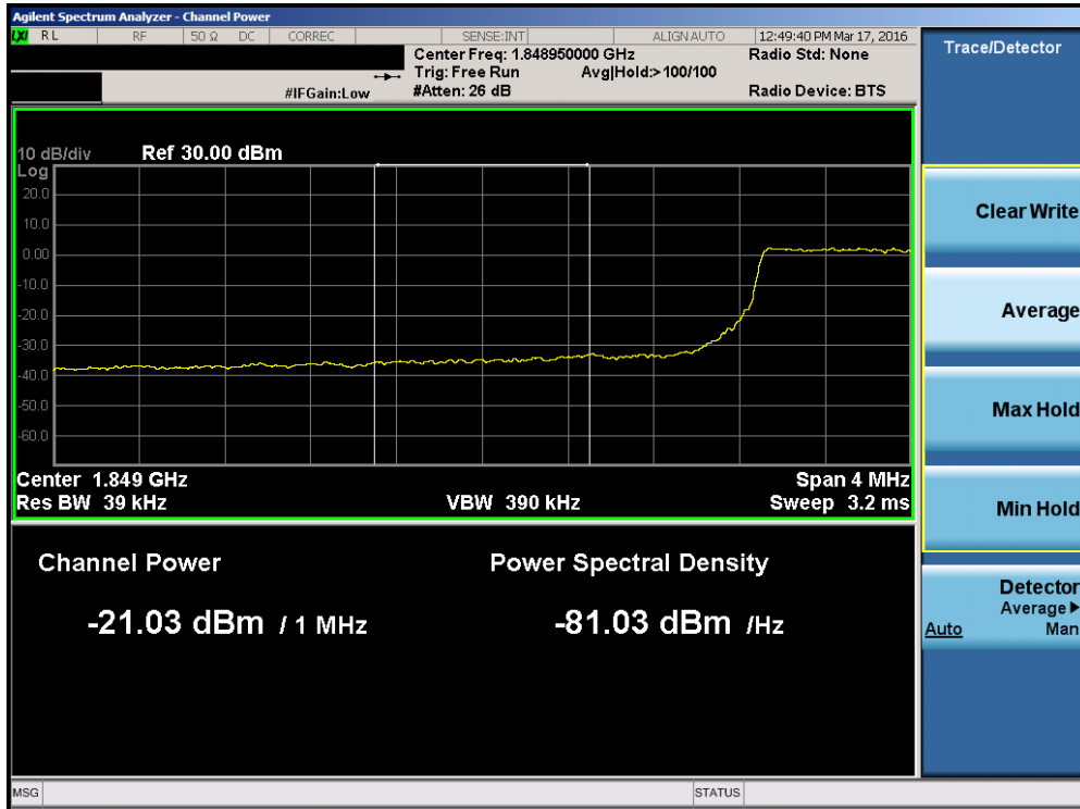
Plot 7-159. Lower Extended Band Edge Plot (Band 25 – 5.0MHz QPSK – RB Size 25)
