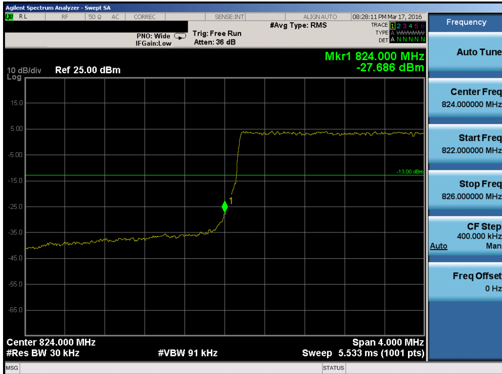
Plot 7-114. Lower Band Edge Plot (Band 26 – 3.0MHz QPSK – RB Size 15)
