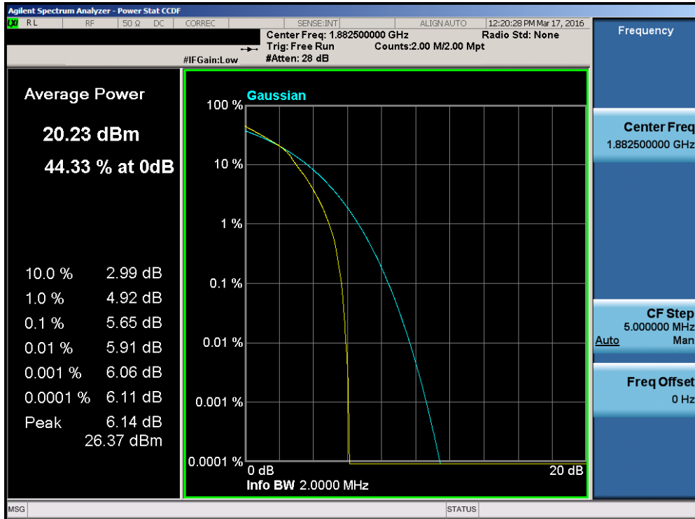
Plot 7-183. PAR Plot (Band 25 – 1.4MHz 16-QAM – RB Size 6)
