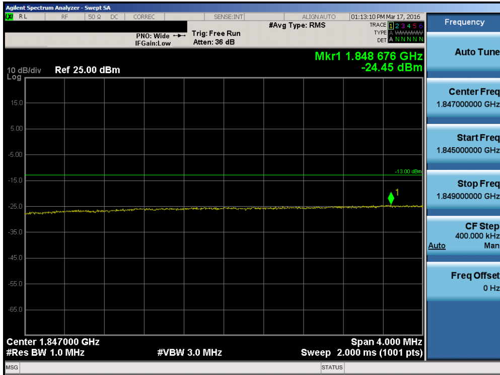
Plot 7-171. Lower Extended Band Edge Plot (Band 25 – 20.0MHz QPSK – RB Size 100)
