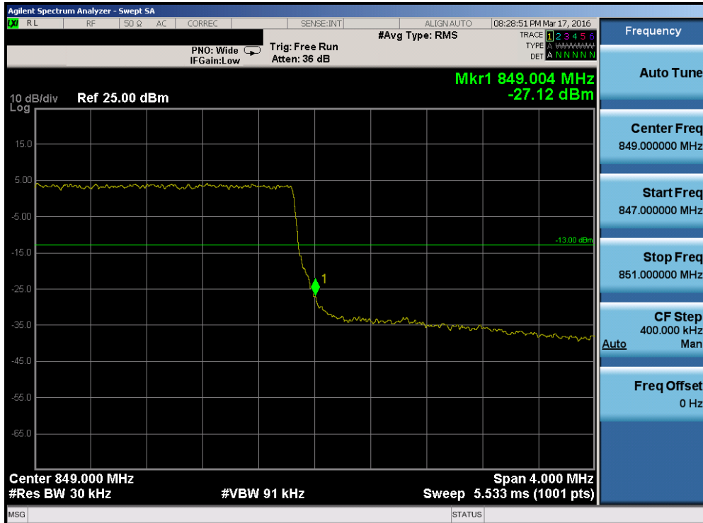
Plot 7-116. Upper Band Edge Plot (Band 26 – 3.0MHz QPSK – RB Size 15)
