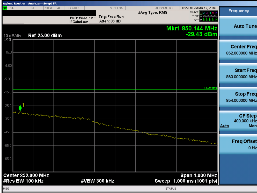
Plot 7-117. Upper Extended Band Edge Plot (Band 26 – 3.0MHz QPSK – RB Size 15)
