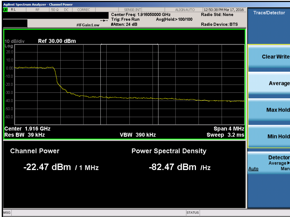
Plot 7-161. Upper Extended Band Edge Plot (Band 25 – 5.0MHz QPSK – RB Size 25)
