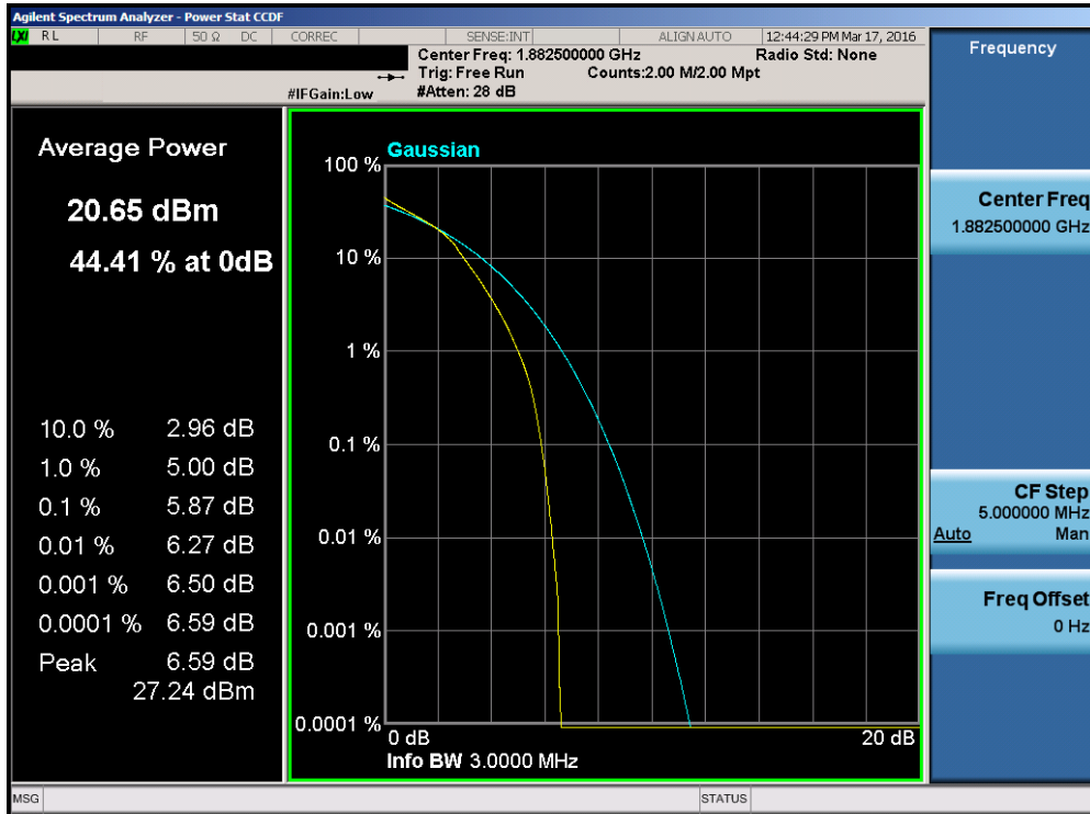
Plot 7-185. PAR Plot (Band 25 – 3.0MHz 16-QAM – RB Size 15)
