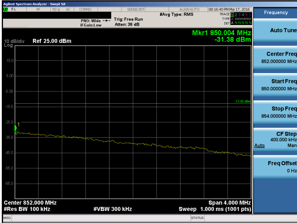
Plot 7-121. Upper Extended Band Edge Plot (Band 26 – 5.0MHz QPSK – RB Size 25)
