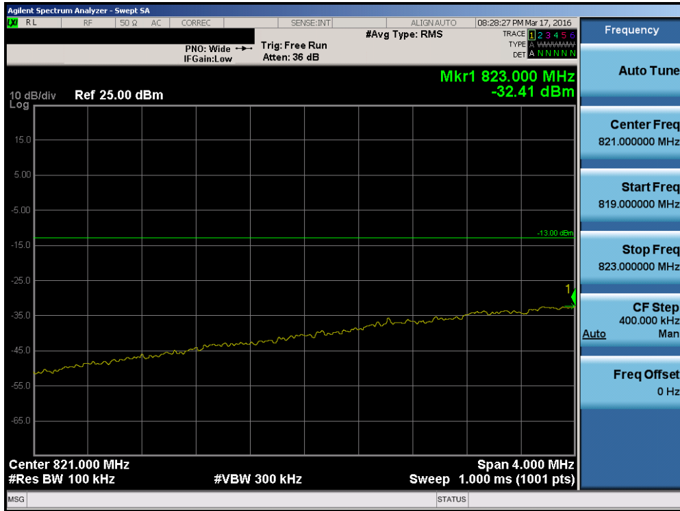
Plot 7-115. Lower Extended Band Edge Plot (Band 26 – 3.0MHz QPSK – RB Size 15)
