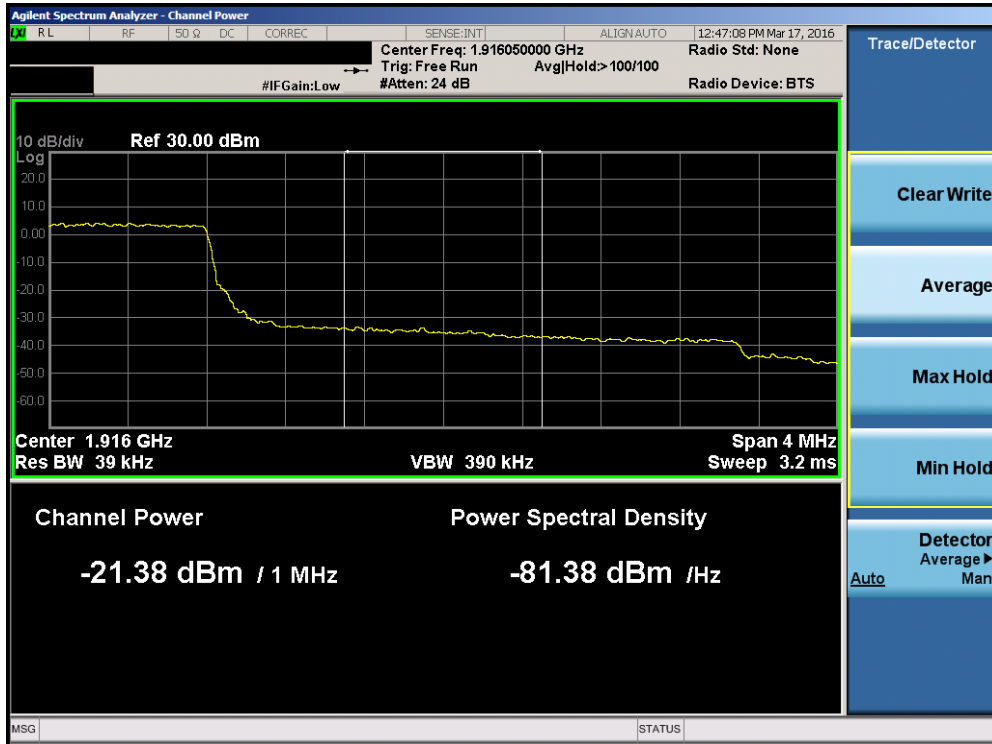
Plot 7-157. Upper Extended Band Edge Plot (Band 25 – 3.0MHz QPSK – RB Size 15)
