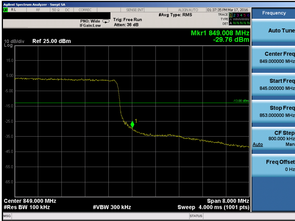
Plot 7-123. Upper Band Edge Plot (Band 26 – 10.0MHz QPSK – RB Size 50)
