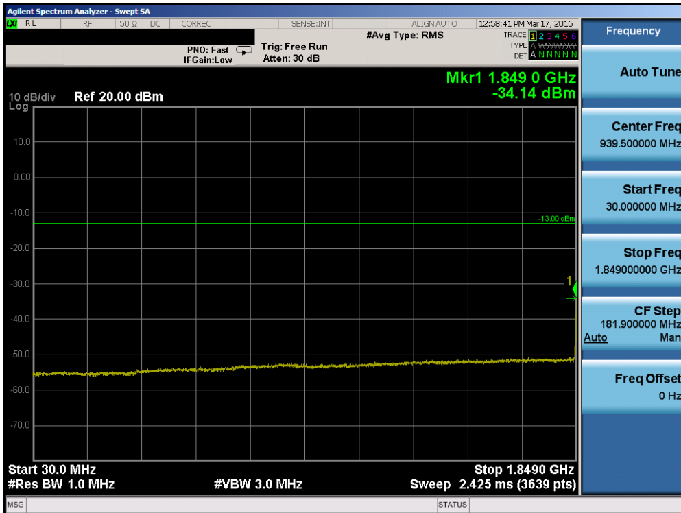
Plot 7-78. Conducted Spurious Plot (Band 25 – 10.0MHz QPSK – RB Size 1, RB Offset 0– Low Channel)
