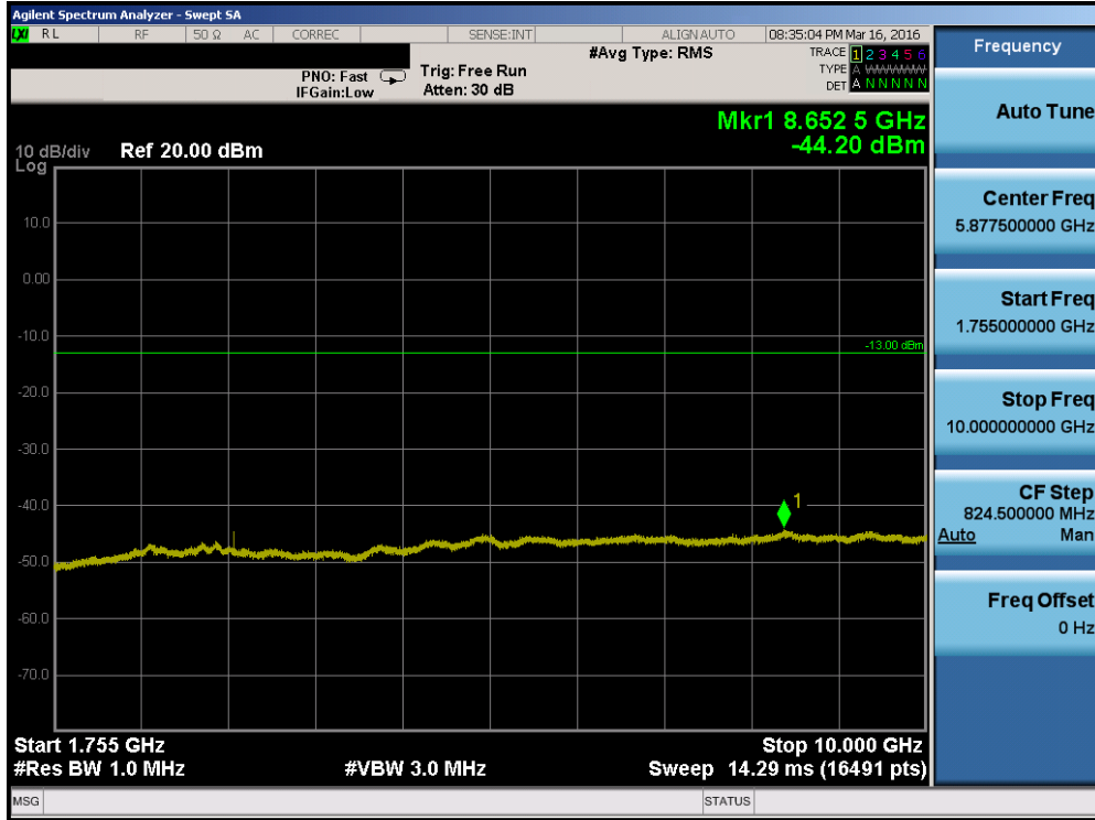
Plot 7-73. Conducted Spurious Plot (Band 4 – 10.0MHz QPSK – RB Size 1, RB Offset 0 – Mid Channel)
