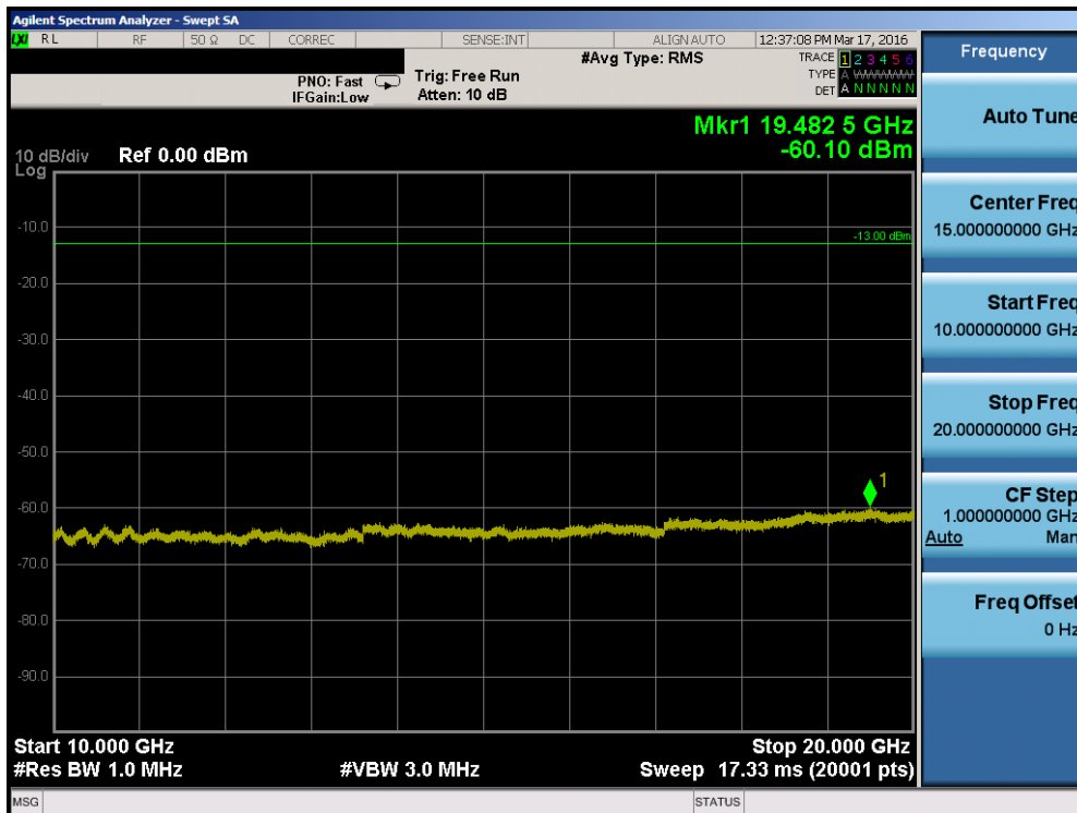
Plot 7-86. Conducted Spurious Plot (Band 25 – 10.0MHz QPSK – RB Size 1, RB Offset 0 – High Channel)
