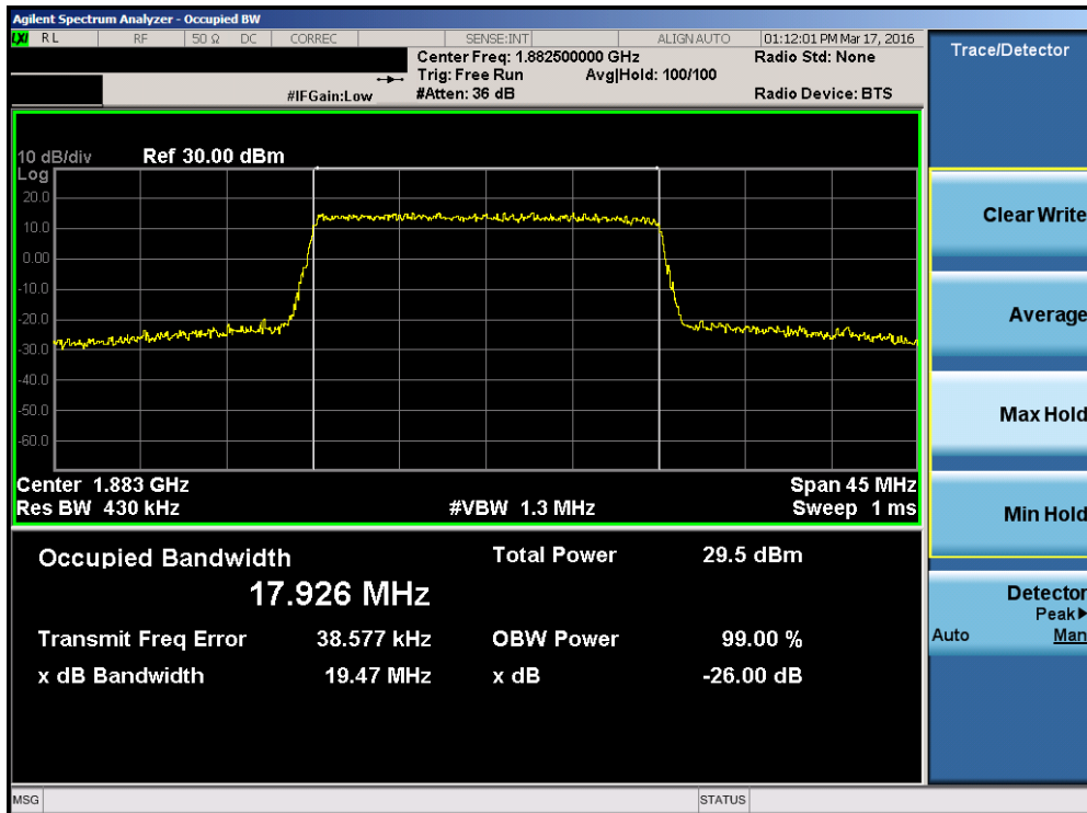
Plot 7-42. Occupied Bandwidth Plot (Band 25 – 20.0MHz 16-QAM – RB Size 100)
