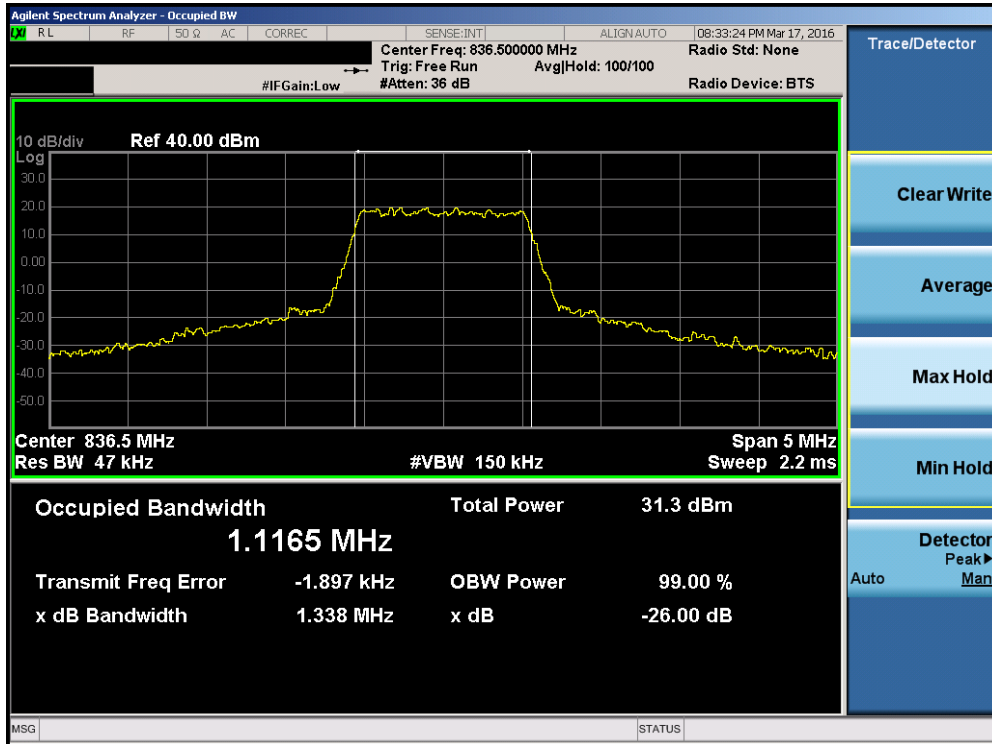
Plot 7-9. Occupied Bandwidth Plot (Band 26 – 1.4MHz QPSK – RB Size 6)
