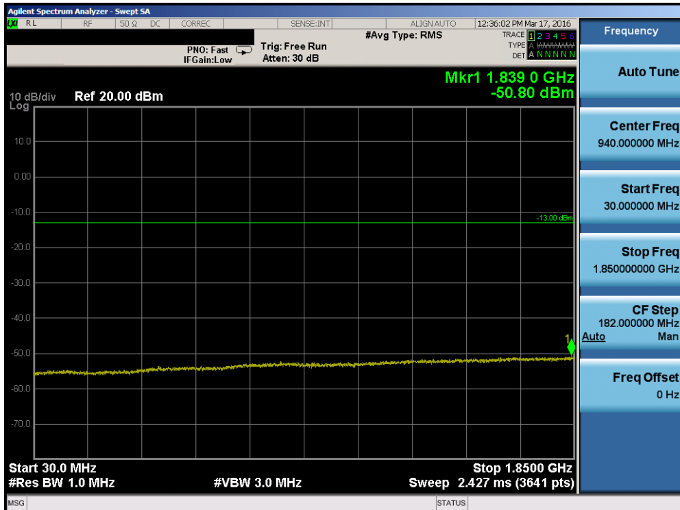
Plot 7-84. Conducted Spurious Plot (Band 25 – 10.0MHz QPSK – RB Size 1, RB Offset 0 – High Channel)
