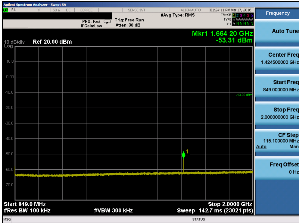
Plot 7-64. Conducted Spurious Plot (Band 26 – 10.0MHz QPSK – RB Size 1, RB Offset 0 – Mid Channel)
