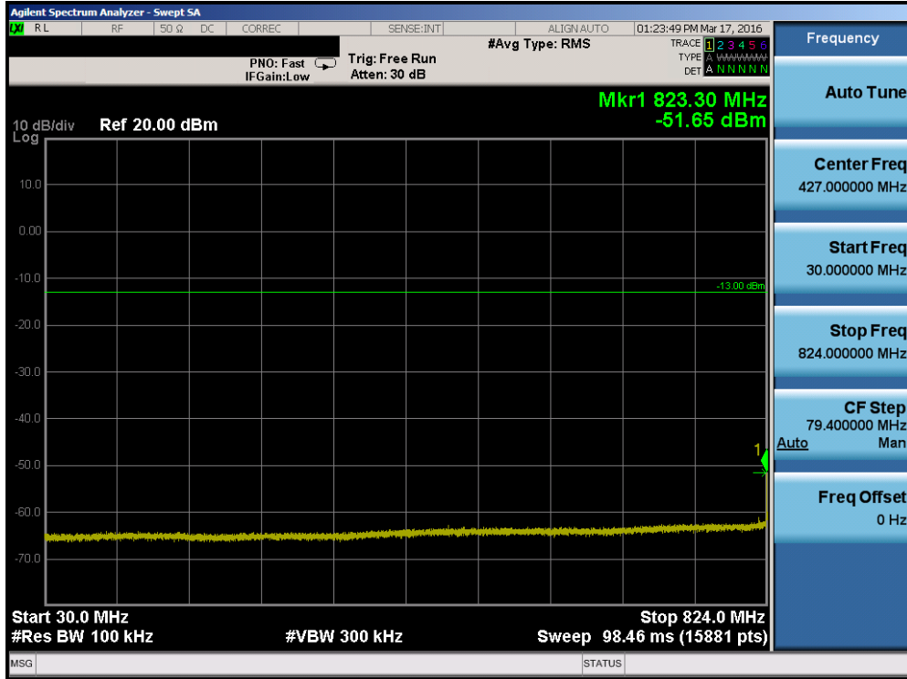
Plot 7-63. Conducted Spurious Plot (Band 26 – 10.0MHz QPSK – RB Size 1, RB Offset 0 – Mid Channel)
