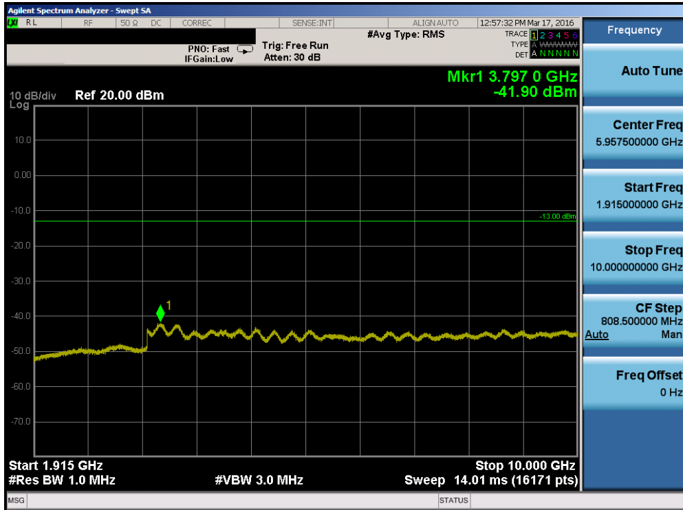
Plot 7-82. Conducted Spurious Plot (Band 25 – 10.0MHz QPSK – RB Size 1, RB Offset 0 – Mid Channel)
