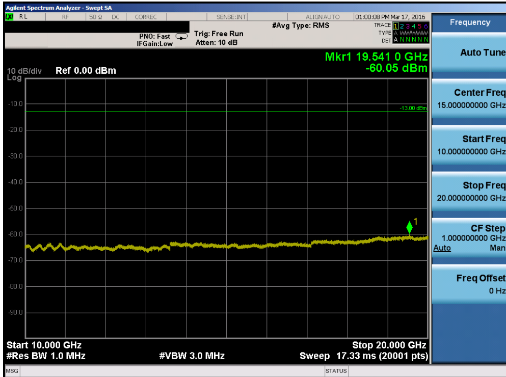
Plot 7-80. Conducted Spurious Plot (Band 25 – 10.0MHz QPSK – RB Size 1, RB Offset 0 – Low Channel)
