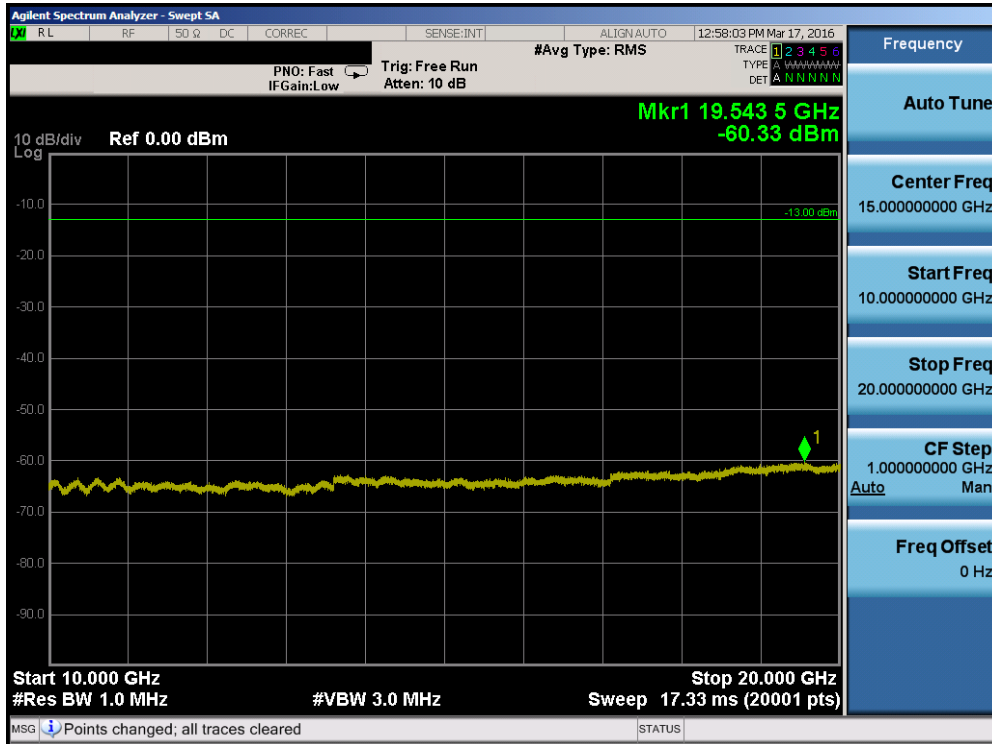
Plot 7-83. Conducted Spurious Plot (Band 25 – 10.0MHz QPSK – RB Size 1, RB Offset 0 – Mid Channel)
