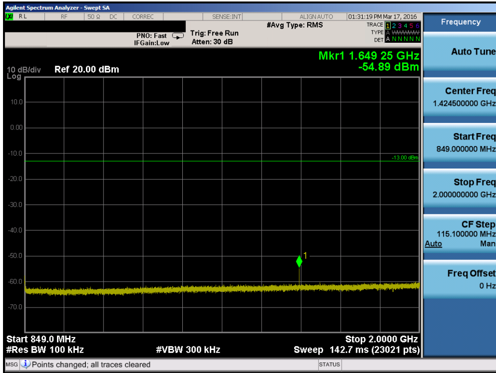
Plot 7-61. Conducted Spurious Plot (Band 26 – 10.0MHz QPSK – RB Size 1, RB Offset 0 – Low Channel)
