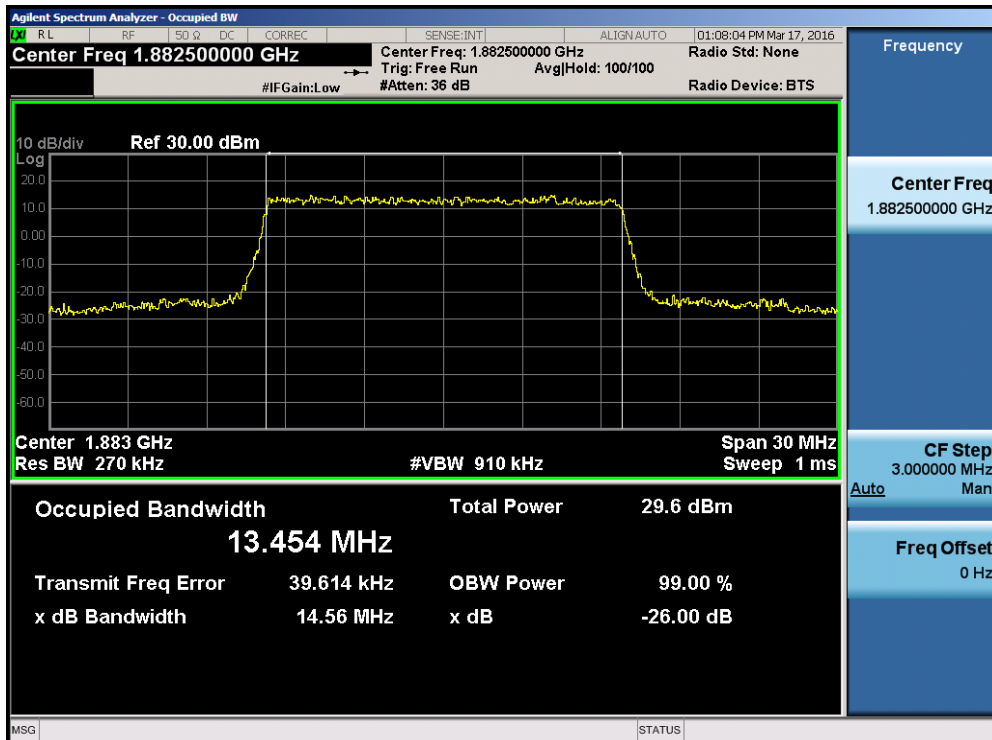
Plot 7-40. Occupied Bandwidth Plot (Band 25 – 15.0MHz 16-QAM – RB Size 75)
