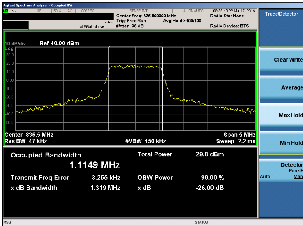
Plot 7-10. Occupied Bandwidth Plot (Band 26 – 1.4MHz 16-QAM – RB Size 6)
