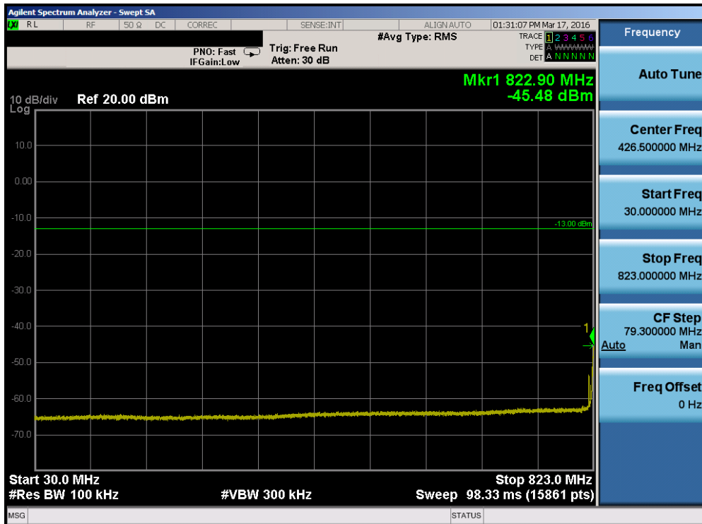
Plot 7-60. Conducted Spurious Plot (Band 26 – 10.0MHz QPSK – RB Size 1, RB Offset 0– Low Channel)
