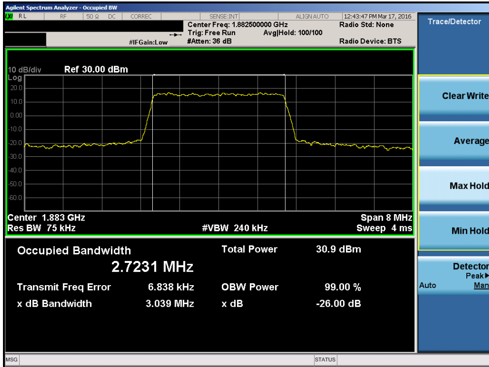
Plot 7-33. Occupied Bandwidth Plot (Band 25 – 3.0MHz QPSK – RB Size 15)
