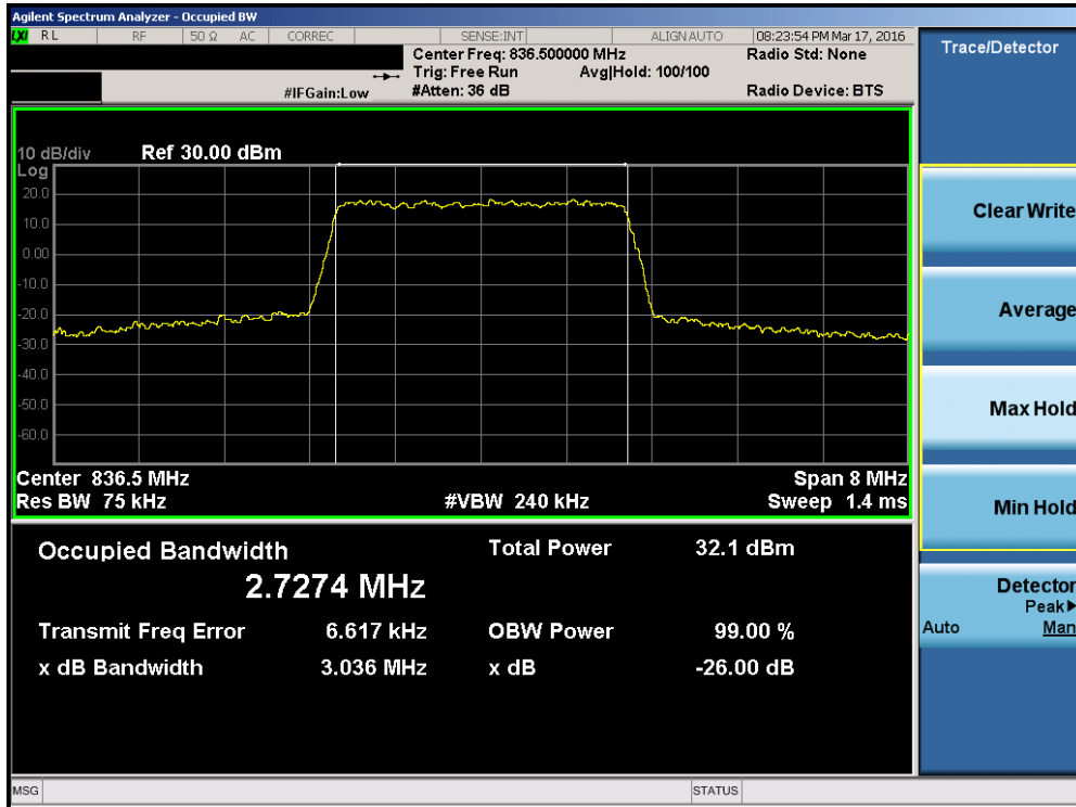
Plot 7-11. Occupied Bandwidth Plot (Band 26 – 3.0MHz QPSK – RB Size 15)
