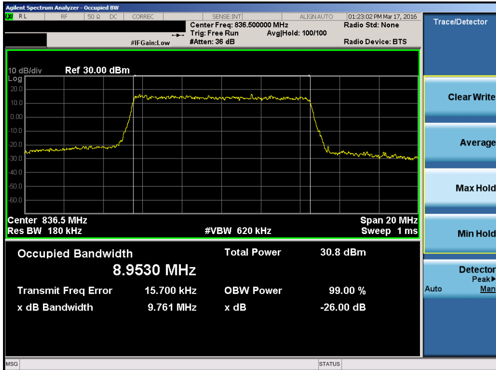
Plot 7-16. Occupied Bandwidth Plot (Band 26 – 10.0MHz 16-QAM – RB Size 50)
