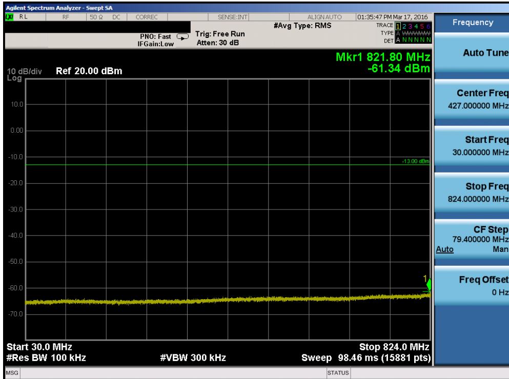
Plot 7-66. Conducted Spurious Plot (Band 26 – 10.0MHz QPSK – RB Size 1, RB Offset 0 – High Channel)
