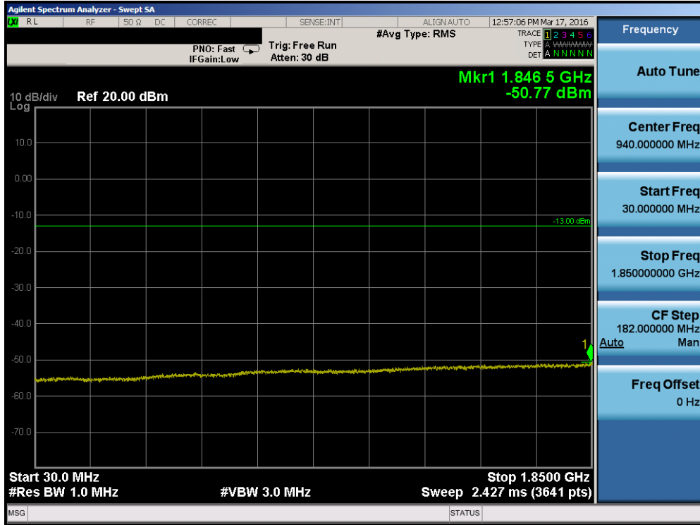
Plot 7-81. Conducted Spurious Plot (Band 25 – 10.0MHz QPSK – RB Size 1, RB Offset 0 – Mid Channel)
