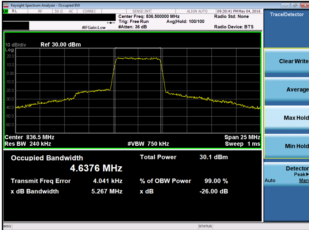
Plot 7-14. Occupied Bandwidth Plot (Band 26 – 5.0MHz 16-QAM – RB Size 25)
