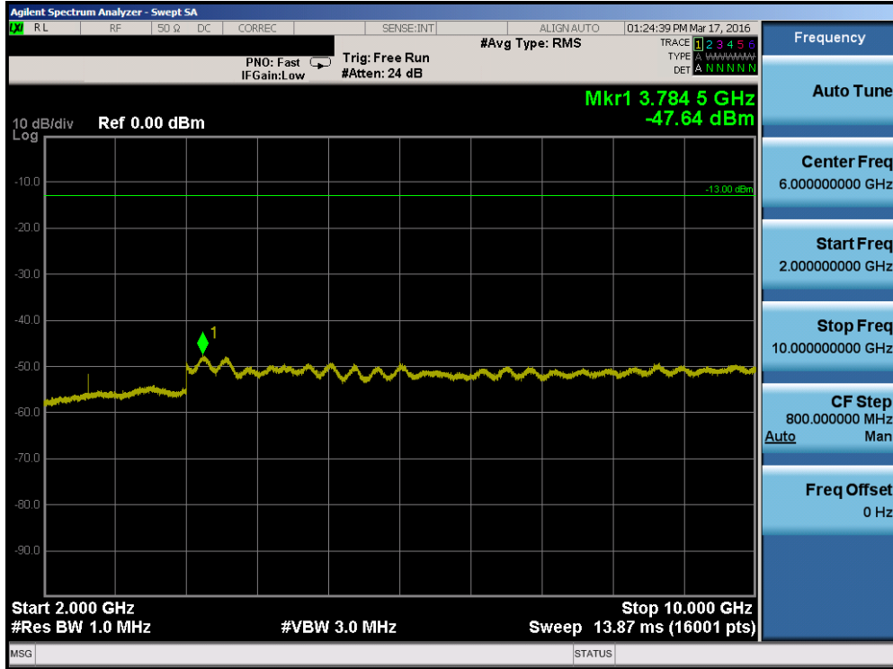
Plot 7-65. Conducted Spurious Plot (Band 26 – 10.0MHz QPSK – RB Size 1, RB Offset 0 – Mid Channel)
