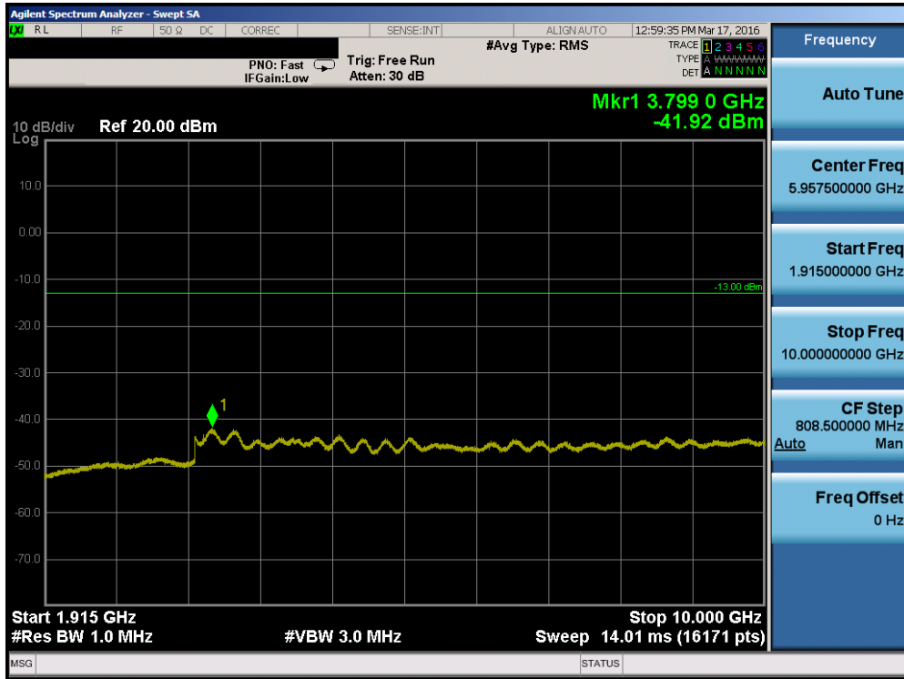
Plot 7-79. Conducted Spurious Plot (Band 25 – 10.0MHz QPSK – RB Size 1, RB Offset 0 – Low Channel)
