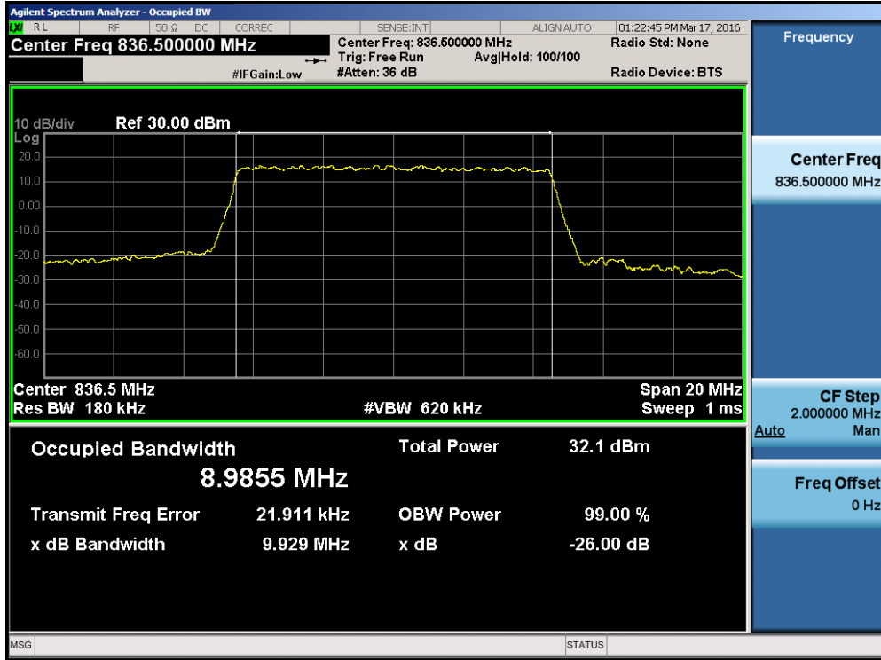
Plot 7-15. Occupied Bandwidth Plot (Band 26 – 10.0MHz QPSK – RB Size 50)
