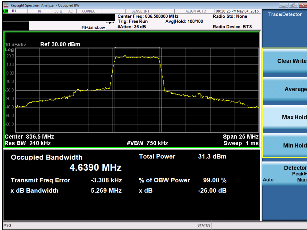
Plot 7-13. Occupied Bandwidth Plot (Band 26 – 5.0MHz QPSK – RB Size 25)
