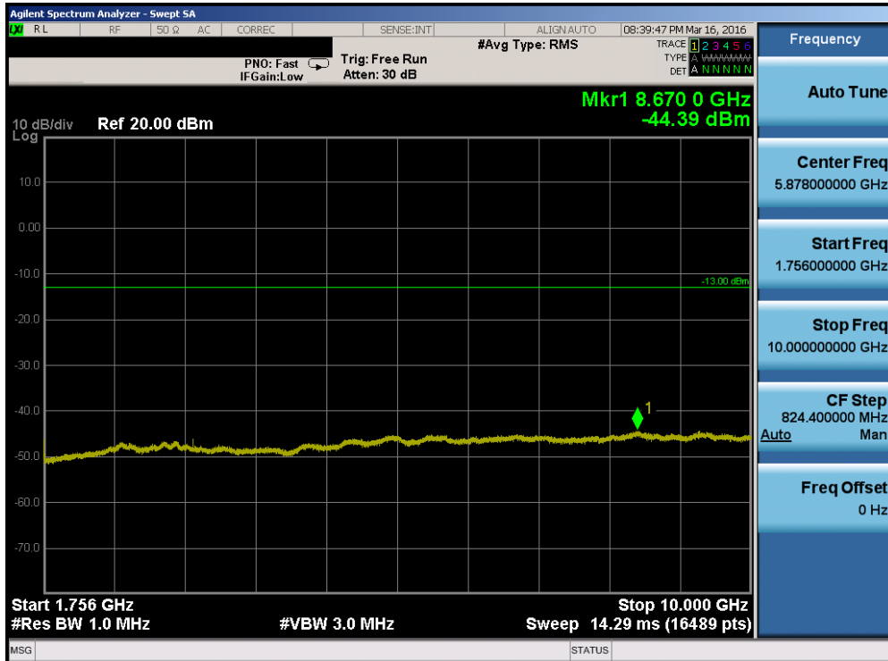
Plot 7-76. Conducted Spurious Plot (Band 4 – 10.0MHz QPSK – RB Size 1, RB Offset 0 – High Channel)
