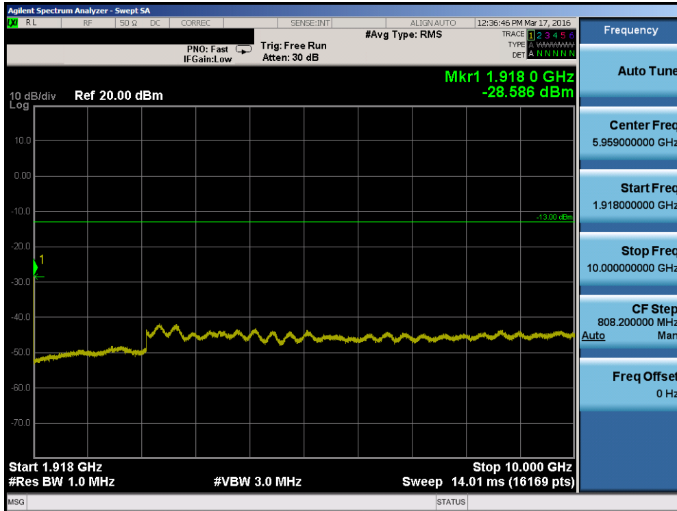
Plot 7-85. Conducted Spurious Plot (Band 25 – 10.0MHz QPSK – RB Size 1, RB Offset 0 – High Channel)
