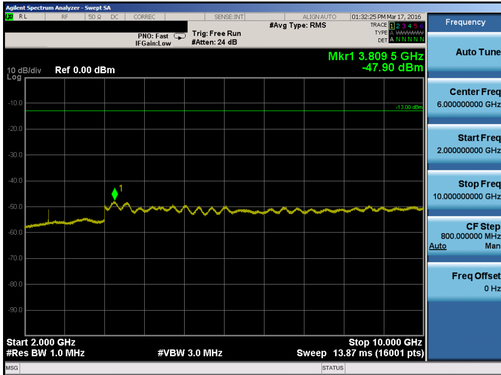
Plot 7-62. Conducted Spurious Plot (Band 26 – 10.0MHz QPSK – RB Size 1, RB Offset 0 – Low Channel)
