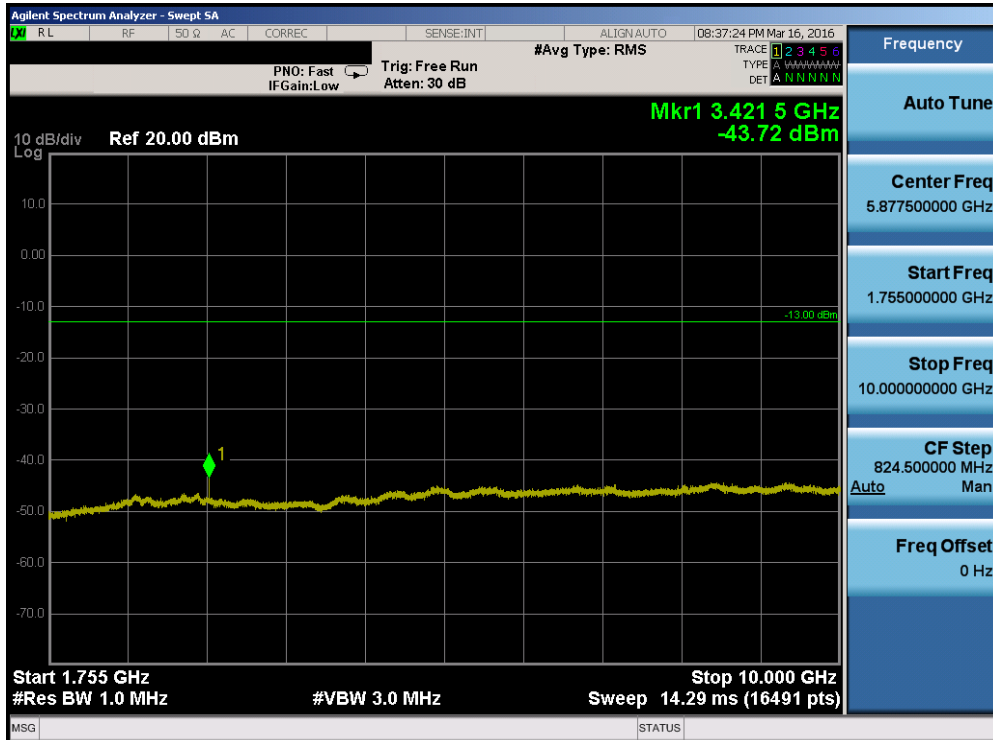
Plot 7-70. Conducted Spurious Plot (Band 4 – 10.0MHz QPSK – RB Size 1, RB Offset 0 – Low Channel)
