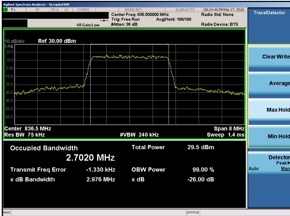
Plot 7-12. Occupied Bandwidth Plot (Band 26 – 3.0MHz 16-QAM – RB Size 15)
