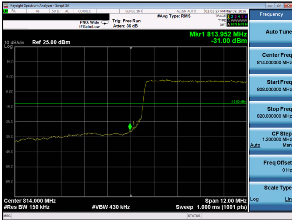
Plot 7-34. Lower Band Edge Plot (15MHz QPSK – RB Size 75)
