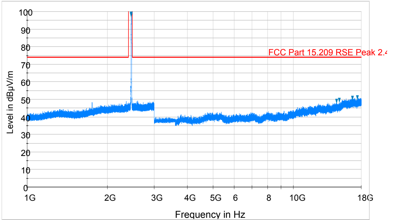
Plot 6-5. Radiated Spurious Plot above 1GHz (802.11b – Ch. 11, Ant. Pol. H)
