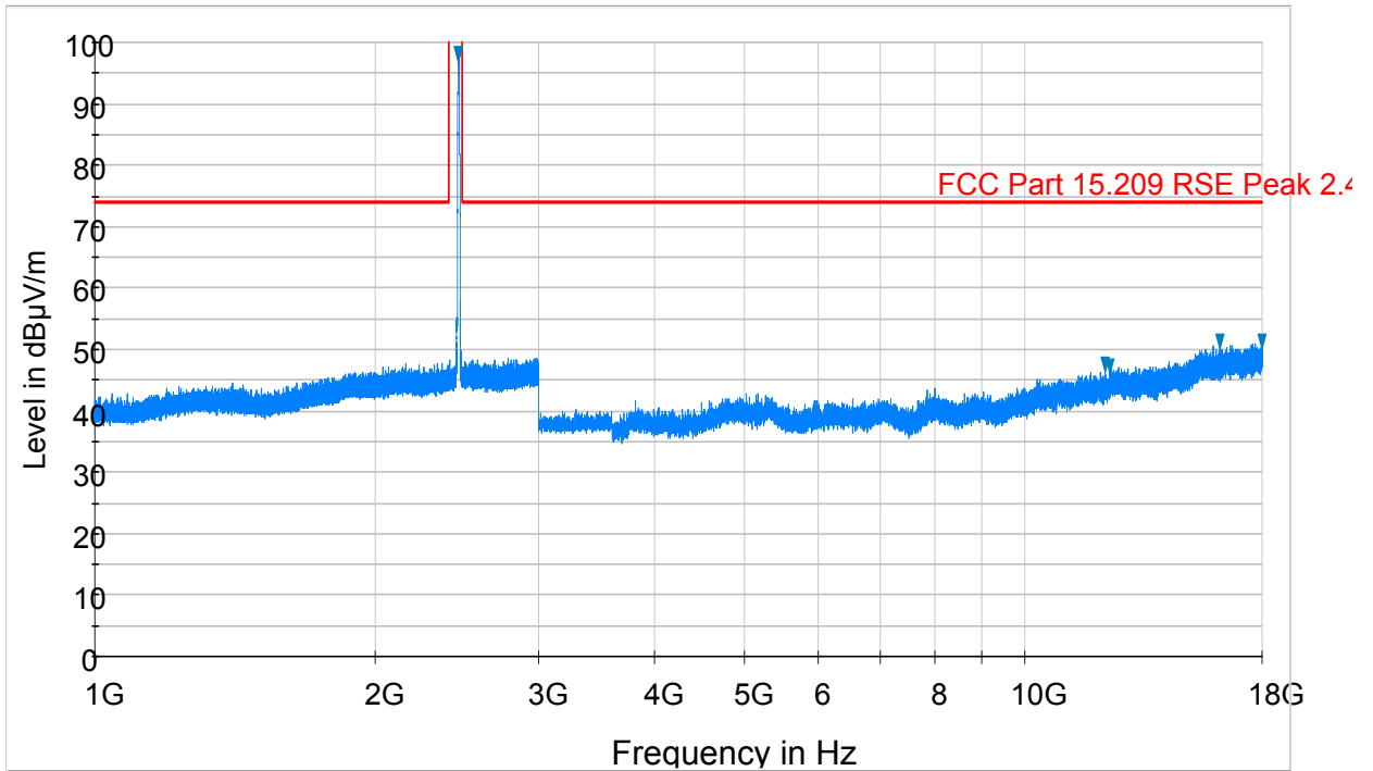
Plot 6-6. Radiated Spurious Plot above 1GHz (802.11b – Ch. 11, Ant. Pol. V)
