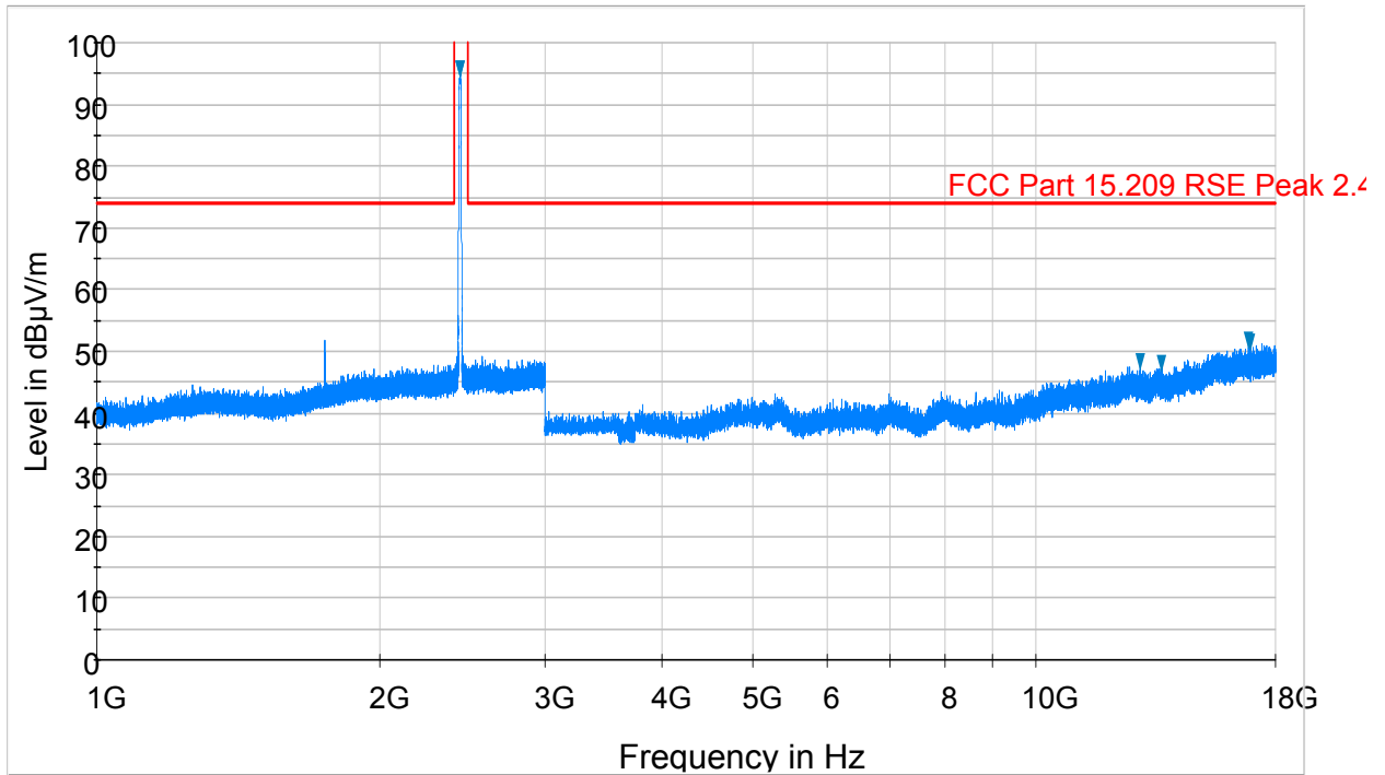
Plot 6-4. Radiated Spurious Plot above 1GHz (802.11b – Ch. 6, Ant. Pol. V)
