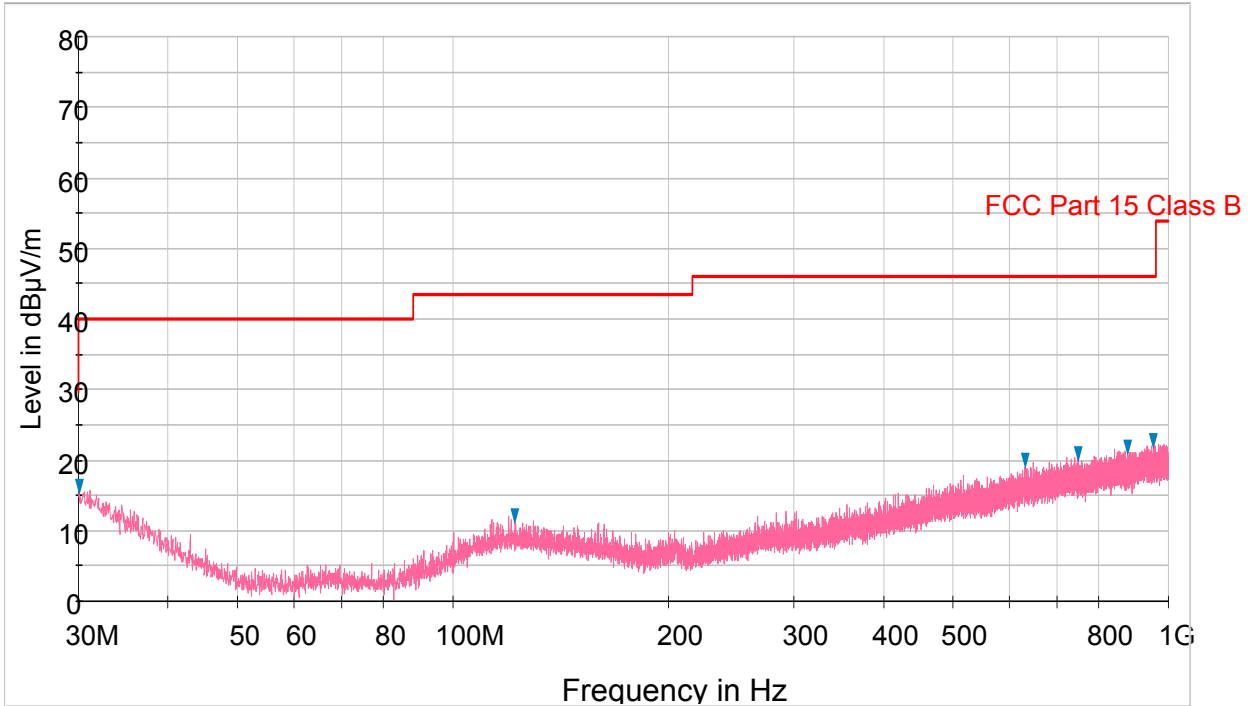
Plot 6-13. Radiated Spurious Plot below 1GHz (Pol. H)
