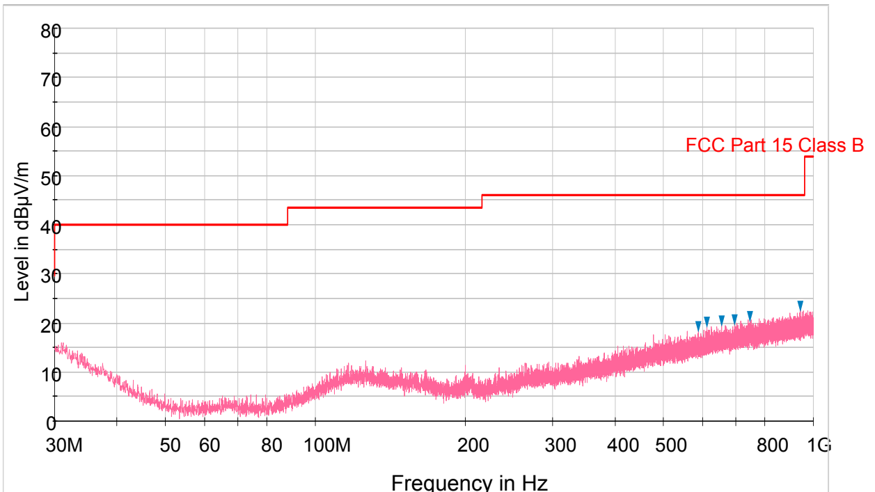
Plot 6-14. Radiated Spurious Plot below 1GHz (Pol. V)
