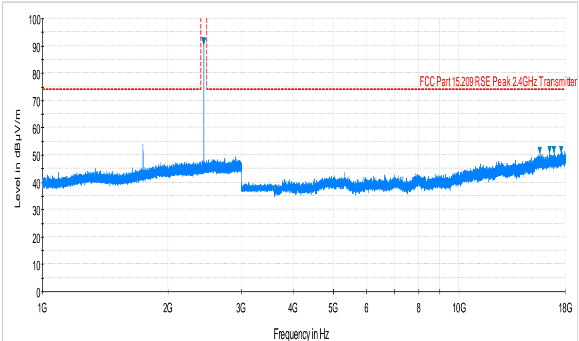
Plot 6-4. Radiated Spurious Plot above 1GHz (Bluetooth LE – Ch. 19, Ant. Pol. V)
