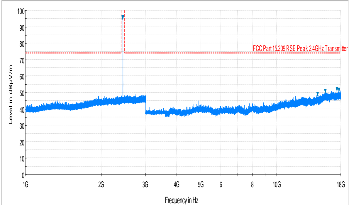
Plot 6-3. Radiated Spurious Plot above 1GHz (Bluetooth LE – Ch. 19, Ant. Pol. H)
