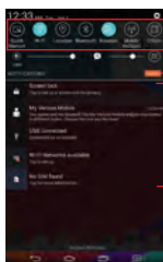
Notifications panel
