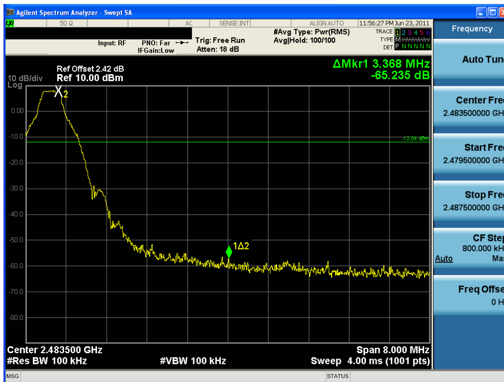
Plot 6-11. Band Edge Plot (Bluetooth, 1Mbps – Ch. 78)
