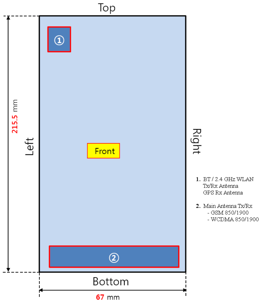
Figure 1-1 DUT Antenna Locations
