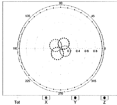
f=2200 MHz,R22,90°
