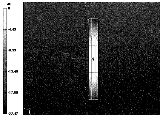
0 dB = 0.460A/m
