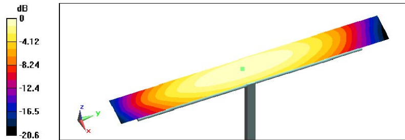
0 dB = 0.477A/m
