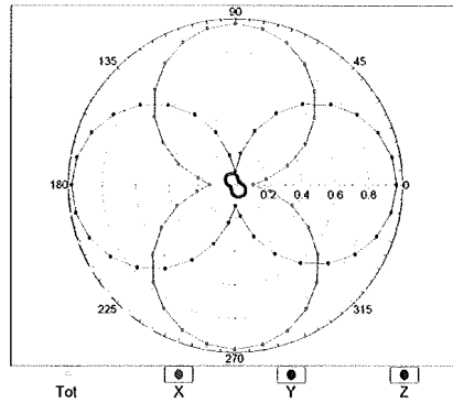
f=2200 MHz,R22,0°
