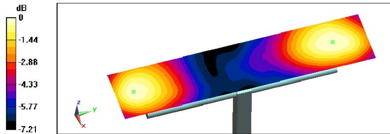
0 dB = 134.6V/m
