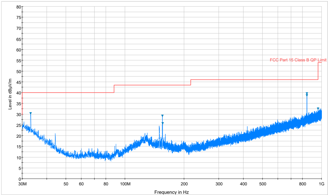
Plot 7-48. Radiated Spurious Plot below 1GHz (Pol. V)
