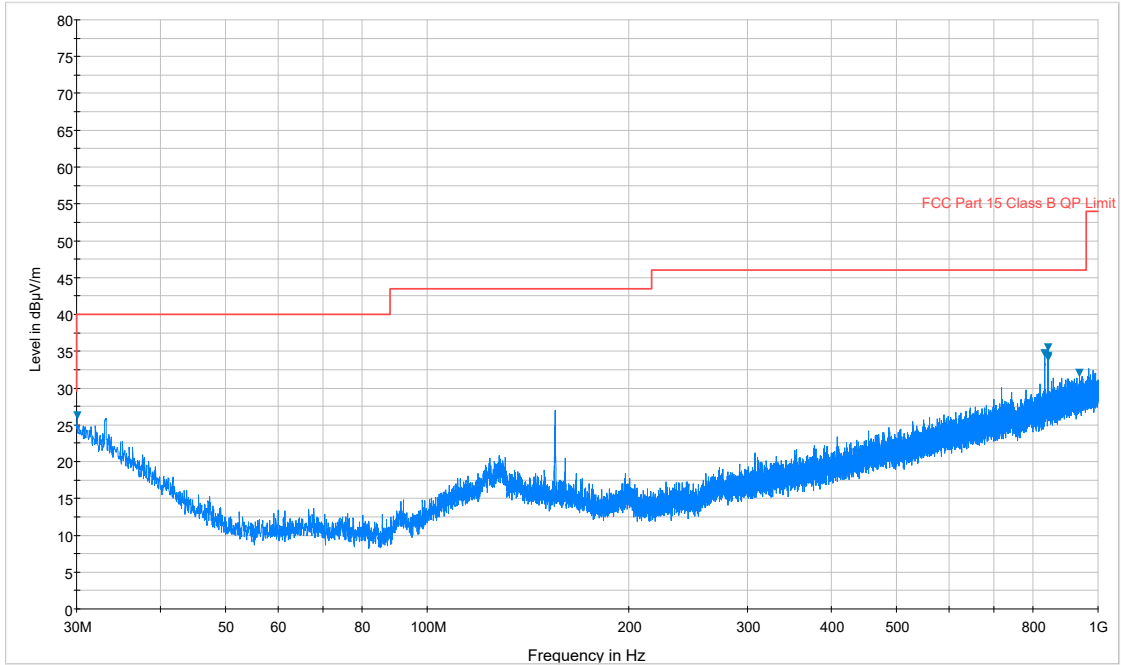
Plot 7-47. Radiated Spurious Plot below 1GHz (Pol. H)
