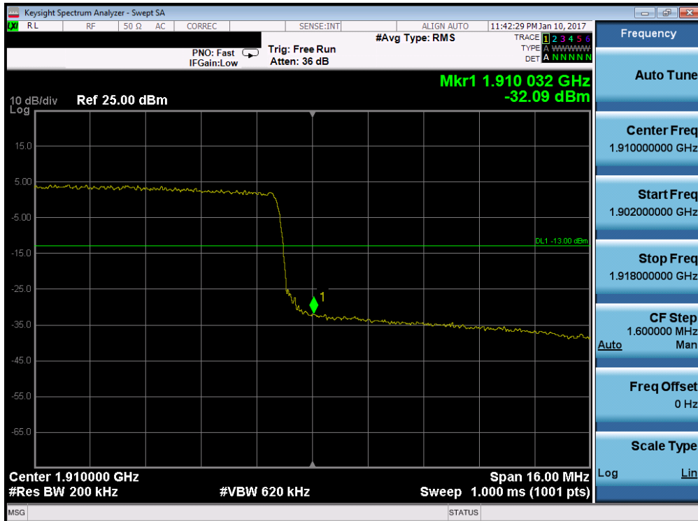
Plot 7-104. Upper Band Edge Plot (Band 2 – 20.0MHz QPSK – RB Size 100)
