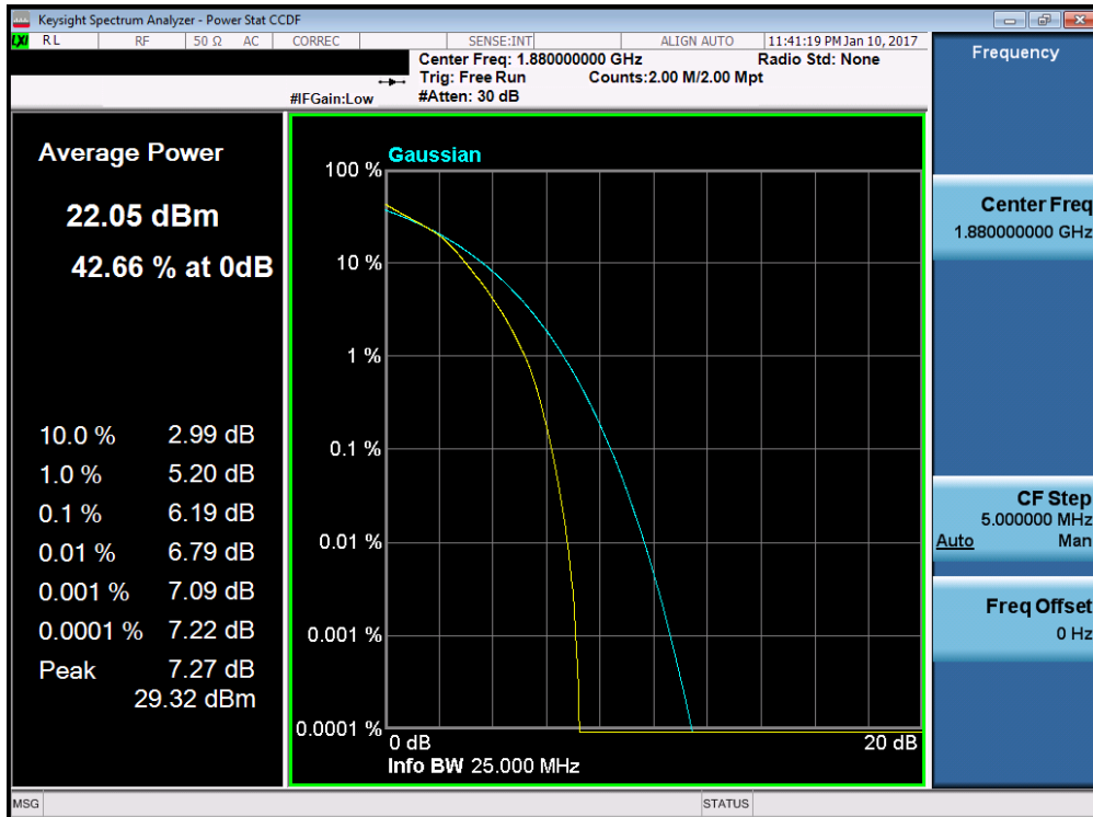
Plot 7-117. PAR Plot (Band 2 – 20.0MHz 16-QAM – RB Size 100)
