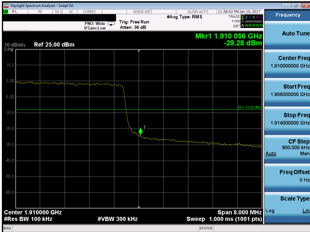
Plot 7-96. Upper Band Edge Plot (Band 2 – 10.0MHz QPSK – RB Size 50)
