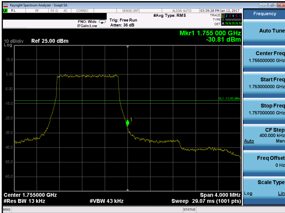
Plot 7-60. Upper Band Edge Plot (Band 4 – 1.4MHz QPSK – RB Size 6)
