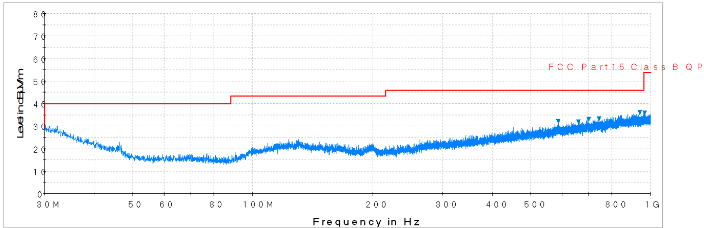
Plot 7-14. Radiated Spurious Plot below 1GHz (Pol. V)
