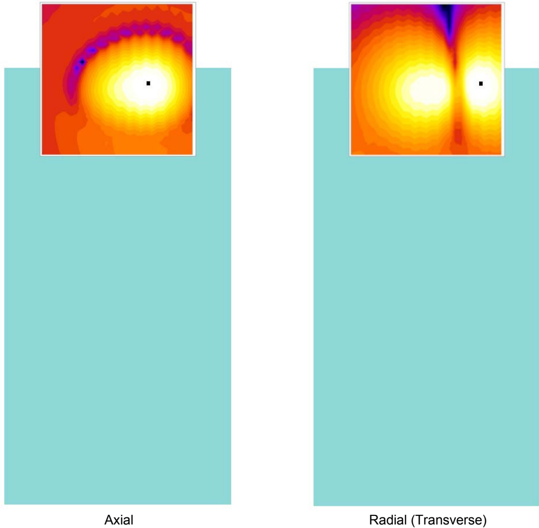
Figure 7-1 T-Coil Scan Overlay Magnetic Field Distributions
