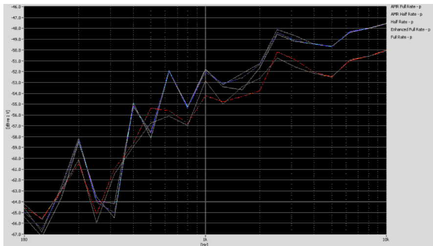
Figure 5-12 Vocoder Analysis for ABM Noise for GSM
