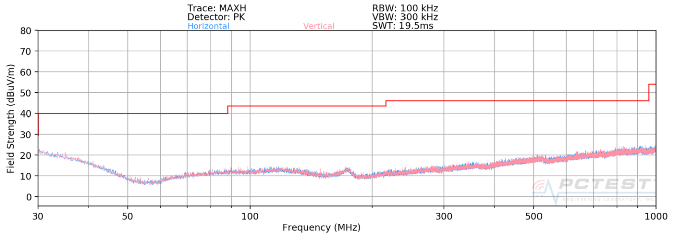
Plot 7-47. Radiated Spurious Plot below 1GHz ANT1
