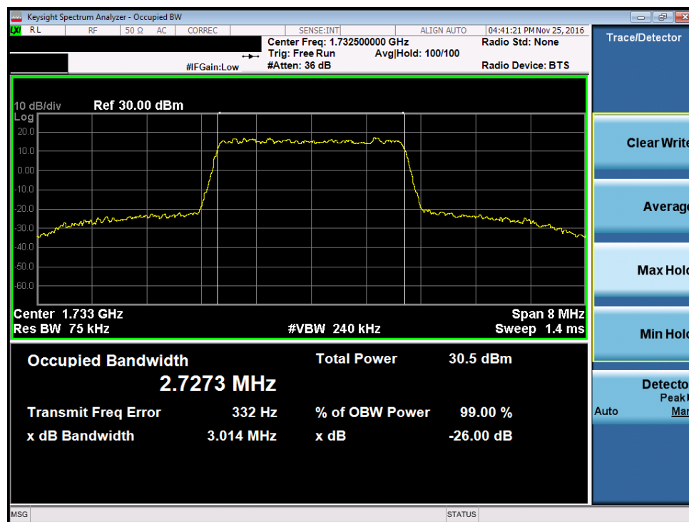
Plot 7-20. Occupied Bandwidth Plot (Band 4 – 3.0MHz QPSK – RB Size 15)
