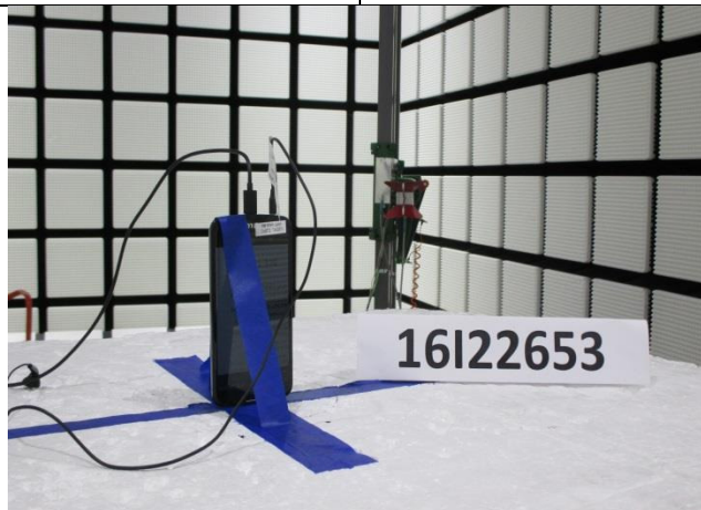
Z-AXIS POSITION
