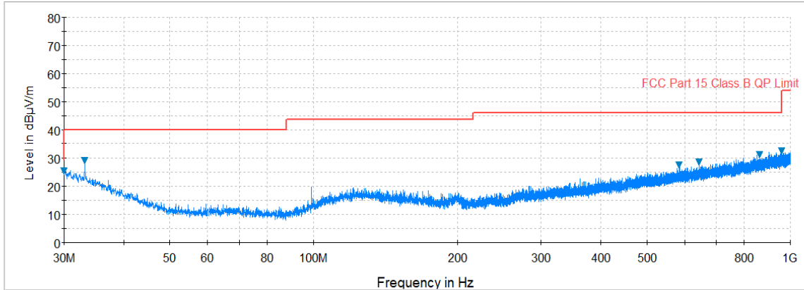
Plot 7-15. Radiated Spurious Plot below 1GHz (Pol. H)
