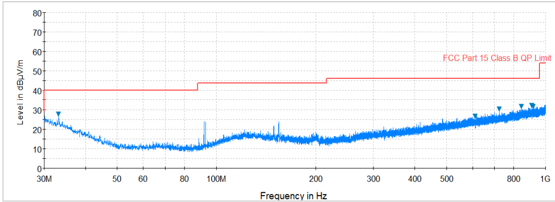
Plot 7-16. Radiated Spurious Plot below 1GHz (Pol. V)
