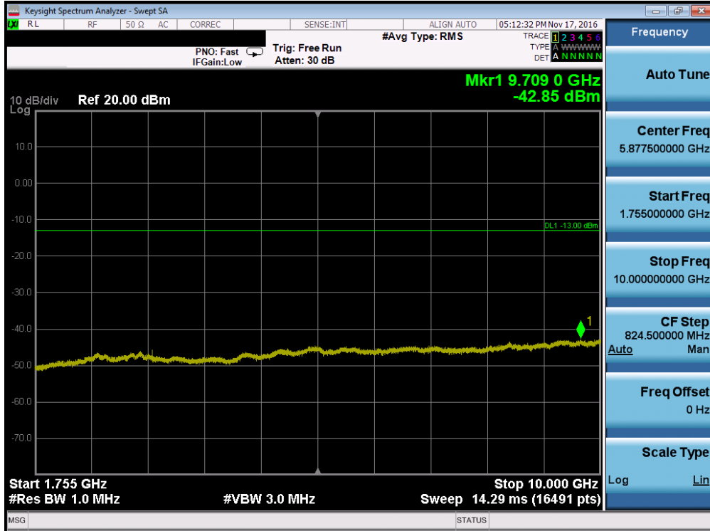
Plot 7-63. Conducted Spurious Plot (Band 4 – 3.0MHz QPSK – RB Size 1, RB Offset 0 – Mid Channel)
