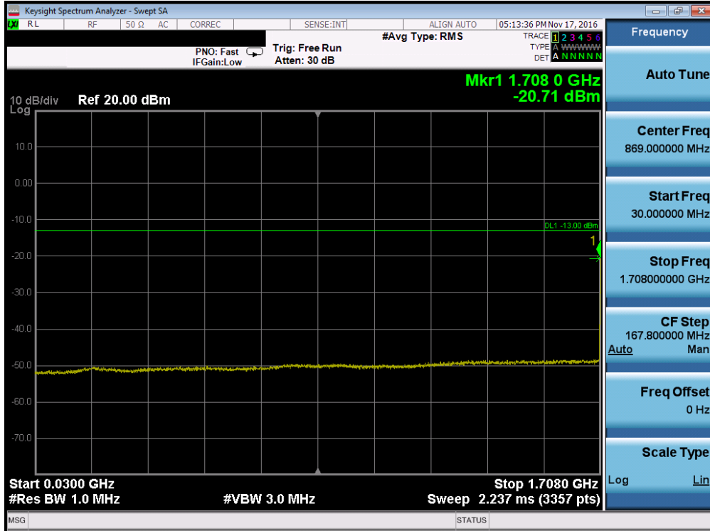
Plot 7-59. Conducted Spurious Plot (Band 4 – 3.0MHz QPSK – RB Size 1, RB Offset 0 – Low Channel)
