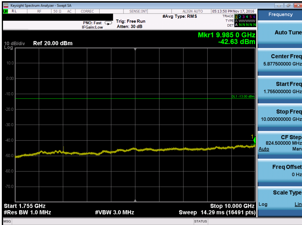
Plot 7-60. Conducted Spurious Plot (Band 4 – 3.0MHz QPSK – RB Size 1, RB Offset 0 – Low Channel)
