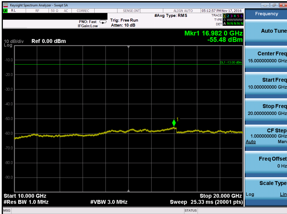
Plot 7-64. Conducted Spurious Plot (Band 4 – 3.0MHz QPSK – RB Size 1, RB Offset 0 – Mid Channel)
