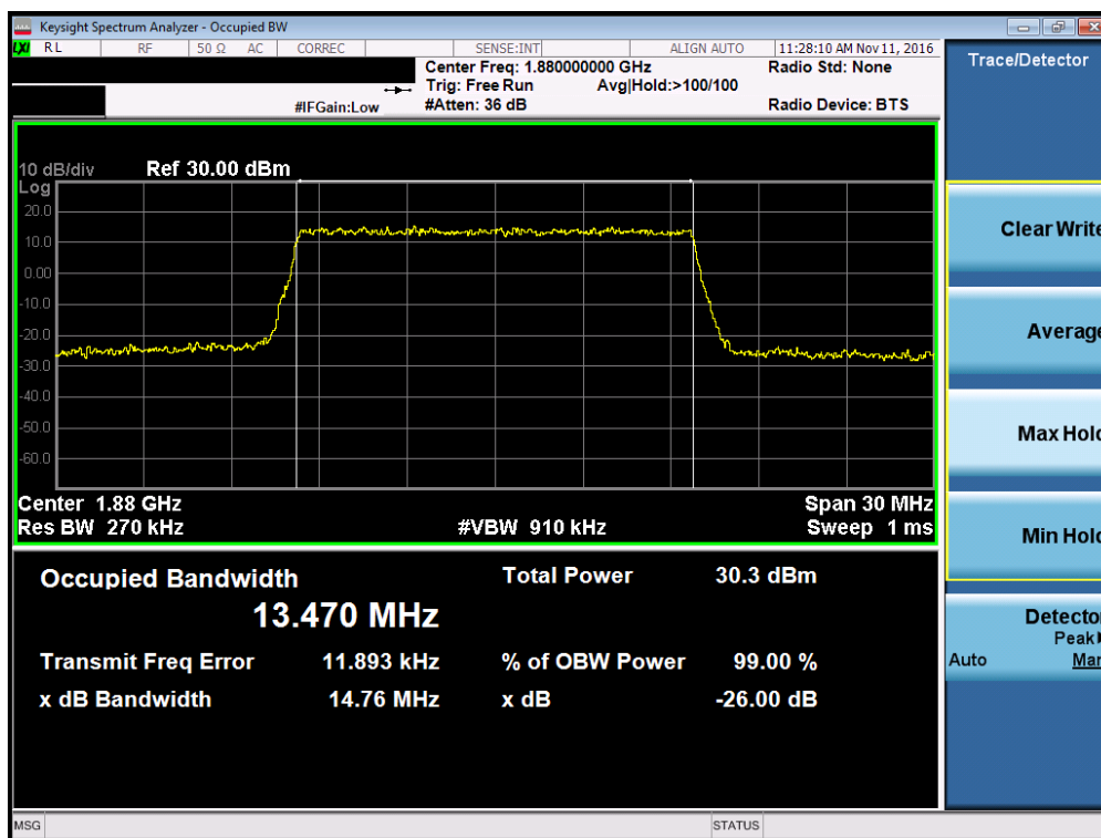
Plot 7-38. Occupied Bandwidth Plot (Band 2 – 15.0MHz 16-QAM – RB Size 75)
