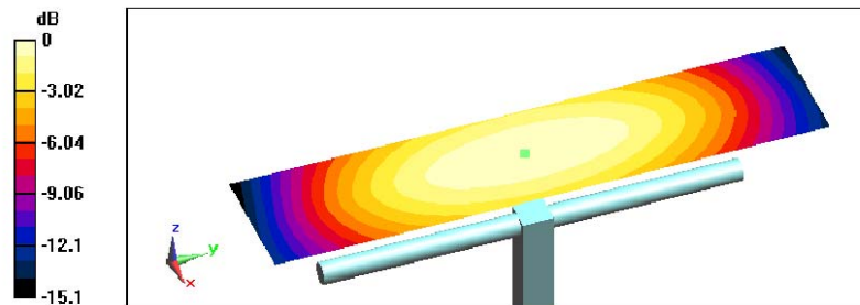
0 dB = 0.445A/m
