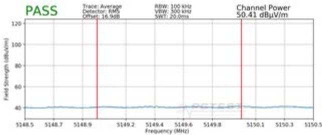
Plot 7-35. Radiated Lower Band Edge Plot (Average – UNII Band 1)
