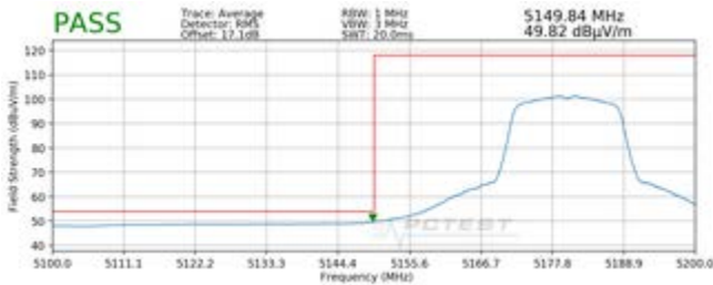
Plot 7-7. Radiated Lower Band Edge Plot (Average – UNII Band 1)
