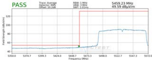
Plot 7-39. Radiated Lower Band Edge Plot (Average – UNII Band 2C)
