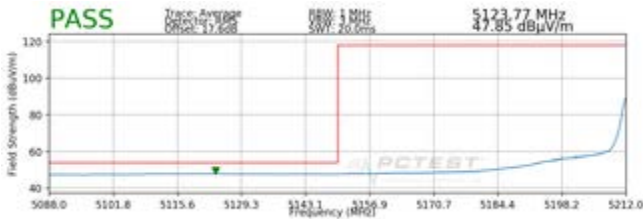
Plot 7-23. Radiated Lower Band Edge Plot (Average – UNII Band 1)
