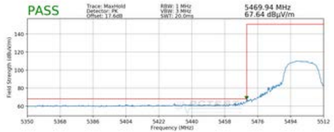
Plot 7-16. Radiated Lower Band Edge Plot (Peak – UNII Band 2C)
