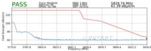
Plot 7-33. Radiated Upper Band Edge Plot (Peak – UNII Band 3)
