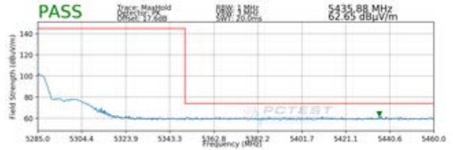
Plot 7-26. Radiated Upper Band Edge Plot (Peak – UNII Band 2A)
