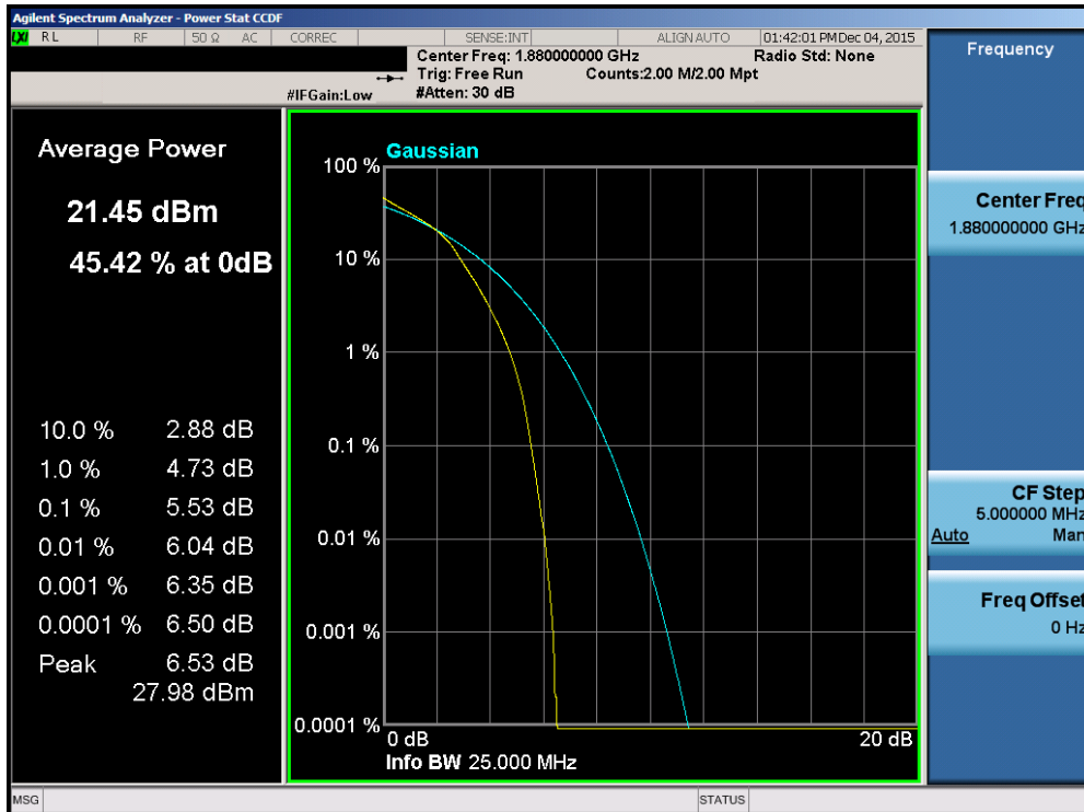
Plot 7-124. PAR Plot (Band 2 – 20.0MHz 16-QAM – RB Size 100)
