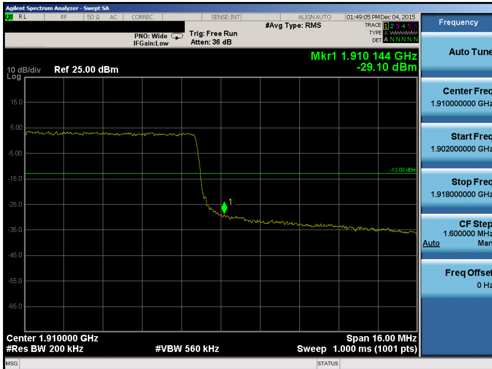
Plot 7-111. Upper Band Edge Plot (Band 2 – 20.0MHz QPSK – RB Size 100)
