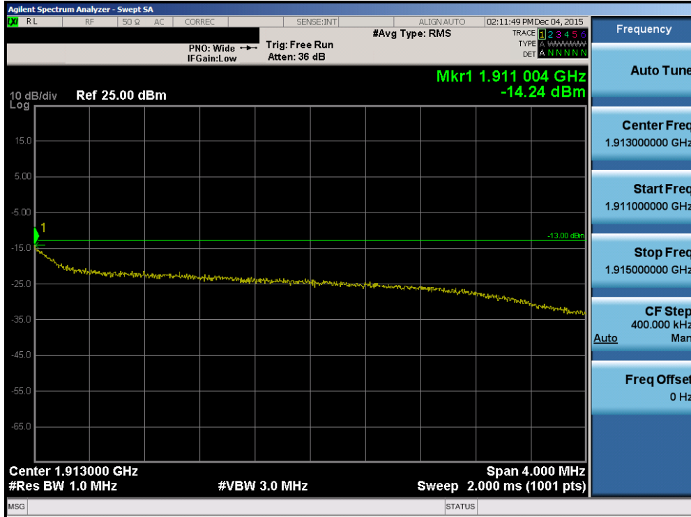
Plot 7-100. Upper Extended Band Edge Plot (Band 2 – 5.0MHz QPSK – RB Size 25)
