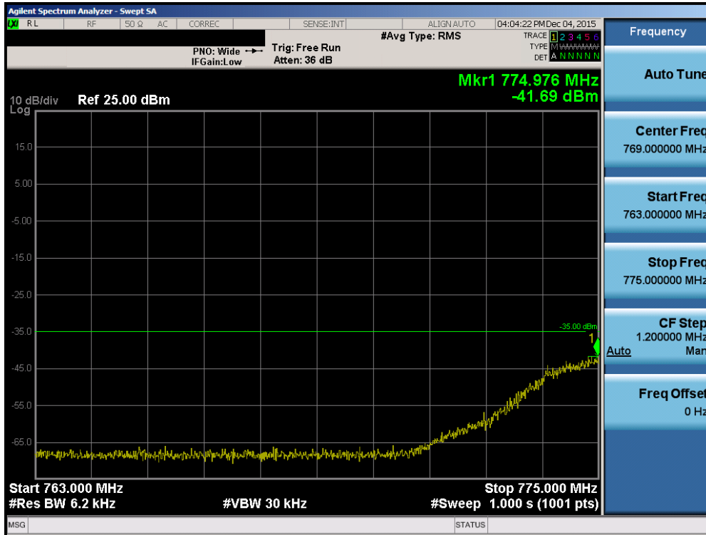
Plot 7-58. Lower Emission Mask Edge Plot (Band 13 – 5.0MHz QPSK – RB Size 25)
