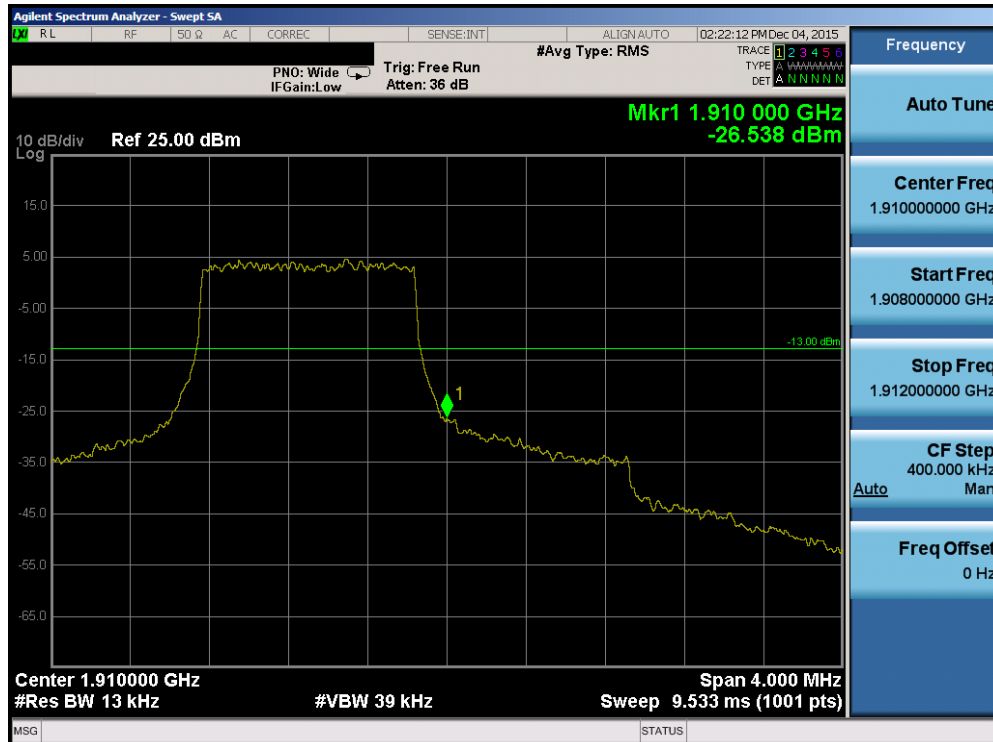
Plot 7-91. Upper Band Edge Plot (Band 2 – 1.4MHz QPSK – RB Size 6)
