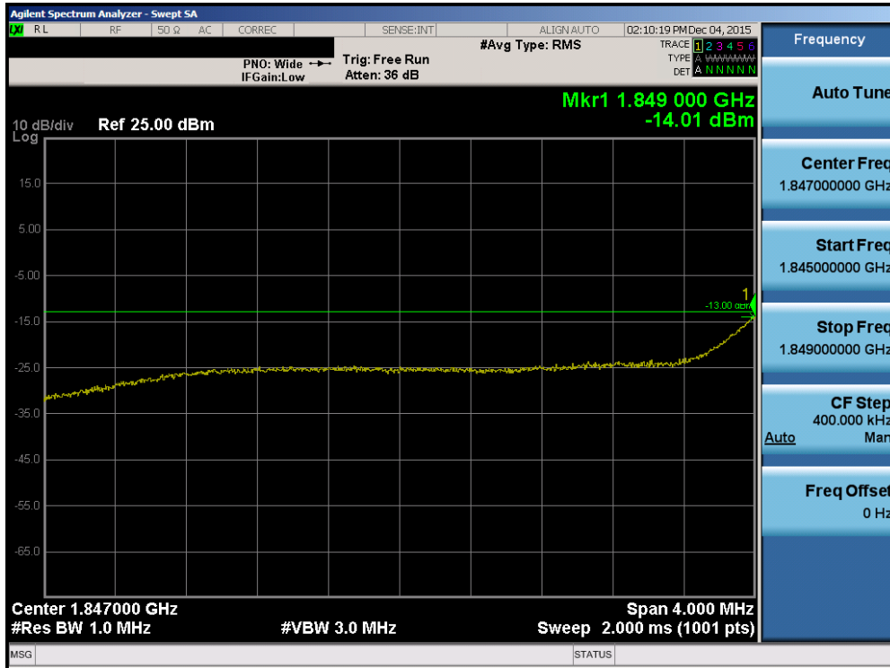
Plot 7-98. Lower Extended Band Edge Plot (Band 2 – 5.0MHz QPSK – RB Size 25)
