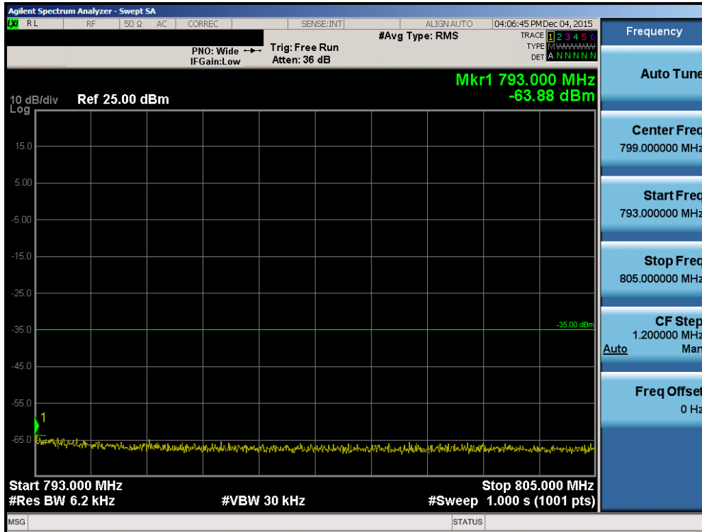
Plot 7-60. Upper Emission Mask Edge Plot (Band 13 – 5.0MHz QPSK – RB Size 25)
