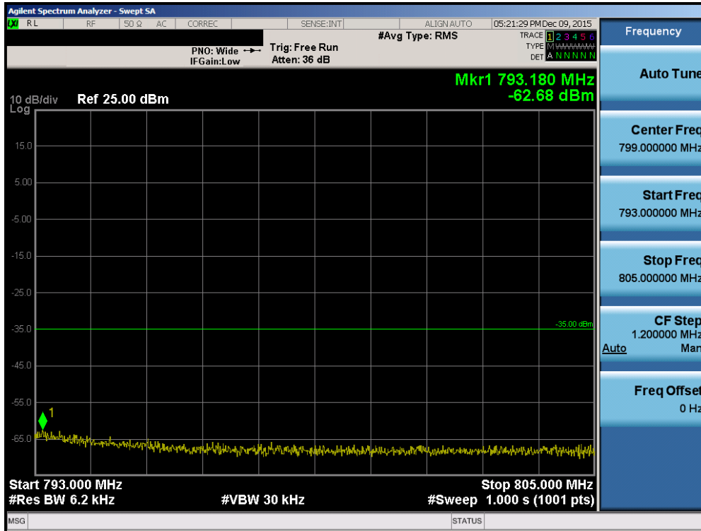
Plot 7-64. Upper Emission Mask Edge Plot (Band 13 – 10.0MHz QPSK – RB Size 50)
