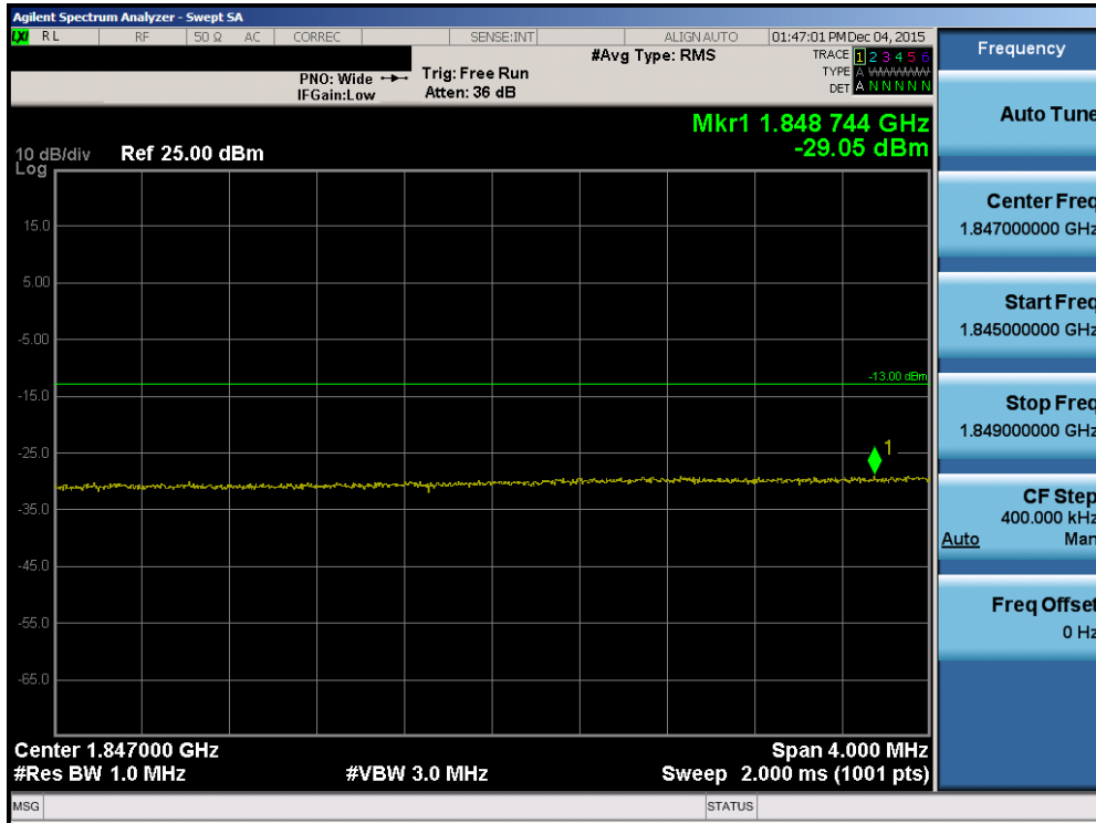
Plot 7-110. Lower Extended Band Edge Plot (Band 2 – 20.0MHz QPSK – RB Size 100)
