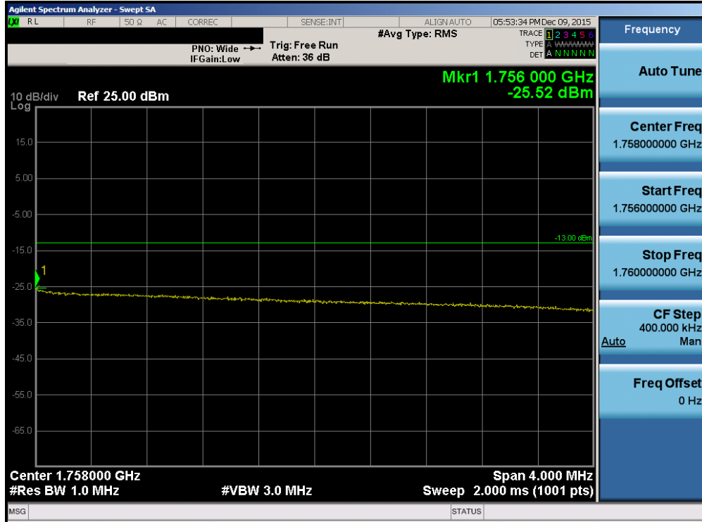
Plot 7-80. Upper Extended Band Edge Plot (Band 4 – 10.0MHz QPSK – RB Size 50)
