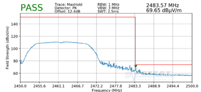
Plot 7-12. Radiated Restricted Upper Band Edge Measurement (Peak)
