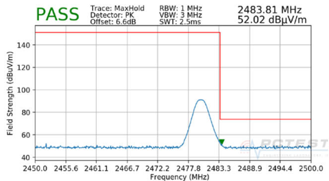
Plot 7-2. Radiated Restricted Upper Band Edge Measurement (Peak)
