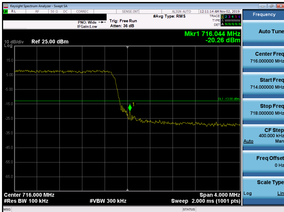
Plot 7-173. Upper Band Edge Plot (Band 12 - 5.0MHz QPSK - Full RB Configuration)
