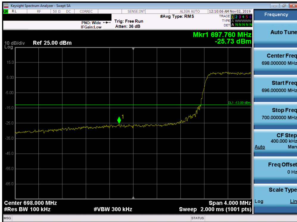
Plot 7-172. Lower Band Edge Plot (Band 12 - 5.0MHz QPSK - Full RB Configuration)
